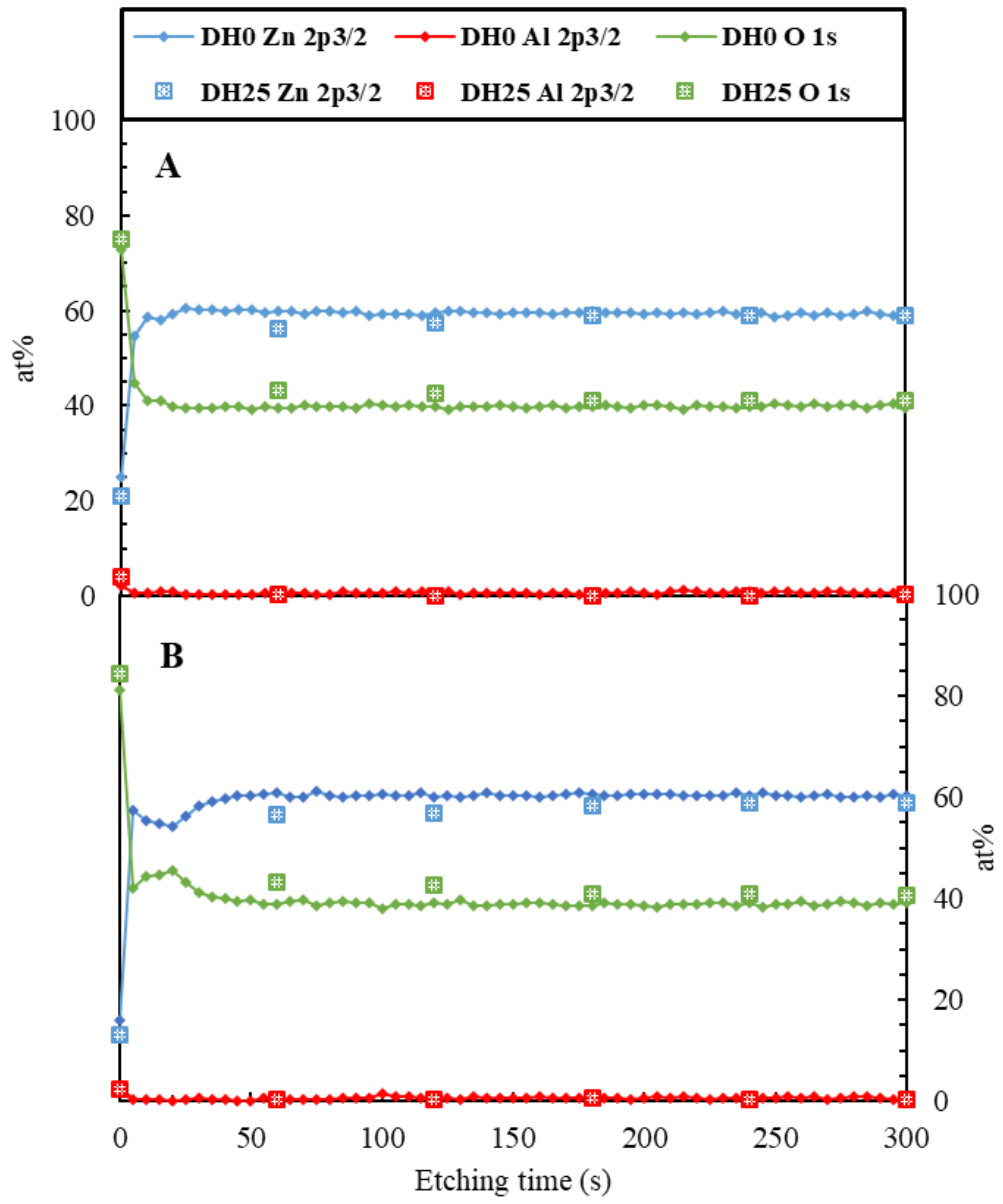
Fig. 6-6. Quantification of the Zn 2p3/2, Al 2p3/2, and O elements via XPS for the AZO/glass (A) and AZO/PI-tape/PC (B) samples before (line with diamonds) and after (squares) the damp-heat (DH) test.
