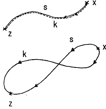
図 1: A pair of identical orbits (upper) and a periodic orbits of period 2t as a result of constructive interference of two different classical trajectories s and k belonging to the same energy hyperspace (lower).
