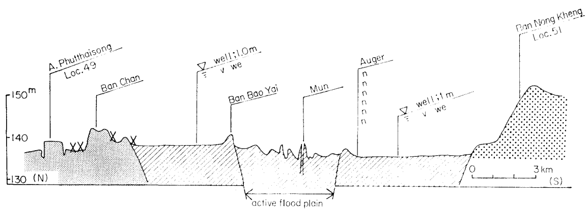
Fig. 33 Cross section 49-51
