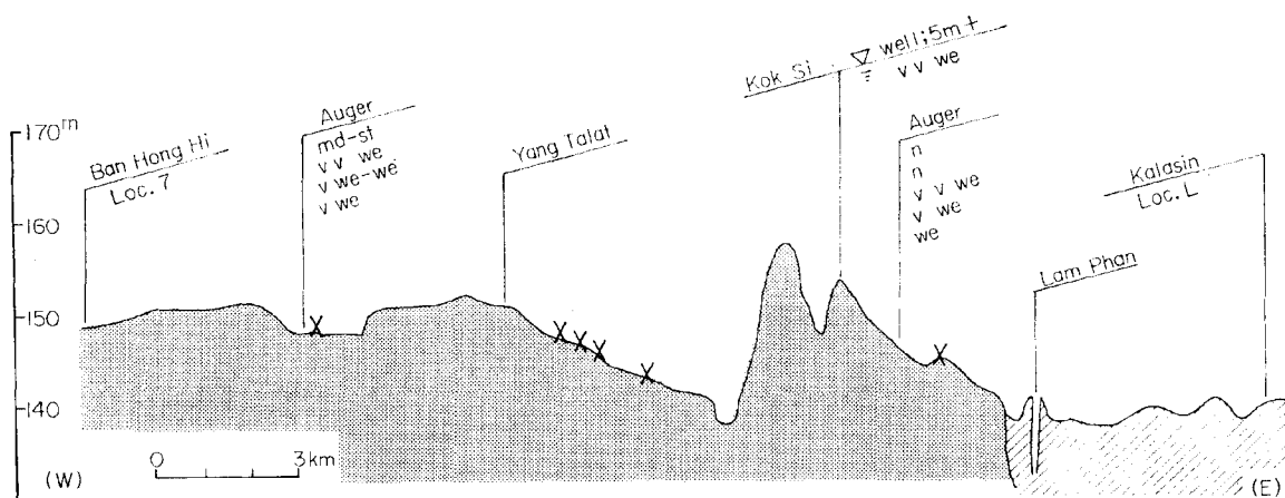
Fig. 7 Cross section ⑦-⑩
