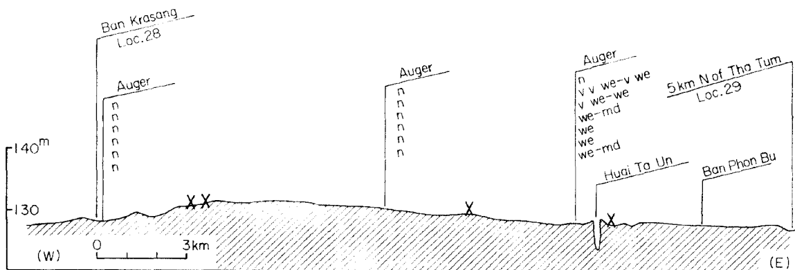
Fig. 20 Cross section 28-29
