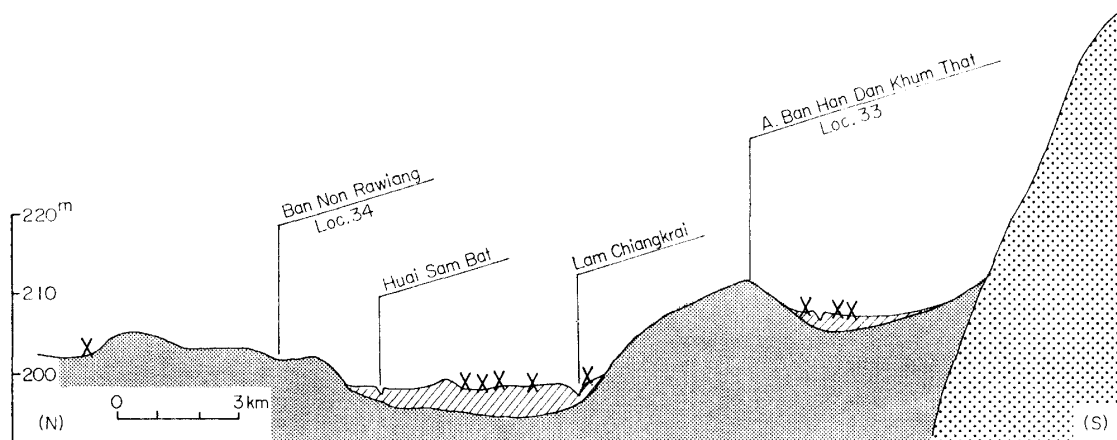
Fig. 23 Cross section 33-34
