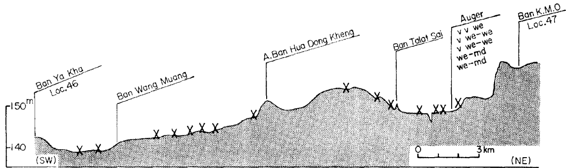
Fig. 30 Cross section 46-47
