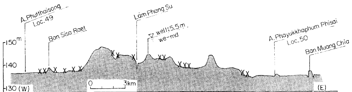
Fig. 32 Cross section 49-50
