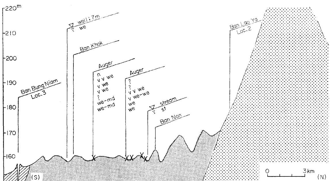
Fig. 3 Cross section ②-③
