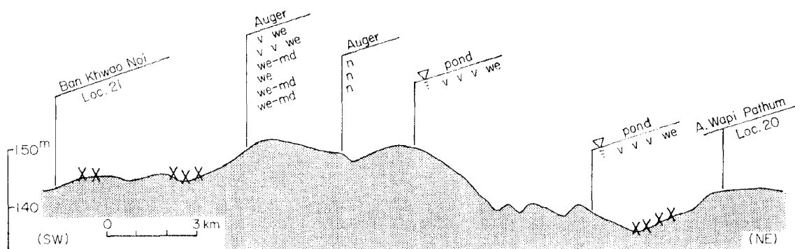
Fig. 15 Cross section (20-21)
