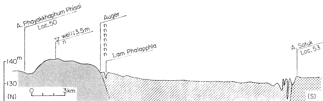
Fig. 35 Cross section 50-53
