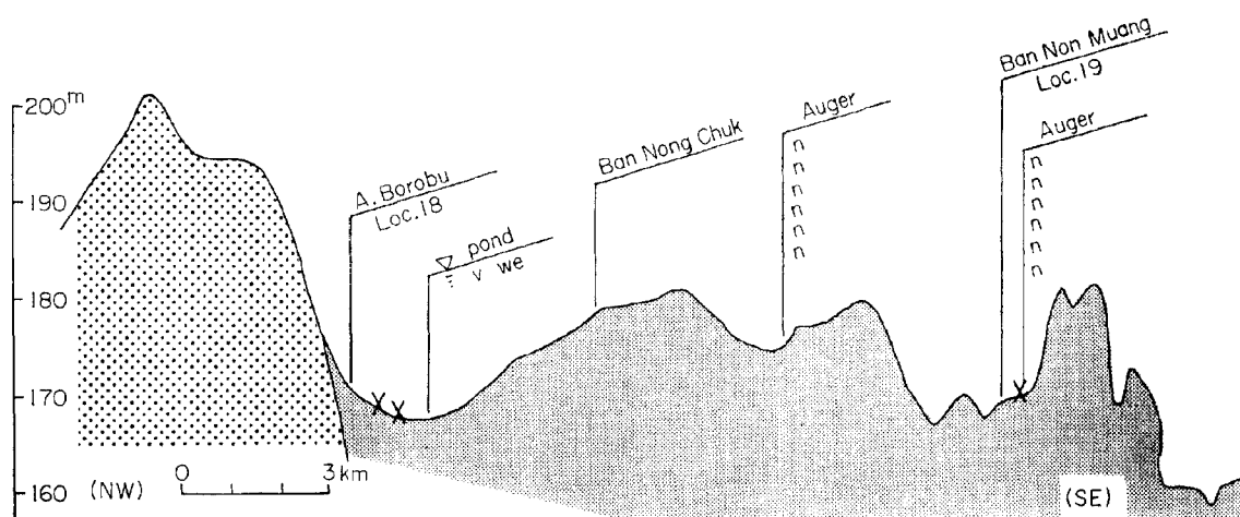
Fig. 14 Cross section (18-19)
