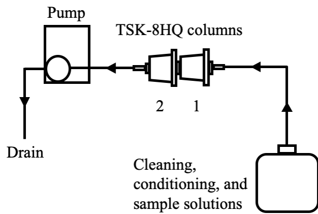
Fig. 1 Diagram of the preconcentration system with two serial-coupled columns of TSK-8HQ.
