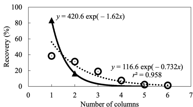
Fig. 4. Recovery (%) of W from seawater for each column via column extraction. Open circles: NOBIAS Chelate-PA1. Closed triangles: TSK-8HQ. The solid and dotted curves are calculated by curve fitting with exponential functions.
