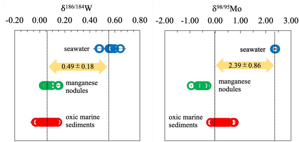
Fig. 8. \delta^{186/184}\text{W} and \delta^{98/95}\text{Mo} in seawater (this study) compared with those in manganese nodules (Abraham et al., 2015; Barling et al., 2001; Goto et al., 2015; Irisawa and Hirata, 2006; Kurzweil et al., 2019; Tsujisaka et al., 2019; Zhao et al., 2016) and oxic sediments from the Mediterranean Sea (Kurzweil et al., 2019) and the Japan Sea (Tsujisaka et al., in press). The error bars represent \pm 2 times the standard error of individual measurements. The dotted lines represent the averages for seawater and solid phases.
