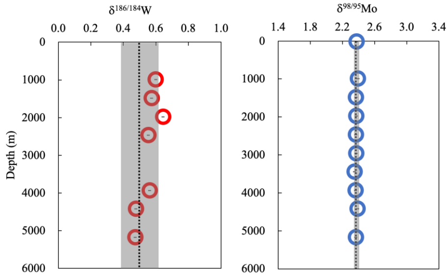
Fig. 6. Vertical profiles of isotopic ratios of W and Mo at station CL-2 (47°00'N, 160°00'E; bottom depth of 5195 m) in the western North Pacific Ocean. The error bars represent \pm 2 times the standard error of individual measurements. The dotted lines represent the averages throughout the water column, and the shaded areas represent \pm 2 sd.
