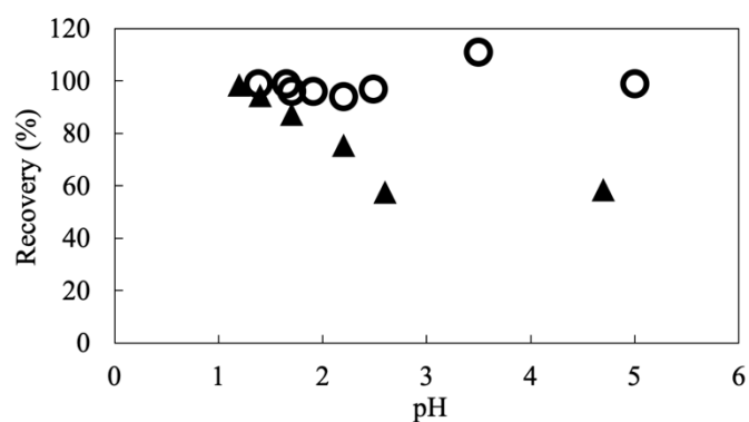
Fig. 2. pH dependence of the recovery (%) of W by column extraction using a single column. Open circles: NOBIAS Chelate-PA1. Closed triangles: TSK-8HQ. The sample solutions were Milli-Q water for NOBIAS Chelated-PA-1 experiments but seawater for TSK-8HQ experiments.
