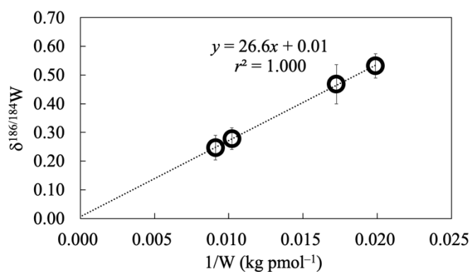
Fig. 5. \delta^{186/184}W vs the inverse W concentration for mixed seawater samples with and without spiking of the W isotope standard. The dotted line represents the linear regression. The error bars represent \pm 2 times the standard error of individual measurements.
