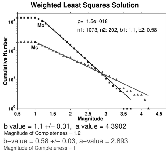
Fig. 7 Frequency-magnitude distribution in the north (N region in fig. 6) and south (S region in fig. 6) of Hida Mountains. The small p indicates here the probability that the two distributions come from the same mother population, by using Utsu's statistical test (1992). Squares – south region; triangles – north region.
