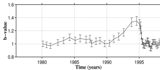
Fig. 3 b -value change in the Tanba region. The graph shows that before the large event the b -value in the Tanba region had a very clear increase. The b -value after the occurrence of 1995 Kobe earthquake returns to an average of 1.0.
