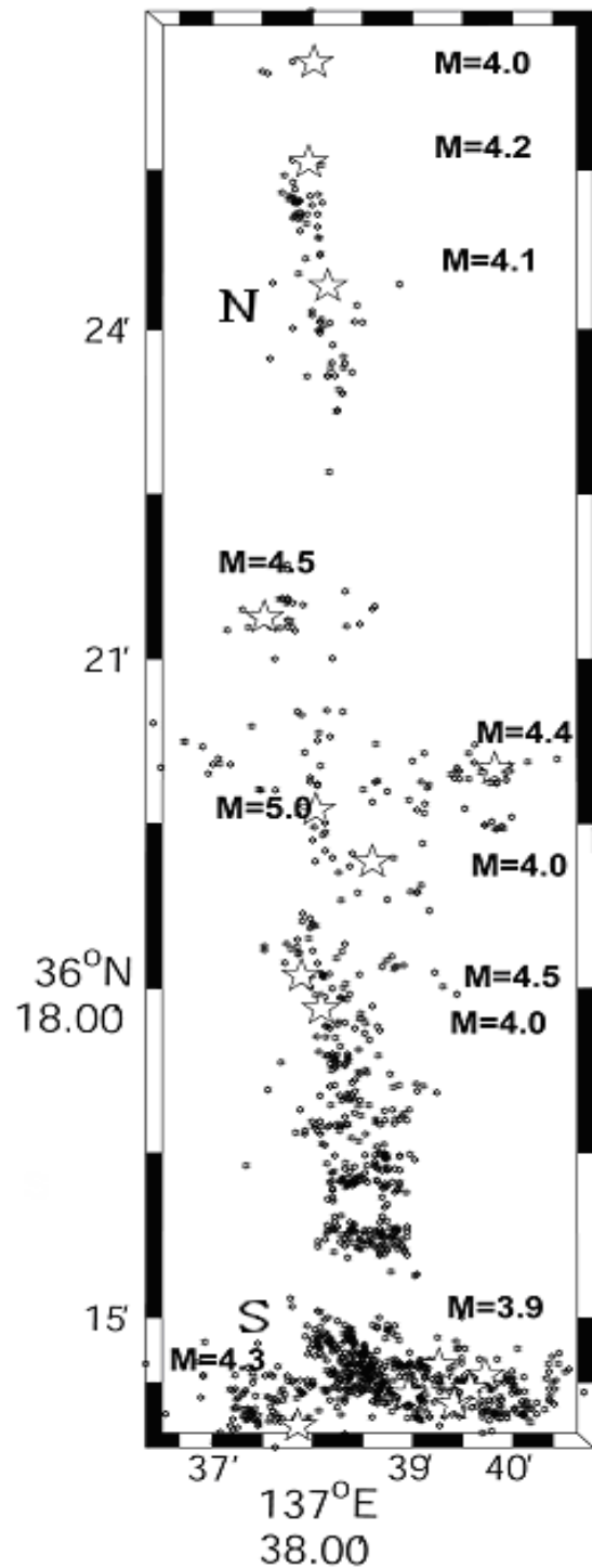
Fig.6 Relocated seismicity for Hida Mt. earthquake swarms ( M \geq 1.7 ). N and S refer to the north south regions that are compared for their frequency magnitude distribution in Fig.7. Star show events with M \geq 4.0 .
