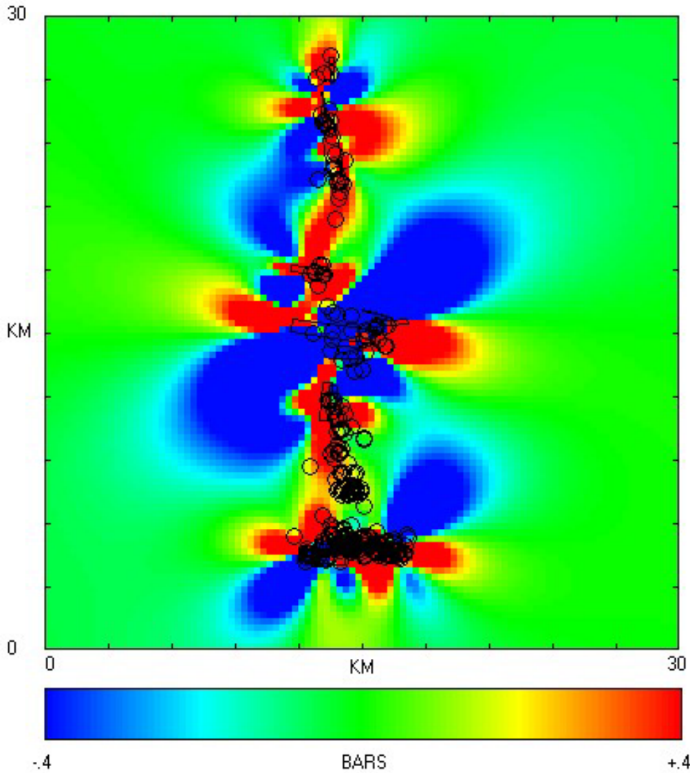
Fig. 10 Coulomb failure stress change on optimum oriented failure planes, as a result of the largest 18 events with M \geq 4.0 occurred during a time period of about two months since the beginning of the Hida Mt. swarm. The red and blue colors indicate an increase or, respectively, a decrease in Coulomb stress. The regional stress has a WNW-ESE direction. Double-difference relocated events ( M \geq 1.7 ) are superposed on the stress map.
