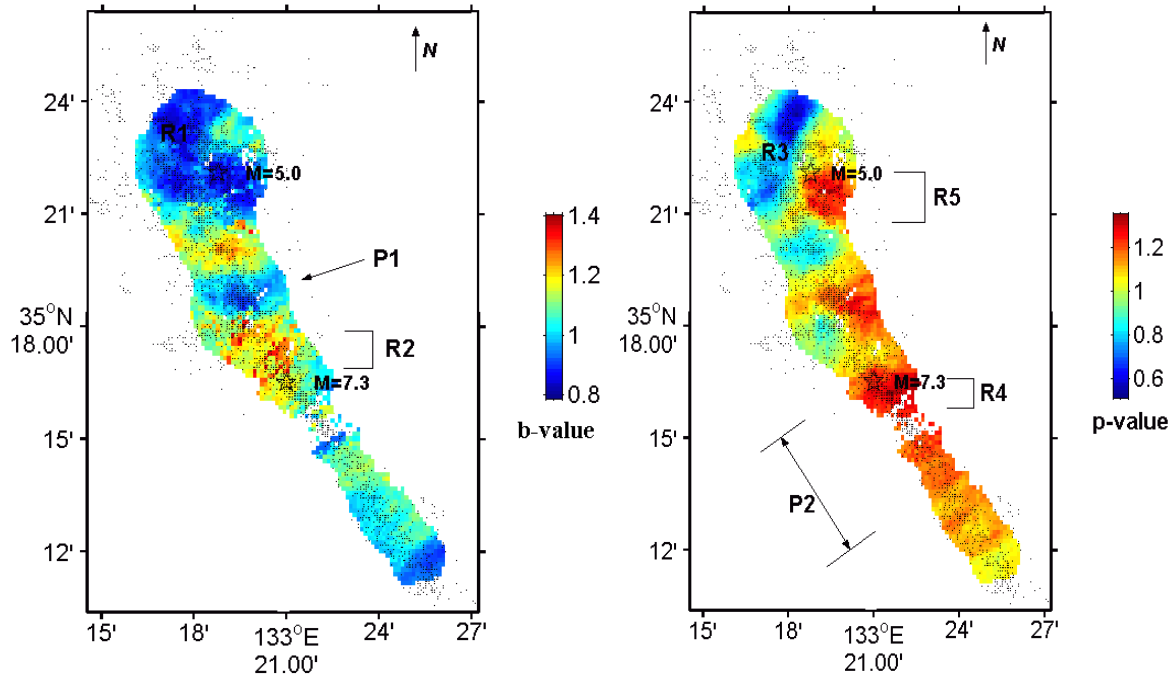
Fig. 4 a) b -value map for the aftershocks of 2000 Western Tottori earthquake. One can notice that the b -value is larger ( \geq 1.0 ) for a large area extending about 10 km on each side of the main shock. There is an exception, the patch P1, where b -value is smaller. The both ends of the aftershock region (NW and SE) are characterized by a small b -value. In order to demonstrate the difference of b -value clearly we have chosen two regions (R1 and R2) and compute their frequency-magnitude distribution. The result is presented in the next figure.
