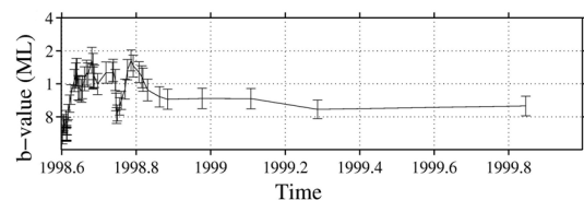
Fig. 8 Variation of b -value with time, for the south region (S in figure 6) of Hida Mt., when using all the earthquakes with M \geq 1.2 located by DPRI, Kyoto University. There are 200 events in a moving window.
