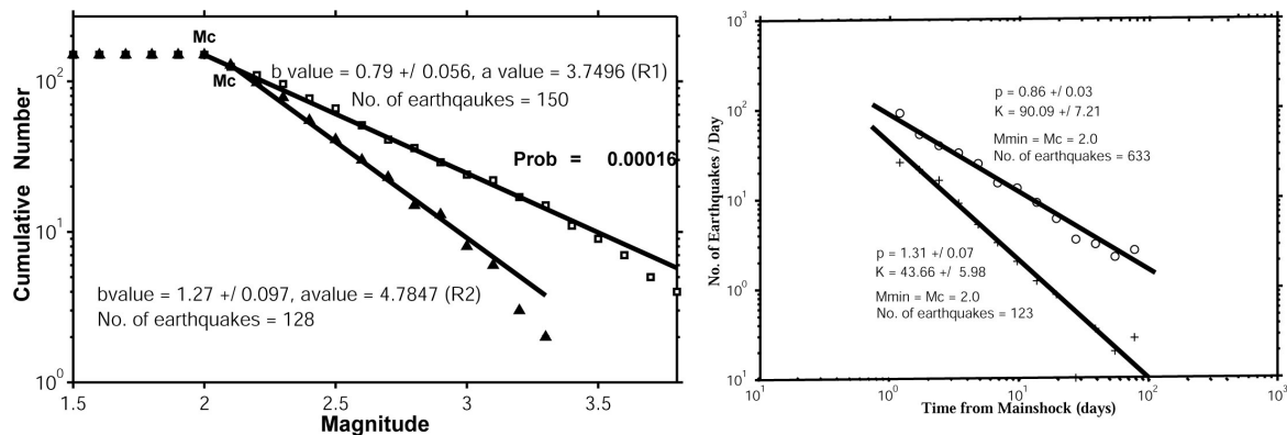
Fig. 5 a) Comparison of the frequency-magnitude distribution for the Region R1 and R2 in Fig.4a. The probability, Prob, that the two distributions come from the same population is very small, as indicated by Utsu's statistical test (Utsu, 1992). b) Comparison of p -value for the regions R3 and R4 in Fig.4b. The decay of aftershocks in the two regions is significantly different. We have obtained a similar result, when comparing the R3 and R5 regions.
