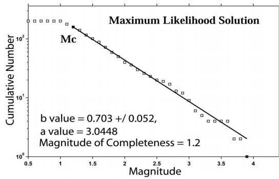
Fig. 9 b-value obtained by the maximum likelihood method for the very beginning of the swarm sequence in the southern cluster ( S in figure 6).
