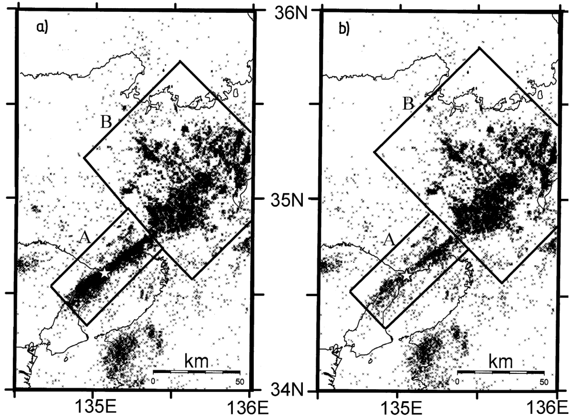
Fig. 1 Clustered (a) and undeclustered (b) seismicity (1976-1998, M \geq 1.5 ) in a large region surrounding the epicenter of the 1995 Kobe earthquake. A – epicentral region, B – Tanba region. Star – Kobe earthquake.
