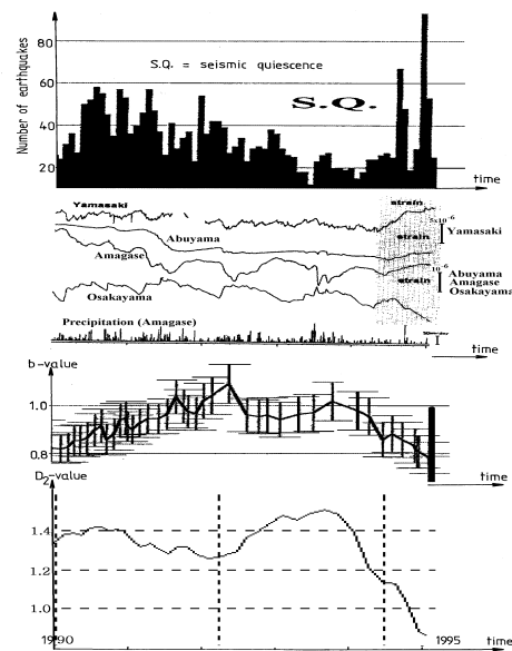
Fig. 2 From up do down: seismicity rate changes, with a clear seismic quiescence pattern (SQ) followed by an increase in seismic activity (ISA), several months before the Kobe earthquake; b) strain variation and precipitation (DPRI); c) b -value changes: increase and decrease before Kobe earthquake; d) changes in the fractal dimension ( D_2 ) of the epicentral distribution of earthquakes: large decrease associated probably with ISA, correlates well with the decrease in b -value.
