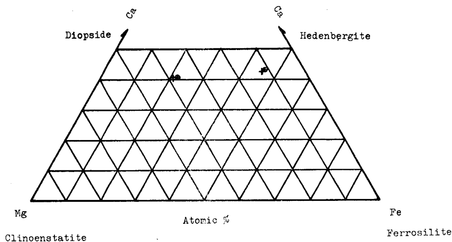
Fig. 5 + ; Pyroxene in Diorite Porphyrite ● ; Pyroxene in Doleritic Propylite
