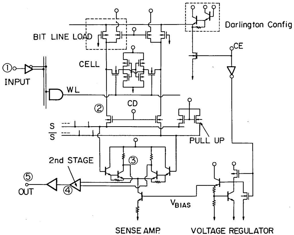
Fig. 3.10 Cell and its peripheral circuitry.
