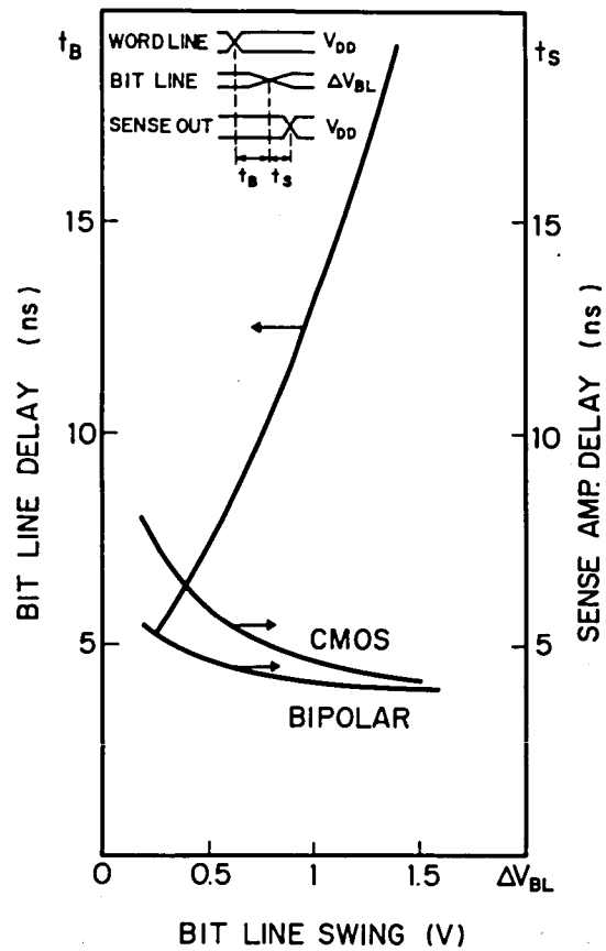
Fig. 3.5 Simulation results of the delay time in bitline and the sense amplifier as a function of bitline swing.
