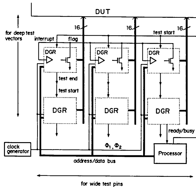
Fig. 5.1 A simple tester built using DGR chips.
