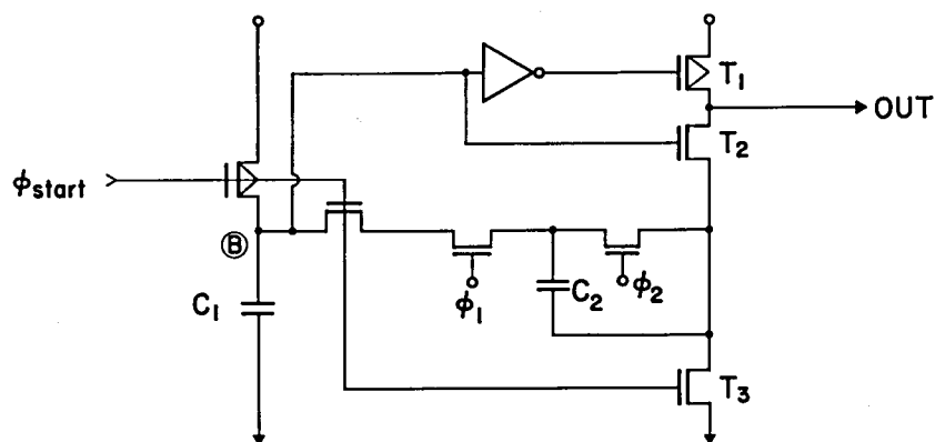
Fig. 4.23 Successive data loading control circuits ( \Phi_{\text{START}} generator). A period of 100us is counted by the switched capacitor.
