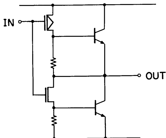
Fig. 3.19 Bi-CMOS buffer circuit.
