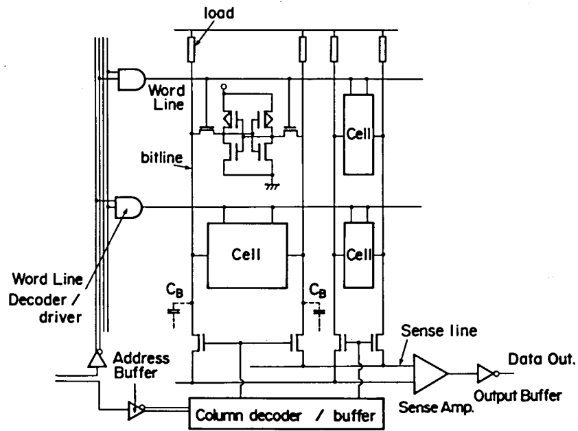
Fig. 3.4 Schematic diagram of CMOS RAM.
