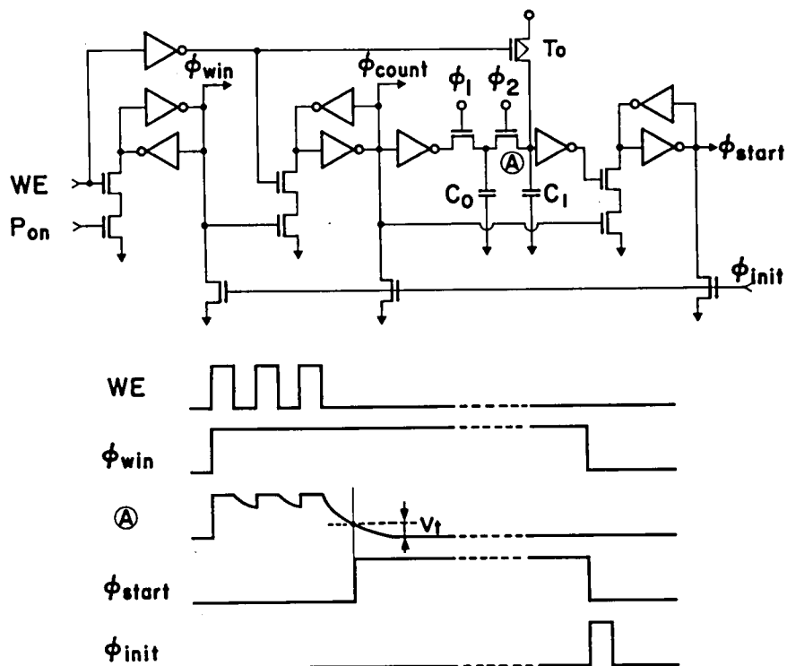
Fig. 4.23 Successive data loading control circuits ( \Phi_{\text{START}} generator). A period of 100us is counted by the switched capacitor.
