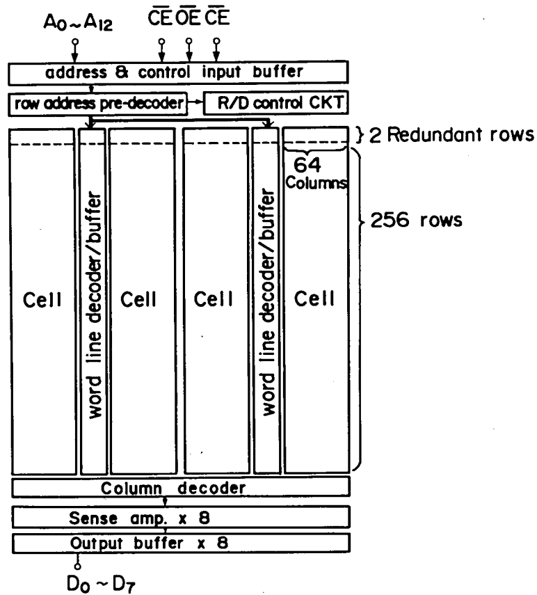
Fig. 3.9 Memory block diagram.
