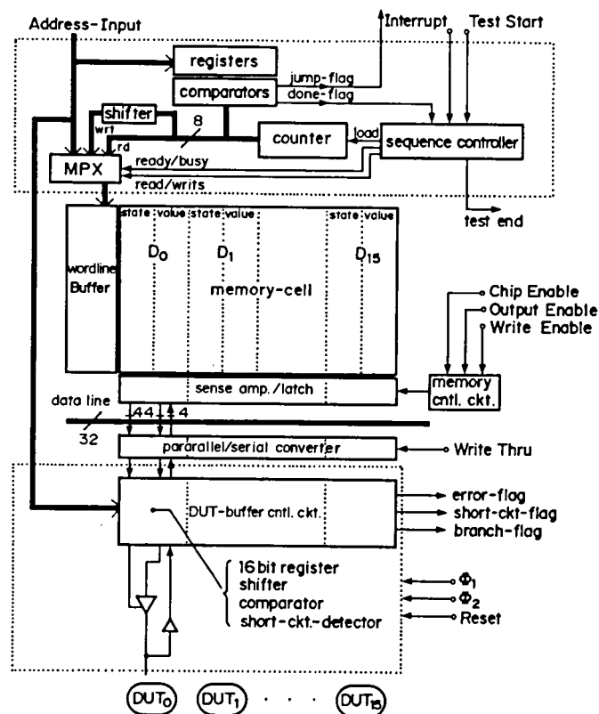
Fig. 5.2 A block diagram of the DGR.
