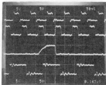
Fig. 5.16 DGR output waveforms of several working modes. \Phi_1 and \Phi_2 are the inputs. It is shown that DGR is working over 10MHz vector rate in every mode.
