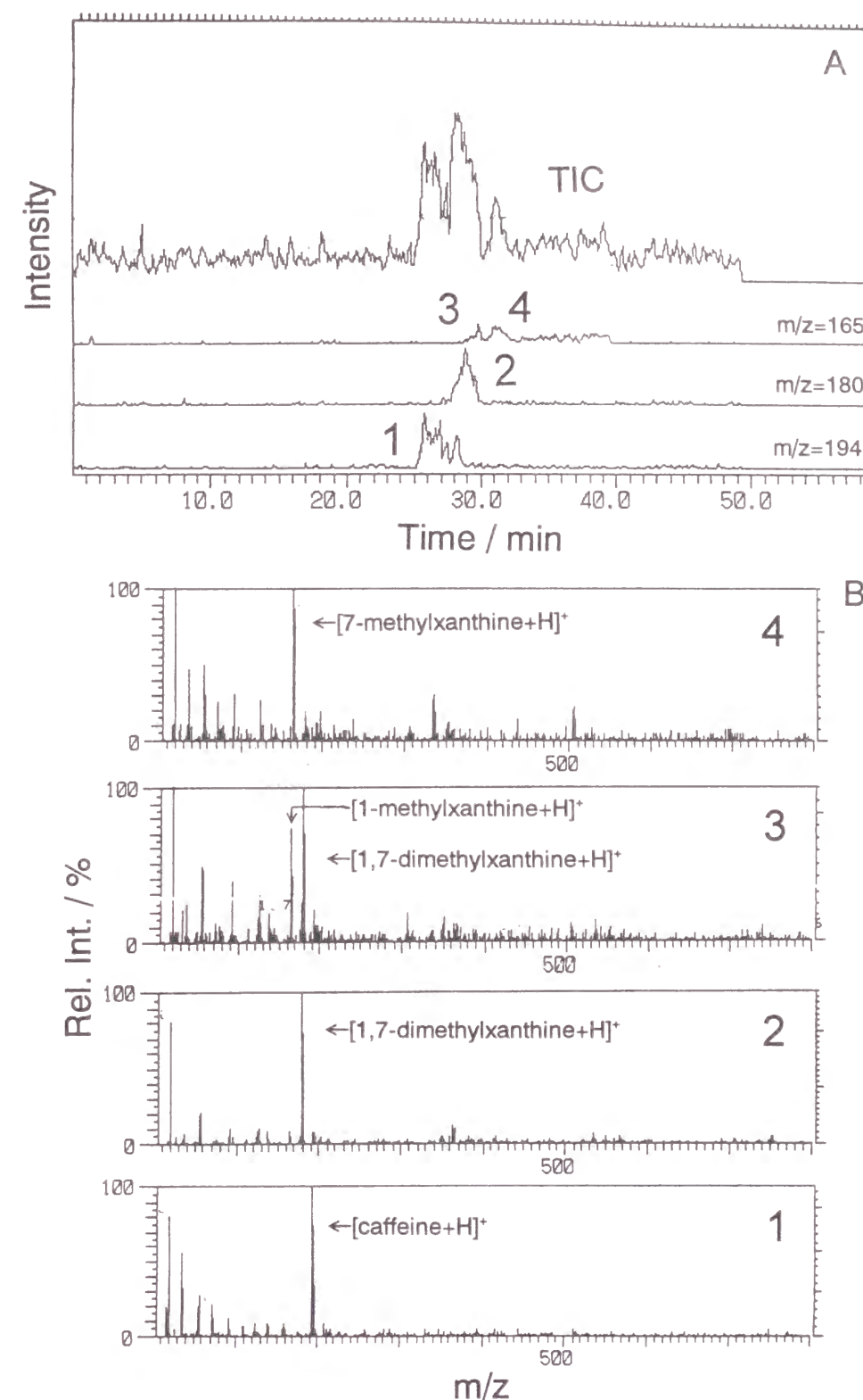
Fig. 5.9 MEKC-ESI-MS of caffeine and its metabolites using BBMA (A) and mass spectra of the peaks (B). Solute as in Fig.5.8. Conditions: capillary, 50 \mu\text{m} i.d., 100 cm fused-silica; separation solution, 2% BBMA introduced at 0.1 atm for 120 s in 20 mM ammonium formate (pH 7); applied voltage, 20 kV. Other conditions as in Fig.5.1.
