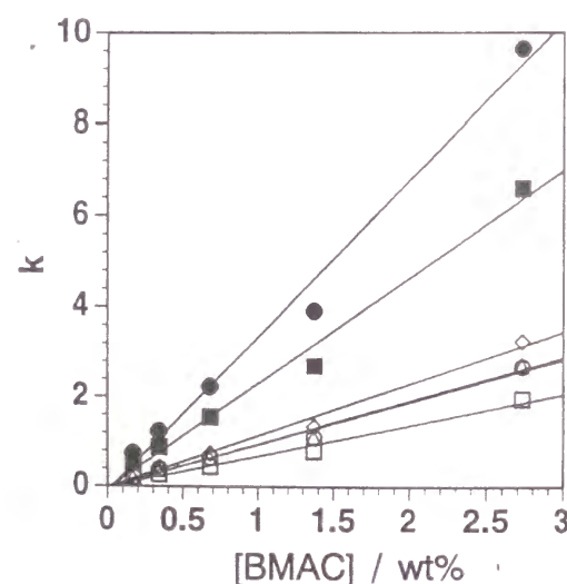
Fig. 3.3 Dependence of the retention factor ( k ) on the concentration of BMAC. Solutes: \square = 1-naphthalenemethanol; \circ = 1,6-dihydroxynaphthalene; \triangle = 1-naphthylamine; \diamond = 1-naphthaleneethanol; \blacksquare = 2-naphthol; \bullet = 1-naphthol. The conditions were the same as in Fig. 3.2(B) except for the concentration of BMAC.
