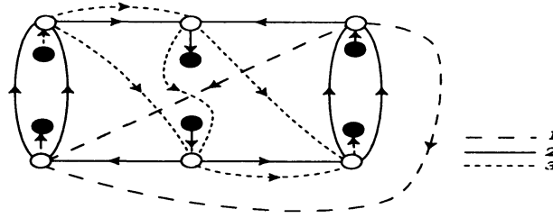
FIGURE 1. Example of a 4-chart
