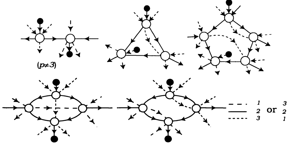
FIGURE 10. \mathfrak{B}
