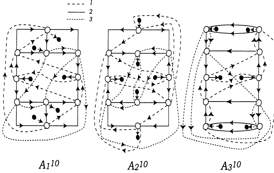
FIGURE 11. A_1^{10} , A_2^{10} and A_3^{10}
