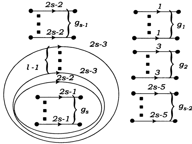
FIGURE 8. B_{s,g_1,\dots,g_s}^l
