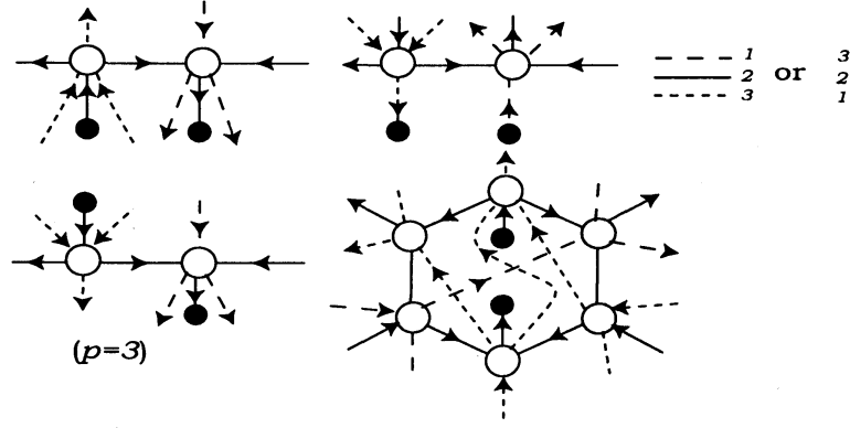
FIGURE 9. \mathfrak{A}
