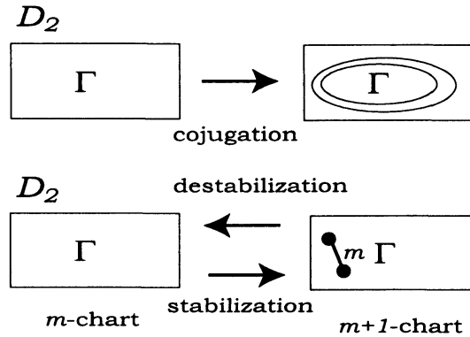
FIGURE 4. Conjugations, stabilizations and destabilizations
