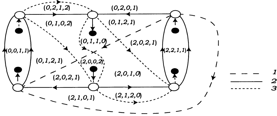
FIGURE 6. Example of an R_3 -coloring
