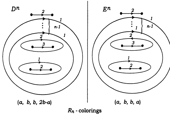
FIGURE 7. D^n | E^n
