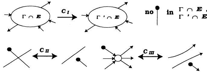
FIGURE 3. C -moves
