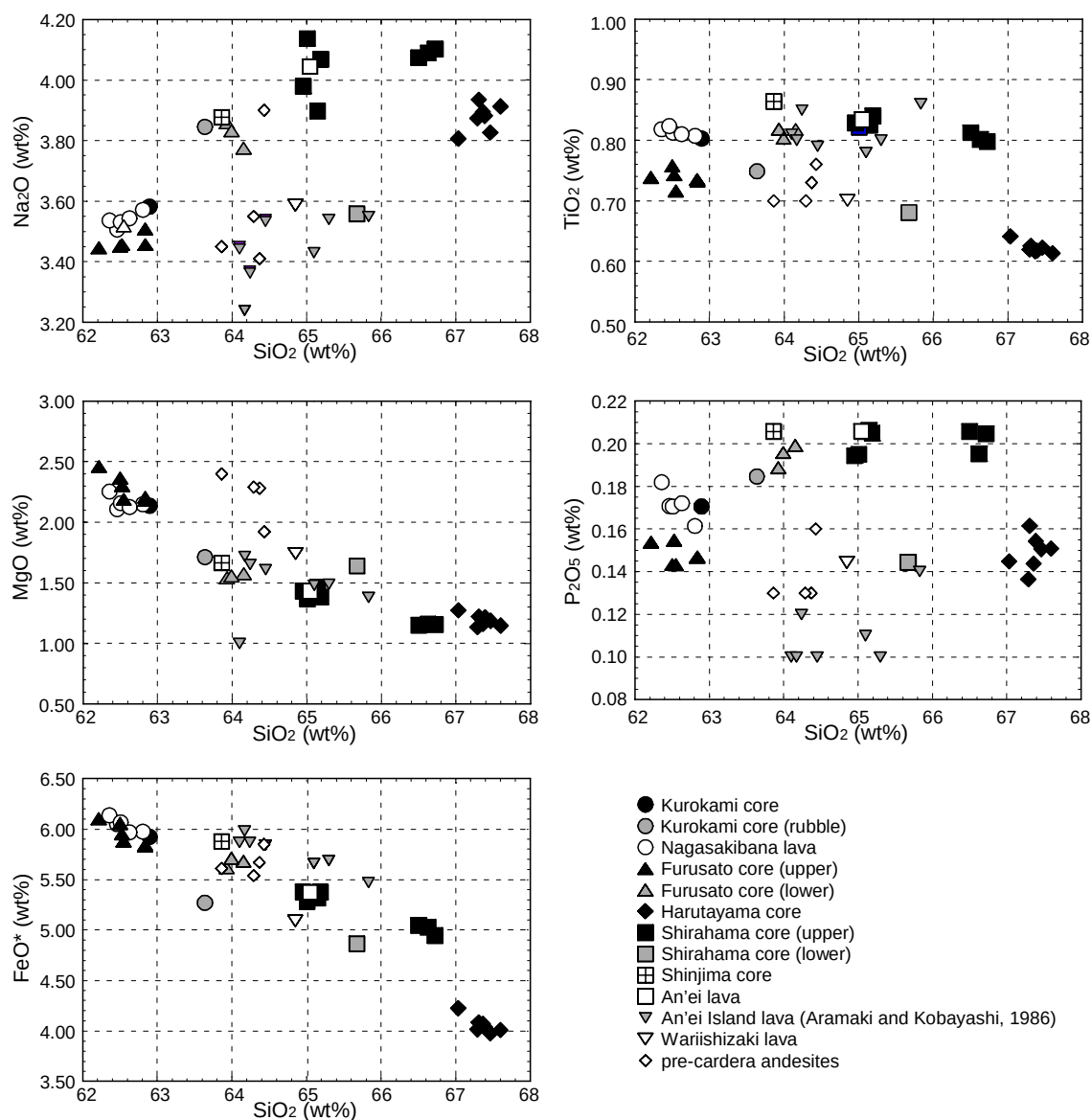
Fig. 2 Chemical compositions of lavas around Sakurajima volcano
