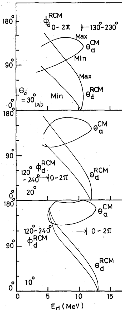
Fig. 12. The relation of the deuteron energy ( E_d ) versus the inelastic scattering angle of alpha-particles in the center-of-mass system ( \theta_\alpha^{\text{CM}} ) and versus the deuteron angle in the recoil center-of-mass system ( \theta_d^{\text{RCM}} , \phi_d^{\text{RCM}} ) in the sequential decay kinematics of the {}^6\text{Li} + \alpha \rightarrow {}^6\text{Li}_{2.18}^* + \alpha \rightarrow \alpha + d + \alpha reaction. See the caption for Fig. 10.
