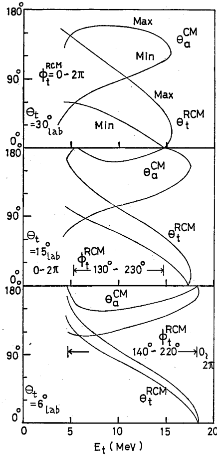
Fig. 10. The relation of the triton energy ( E_t ) versus the inelastic scattering angle of alpha-particles in the center-of-mass system ( \theta_\alpha^{CM} ) and versus the triton angle in the recoil center-of-mass system ( \theta_t^{RCM} , \phi_t^{RCM} ) in the sequential decay kinematics of the {}^7\text{Li} + \alpha \rightarrow {}^7\text{Li}_{4.63}^* + \alpha \rightarrow \alpha + \alpha + t reaction. Only the maximum and the minimum of the corresponding \theta_\alpha^{CM} , \theta_t^{RCM} and \phi_t^{RCM} are shown.
