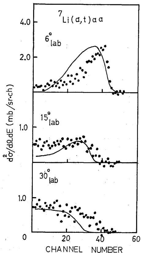
Fig. 11. The calculated energy spectra of tritons assuming a sequential decay, {}^7\text{Li} + \alpha \rightarrow {}^7\text{Li}_{4.68}^* + \alpha \rightarrow \alpha + t + \alpha , using a PWBA theory. The calculated results are normalized to the experimental spectra at the maximum of the anomalous broad peak. The experimental spectra were obtained by subtracting the smooth background under the anomalous peak.
