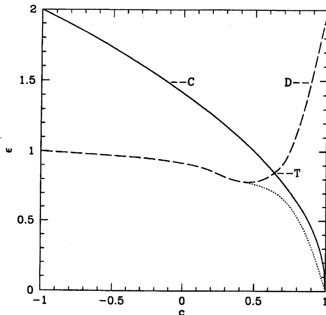
Figure 1: Percolation phase diagram of the O(3) model on the T lattice. C is the line c = 1 - \epsilon^2/2 ; above the dashed line D \mathcal{S}_\epsilon percolates, above the dotted line \langle \mathcal{S}_\epsilon \rangle < \infty .
