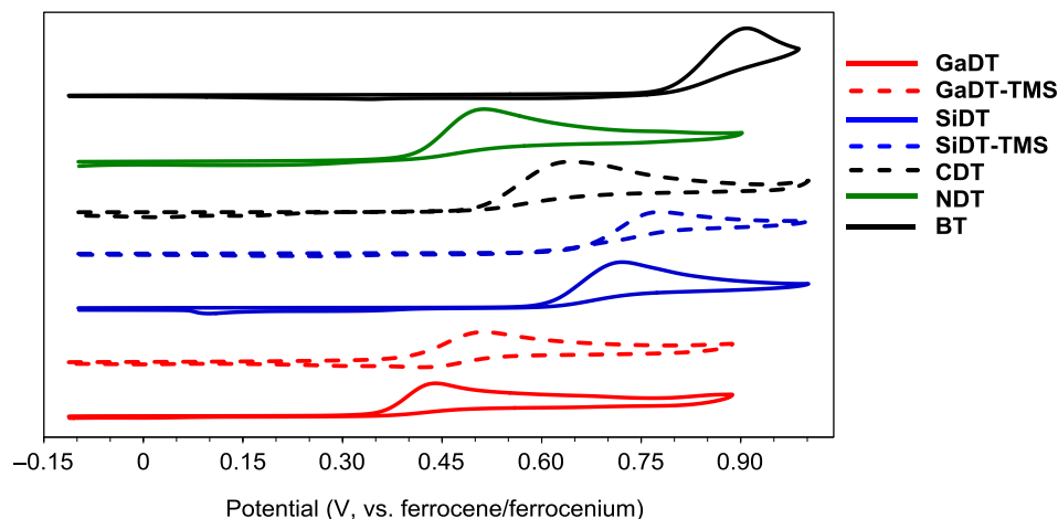
Figure 4. Cyclic voltammograms of 1.0 mM GaDT (solid red), GaDT-TMS (dashed red), SiDT (solid blue), SiDT-TMS (dashed blue), CDT (dashed black), NDT (solid green) and BT (solid black) in \text{CH}_3\text{CN}/\text{CH}_2\text{Cl}_2 (6:1) solution containing \text{NBu}_4\text{PF}_6 (0.10 M) using a Pt working electrode, a Pt wire counter electrode, an Ag/AgCl reference electrode, and a ferrocene/ferrocenium external standard at room temperature with a scan rate of 0.05 \text{ V s}^{-1} .
