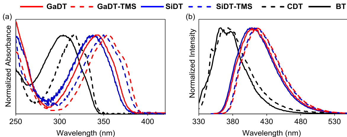
Figure 3. (a) UV-vis absorption and (b) photoluminescence (excited at \lambda_{\text{max,abs}} ) spectra of 1.0 \times 10^{-5} M GaDT (solid red), GaDT-TMS (dashed red), SiDT (solid blue), SiDT-TMS (dashed blue), CDT (dashed black) and BT (solid black) in THF.
