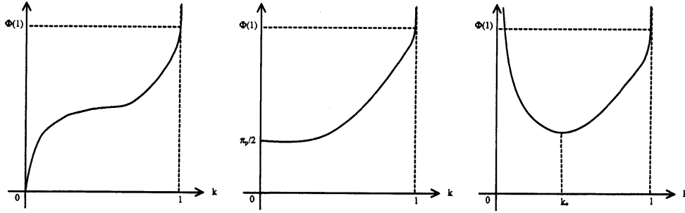
Figure 6: Graphs of \Phi(k) for p > q , p = q and p < q in case p > 2 , where \Phi(1) = 2^{\frac{1}{p}-1} \pi_{\frac{p}{2}, q} .
