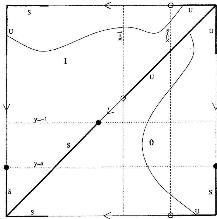
FIGURE 1. Real partition by \text{supp } \eta . The critical set of f/f^{-1} is shown as dashed/dotted lines, indeterminacy set of f/f^{-1} as hollow/solid circles, and sample stable arcs as wavy lines. The arrows indicate the direction of motion of points under iteration of f .
