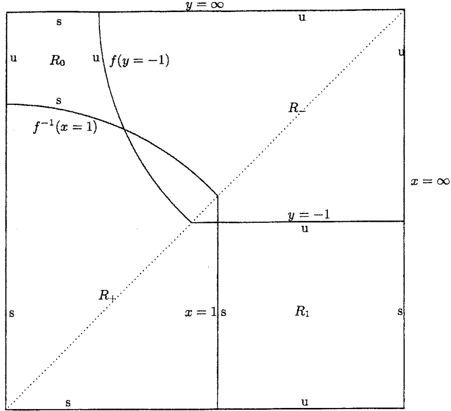
FIGURE 2. Refinement of the original partition to include critical curves. Stable and unstable boundary segments are labeled 's' and 'u', respectively.
