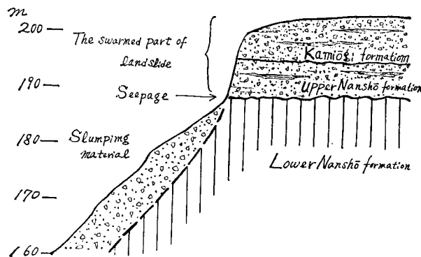
Fig. 11 Schematic profile
