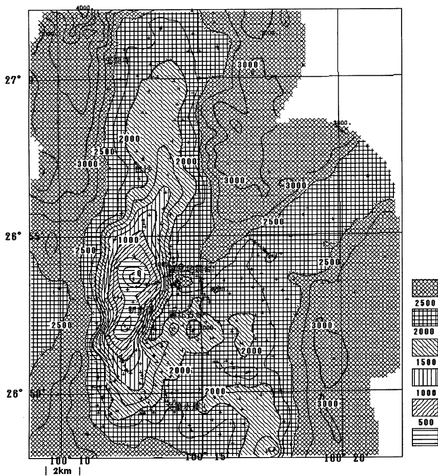
Fig.4 Gravity Basement of Lijiang Basin. Density contrast is 0.5\text{g/cm}^3 by assuming that basement is 2.5\text{ g/cm}^3 and sedimentary layer is 2.0\text{ g/cm}^3 . Contour interval is 250m.
