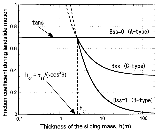
Fig. 5 The change of friction coefficient during landslide motion with thickness of sliding mass and B_{ss}
