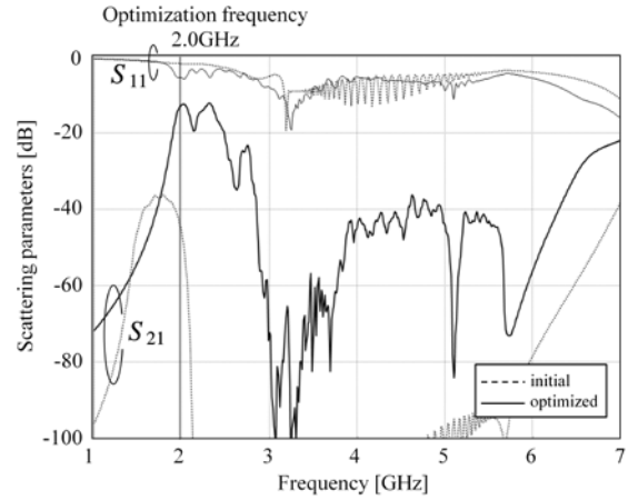
Fig 3. Frequency characteristics of scattering parameters S_{11} and S_{21} of Example 1, maximizing S_{21} at 2.0 GHz
