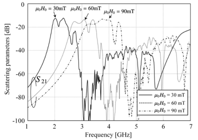
Fig 4. Frequency characteristics of scattering parameter S_{21} obtained using the optimized configuration of Example 1, with \mu_0 H_0 = 30 \text{ mT} , 60 mT and 90 mT, respectively.
