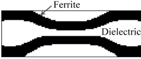
Fig 2. Optimized configuration of Example 1.
