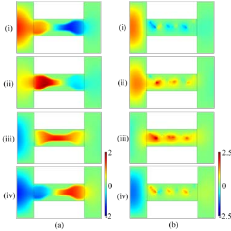
Fig 7. Electric fields of optimized configuration: (a) Example 1 at 2.0 GHz; (b) Example 2 at 3.25 GHz for various phases of incident waves: (i) 0°; (ii) 60°; (iii) 120°; (iv) 180°.
