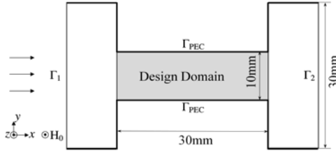
Fig 1. Design domain and boundary conditions.
