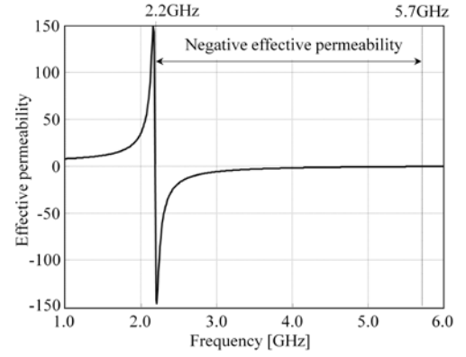
Fig 8. Effective permeability curve of the ferrite material.
