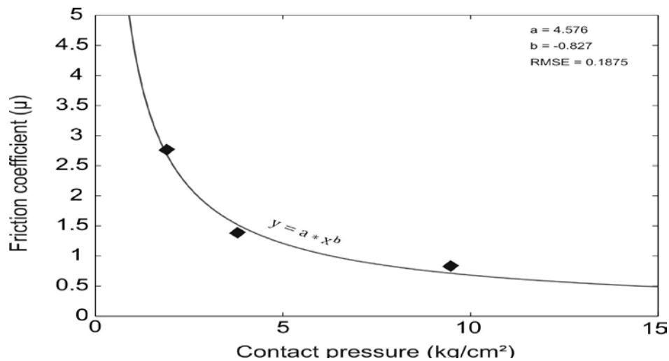
Figure8. Contact pressure and friction coefficient relationship.
