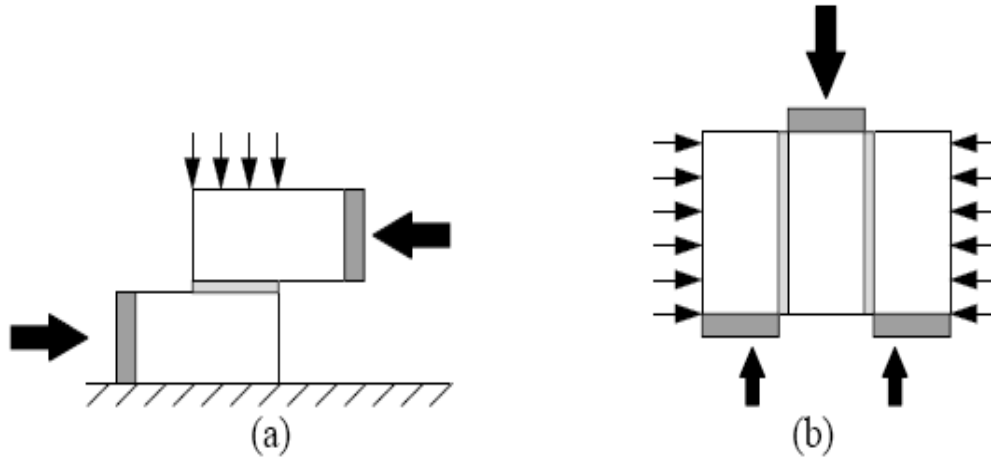
Figure1. Possible test set-ups for determination of shear bind strength: a) couple test b) triplet test.
