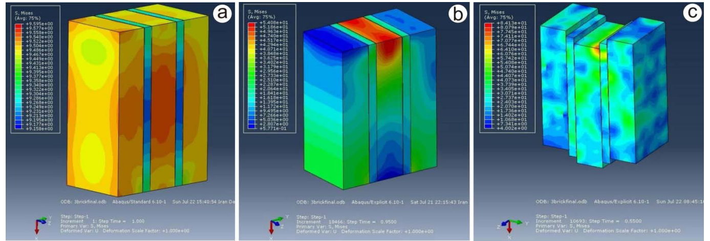
Figure7. a) Stress distribution in step 1 (applying the horizontal stress). b) Stress distribution in step 2 (applying vertical deviator load to break the specimen). c) Stress distribution of the fractured triplet specimen.
