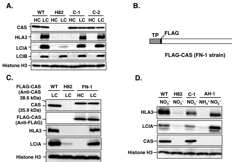
Figure 24. Accumulation of CAS, HLA3, LCIA, and LCIB in wild-type (WT), H82, C-1, C-2, FN-1, and AH-1 cells. (A) Cells were grown in medium with \text{NH}_4^+ as the nitrogen source in high- \text{CO}_2 (HC) or low- \text{CO}_2 (LC) conditions for 12 h. Histone H3 was used as a loading control. (B) Schematic representation of recombinant CAS proteins in complemented strain (FN-1) expressing FLAG-tagged CAS. The gray, solid, and open rectangles indicated the transit peptide (TP), FLAG-tag, and CAS, respectively. (C) Accumulation levels of LCIA, HLA3, and recombinant CAS in FN-1 cells were recorded. Cells were grown in HC or LC conditions for 12 h. (D) Cells were grown in medium with \text{NH}_4^+ or \text{NO}_3^- as nitrogen sources in LC conditions for 12 h.
