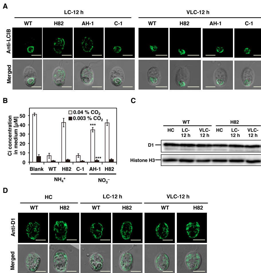
Figure 27. Subcellular localization of LCIB and D1 in H82 mutant and inorganic carbon (Ci) concentration in growth medium. (A) Localization of LCIB in wild-type (WT), H82, AH-1, and C-1 cells using an indirect immunofluorescence assay. High-CO 2 (HC)-grown cells were transferred to low-CO 2 (LC) or very LC (VLC) conditions for 12 h. AH-1 cells were cultured in HSM medium with NO 3 - (HSM-NO 3 - ) as the nitrogen source. Each image is placed with the flagella facing upward on the panel. Merged indicates the merger of a fluorescence image with its differential interference contrast (DIC) image. Scale bars, 5 μm. (B) Measurement of Ci concentrations in HSM medium with NH 4 + (HSM-NH 4 + ) as the nitrogen source or HSM-NO 3 - medium after culturing cells in 0.04% or 0.003% CO 2 for 12 h. Blank means the Ci concentrations in culture medium without cells. Data in all experiments are mean values ± SD from three biological replicates. The difference of the Ci concentration in medium between AH-1 and H82 cells was evaluated. *** P < 0.1 by Student's t test. (C and D) Accumulation (C) and subcellular localization (D) of D1 in HC-, LC-, and VLC-grown WT and H82 cells.
