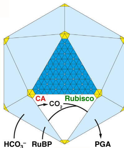
Figure 6. Schematic diagram of the carboxysome (modified from Cameron et al., 2013). The carboxysome shell is comprised of hexameric (blue) and pentameric (yellow) proteins that enclose enzymes of the Calvin–Benson–Bassham (CBB) cycle including almost all Rubisco (green). Bicarbonate ( \text{HCO}_3^- ) is converted to \text{CO}_2 by carbonic anhydrase (CA, red) in the carboxysome for \text{CO}_2 fixation.
