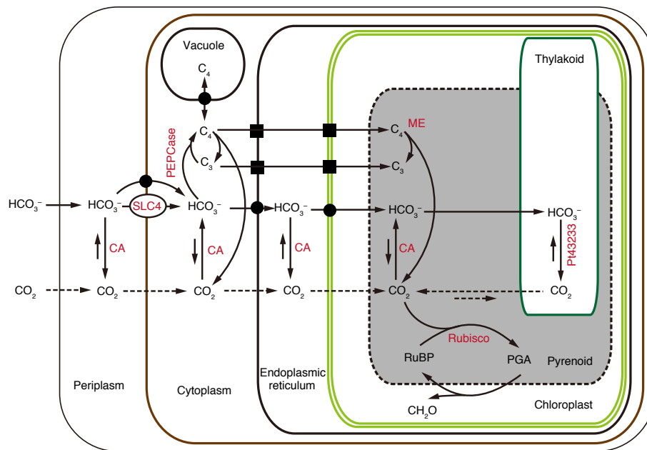
Figure 5. Schematic presentation of the possible \text{CO}_2 -concentrating mechanism (CCM) in diatoms in \text{CO}_2 -limiting conditions (modified from Roberts et al., 2007; Nakajima et al., 2013; Kikutani et al., 2016). The scheme shows the proposed uptake of inorganic carbon (Ci) from the extracellular space to the thylakoid lumen. The possible involvement of \text{C}_4 acid in the diatom CCM is also illustrated. The unknown Ci transporters are shown as closed circles. The transporters for \text{C}_3 or \text{C}_4 acid are indicated as closed squares. The broken lines indicate the diffusion paths of \text{CO}_2 . CA, carbonic anhydrase. PEPCase, phosphoenolpyruvate carboxylase; ME, malic enzyme; RuBP, ribulose-1,5-bisphosphate; PGA, phosphoglyceric acid; SLC4, Ci transporters (Nakajima et al., 2013); Pt43233, thylakoid lumen-localized \theta -CA (Kikutani et al., 2016).
