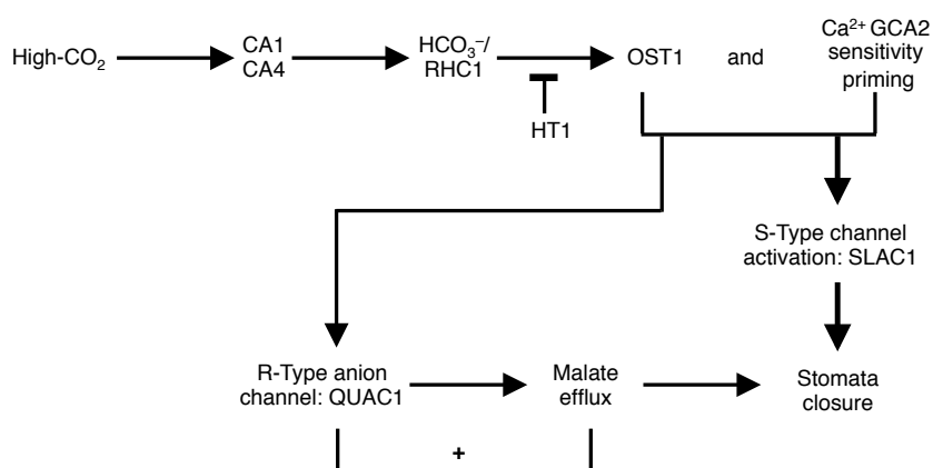
Figure 1. A model illustrating the functions of proteins in guard cells mediating CO 2 control of stomata movements (modified from Engineer et al., 2016). In this model, the HT1 protein kinase functions as a negative regulator. CA1, CA4, OST1, GCA2, QUAC1 and SLAC1 function as positive mediators of high-CO 2 -induced stomata closure. Abbreviations: CA, carbonic anhydrase; HT1, high temperature 1; RHC1, resistance to high-CO 2 1; OST1, open stomata 1; GCA2, growth controlled by abscisic acid 2; QUAC1, quickly activating anion channel 1; SLAC1, slow anion channel associated 1. '+' indicates that the extracellular malate can increase the activity of QUAC1.
