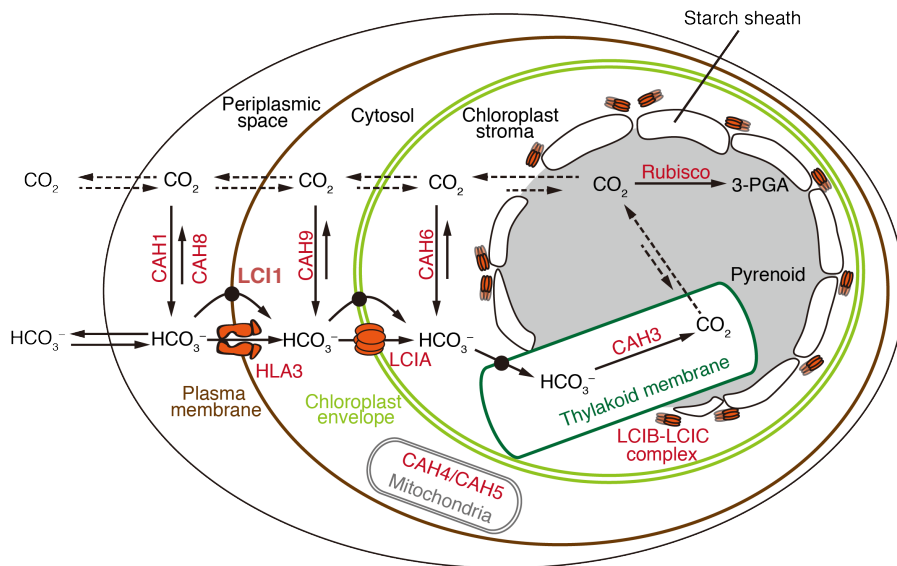
Figure 4. Schematic model of \text{CO}_2 -concentrating mechanism (CCM) in Chlamydomonas reinhardtii in \text{CO}_2 -limiting conditions. (modified from Moroney and Ynalvez, 2007; Wang et al., 2015; Yamano et al., 2015). The proposed uptake of inorganic carbon ( \text{Ci} ) from the extracellular space to the thylakoid lumen is illustrated. In \text{CO}_2 -limiting conditions, the pyrenoid develops as a spherical structure surrounded by starch sheaths. The unknown \text{Ci} transporters are shown as closed circles. The broken lines indicate the diffusion paths of \text{CO}_2 . CAH, carbonic anhydrase in Chlamydomonas reinhardtii .
