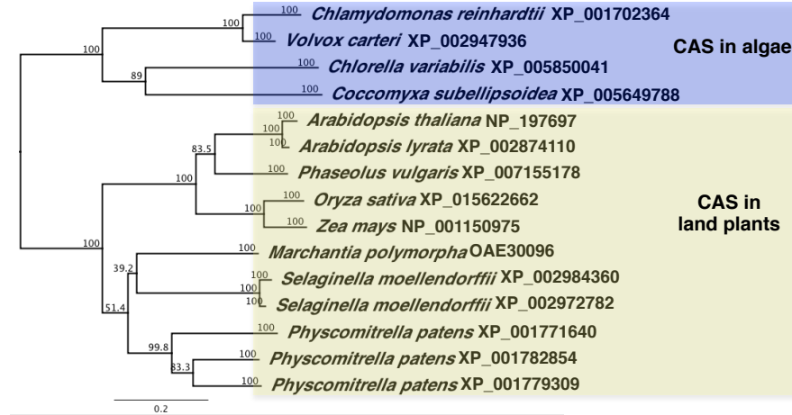
Figure 9. Domain structure and phylogenetic tree of homologous calcium ( \text{Ca}^{2+} )-sensing receptor (CAS). (A) Schematic presentation of the domain structure of CAS. (B) Alignment of Chlamydomonas CAS with the amino acid sequences of putative homologous proteins from Chlamydomonas reinhardtii , Volvox carteri , Arabidopsis thaliana , and Oryza sativa . The rectangles with white, black, and gray colors represent chloroplast transit peptide, hydrophobic sequence, and rhodanese-like domain, respectively. (C) The phylogenetic tree was constructed using the neighbor-joining method. Bootstrap values are calculated over 1,000 replicates.
