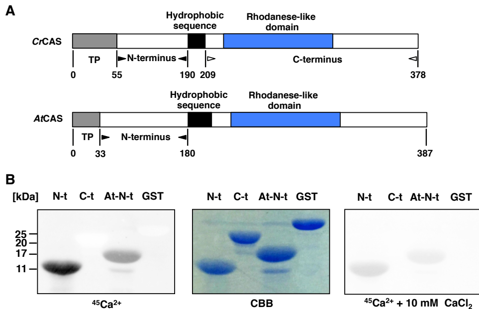
Figure 33. \text{Ca}^{2+} -binding activity of Cr CAS in vitro . (A) The N-terminus and C-terminus of CAS are separated by a hydrophobic sequence. The gray, solid, and blue rectangles indicate the transit peptide, hydrophobic sequence, and rhodanese-like domain, respectively. The numbers below the illustration represent the positions from the initial amino acid. The transit peptide of At CAS was predicted using the ChloroP program. (B) ^{45}\text{Ca} blotting analysis of the N- and C-terminus (N-t and C-t, respectively) of the CAS protein. Purified recombinant N-t, C-t, N-terminus of At CAS (At-N-t), and GST with the same number of molecules were loaded, stained with Coomassie Brilliant blue (B, middle), and probed with ^{45}\text{Ca} in the absence (B, left) or presence (B, right) of 10 mM cold \text{CaCl}_2 . kDa, kilodalton.
