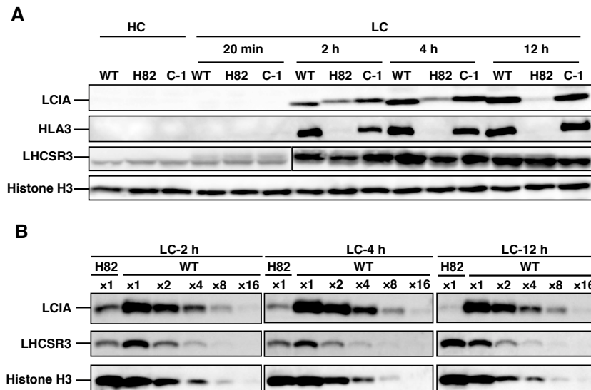
Figure 26. Accumulation of HLA3, LCIA, and LHCSR3 in wild-type (WT), H82, and C-1 cells. (A) High-CO 2 (HC)-grown cells were transferred to low-CO 2 (LC) conditions for 0.3, 2, 4, or 12 h before sampling. Cells were illuminated in 120 \mu\text{mol photons}\cdot\text{m}^{-2}\cdot\text{s}^{-1} . Histone H3 was used as a loading control. (B) To compare the accumulation levels of these proteins in H82 cells with that of WT cells, aliquots of total cell protein corresponding to 1 \mu\text{g} of chlorophyll were loaded in the lane designated \times 1 , and the same amount of protein was serially diluted 2–16 times and loaded in the lanes designated \times 2 , \times 4 , \times 8 , and \times 16 , respectively.
