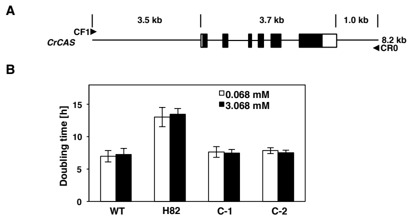
Figure 20. The growth rate of H82 and its complemented strains. (A) Schematic representation of the fragment introduced into H82 cells for complementation. The solid rectangles indicate the exons of the CAS gene. The open rectangles represent the 5'-UTR (left) and 3'-UTR (right). This fragment was amplified using primers CF1 and CR0. (B) The doubling time of wild-type (WT), H82, and its complemented strains (C-1 and C-2) in low- \text{CO}_2 (LC) conditions at pH 7.0. The optical density at 730 nm was measured at four time-points (0, 12, 24, and 36 h) for calculating the doubling time.
