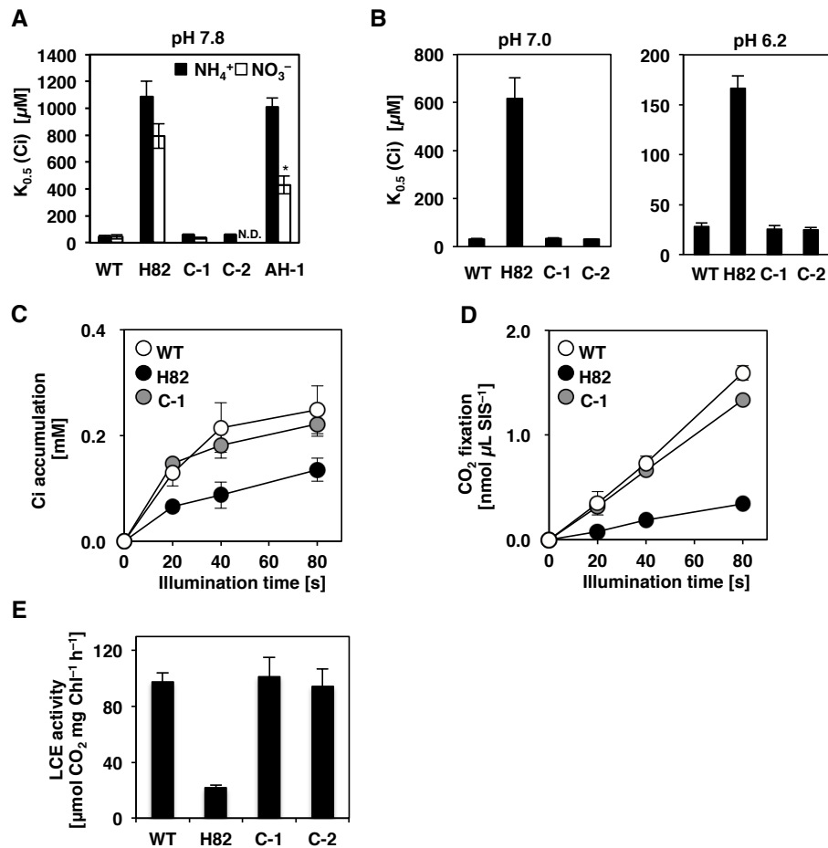
Figure 22. Photosynthetic characterization of H82 and its complemented strains. (A) Photosynthetic inorganic carbon (Ci) affinity of wild-type (WT), H82, its complemented strains (C-1 and C-2), and transgenic H82 cells containing inducible genes of HLA3 and LCIA (AH-1) cells grown in medium with \text{NH}_4^+ or \text{NO}_3^- as nitrogen sources in low- \text{CO}_2 (LC) conditions for 12 h. Photosynthetic \text{O}_2 -evolving activity was measured in external dissolved Ci concentrations at pH 7.8, and the Ci concentration required for half maximal velocity ( K_{0.5} (Ci)) was calculated. Data in all experiments are mean values \pm standard deviation (SD) from three biological replicates. * P < 0.01 by Student's test. N.D., not determined. (B) Photosynthetic Ci affinity of WT, H82, C-1, and C-2 in medium with \text{NH}_4^+ as nitrogen source in LC conditions for 12 h. Photosynthetic \text{O}_2 -evolving activity was measured at pH 7.0 or 6.2. (C and D) Accumulation (C) and fixation (D) of Ci in WT, H82, and C-1 cells. Cells were grown in LC conditions for 12 h, and the intracellular Ci concentration and carbon fixation were measured using a silicone-oil layer method. SIS, sorbitol impermeable space. (E) Light-dependent \text{CO}_2 -exchange (LCE) activity of WT, H82, C-1, and C-2. Cells were grown in LC conditions for 12 h.
