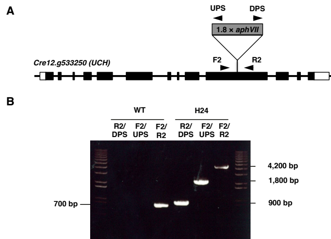
Figure 17. Molecular characterization of the H24 mutant. (A) Schematic representation of the aphVII insertion into the genome of the H24 mutant. The UTR , exon, and aphVII are shown as white, black, and gray boxes, respectively. (B) Confirmation of aphVII insertion by genomic PCR. Genomic PCR was performed using the primer sets depicted in (A). WT, wild-type; bp, base pair; M, marker.
