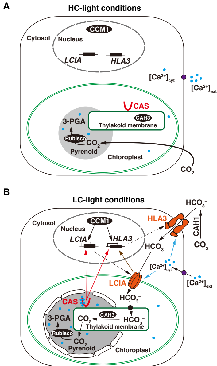
Figure 36. A tentative model illustrating how CAS protein and \text{Ca}^{2+} regulate the expression of HLA3 and LCIA during CCM induction by switching from high- \text{CO}_2 (HC)-light (A) to low- \text{CO}_2 (LC)-light (B) conditions. The red structure indicates the CAS protein. The CAS-mediated pathways involved in regulating the expression of HLA3 and LCIA are shown as red arrows. The purple dot indicates a putative plasma membrane-localized \text{Ca}^{2+} transporter. The \text{Ca}^{2+} -mediated pathways involved in regulating accumulation of HLA3 and LCIA are represented as blue arrows. \text{Ca}^{2+} ions are indicated as blue dots. The LCIA -mediated pathway involved in regulating expression of HLA3 is indicated as brown arrows. PGA, phosphoglyceric acid; CAH, carbonic anhydrase.
