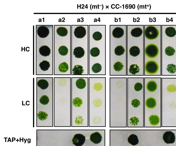
Figure 19. Tetrad analysis of the H24 mutant. Genetic separation of the high-CO 2 (HC)-requiring phenotype and hyg resistance. Tetrad progenies (a and b sets) were obtained from crosses of H24 (mt - ) and CC-1690 (mt + ) strains. LC, low-CO 2 .
