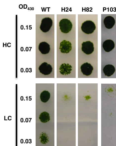
Figure 11. Spot test of wild-type (WT) and high-CO 2 (HC)-requiring mutants H24, H82, and P103. Cells grown to logarithmic phase were diluted to the indicated optical density at 430 nm (OD 430 =0.15, 0.07, or 0.03). Then 3 \mu L of each cell suspension was spotted on HSM plates and incubated for 9 days in growth chambers supplied with HC or low-CO 2 (LC) in continuous light at 120 \mu mol photons·m -2 ·s -1 .
