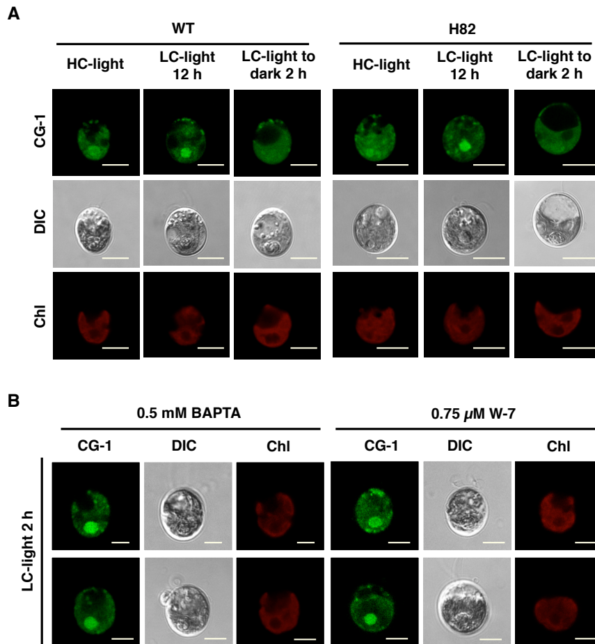
Figure 35. Calcium Green-1, AM (CG-1) fluorescence in wild-type (WT) and H82 cells, and the effect of 1,2-bis (o-aminophenoxy) ethane-N, N, N, N'-tetraacetic acid (BAPTA) or N-(6-aminoethyl)-5-chloro-1-naphthalenesulfonamide hydrochloride (W-7) on the fluorescence of Calcium Green-1 AM. (A) Cells were grown in high-CO 2 (HC) or low-CO 2 (LC) conditions for 12 h in light or cells in LC-light conditions were transferred to LC-dark conditions for 2 h, then incubated with CG-1 at room temperature for 30 min. Fluorescence images derived from CG-1 treatments and chlorophyll (Chl) are shown. Each image is placed with the flagella facing upward on the panel. DIC, differential interference contrast image. Scale bars, 5 μm. (B) Cells were grown in LC-light conditions for 2 h. The chemical being tested was added to fresh medium before shifting from HC to LC conditions.
