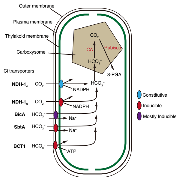
Figure 3. A model of the \text{CO}_2 -concentrating mechanism (CCM) in cyanobacteria (modified from Price et al., 2011). The paths of inorganic carbon ( \text{Ci} ) in the cyanobacteria CCM. The ellipses indicate three types of identified \text{Ci} transporters, including constitutive (blue), inducible (red), and mostly inducible (purple). CA, carbonic anhydrase; PGA, phosphoglyceric acid. Mostly Inducible protein is accumulated in sufficient \text{CO}_2 , but much higher in \text{CO}_2 -limiting conditions.
