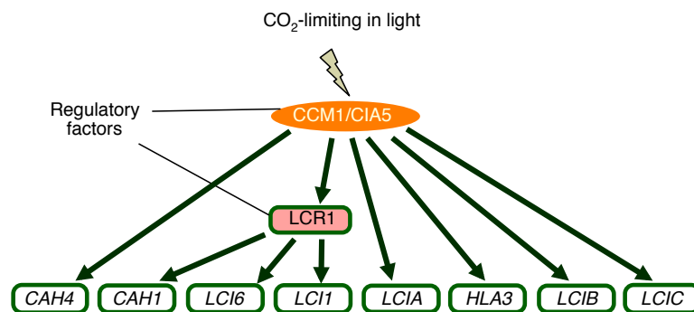
Figure 8. A model for CO 2 -dependent regulatory network in Chlamydomonas reinhardtii (modified from Yoshioka et al., 2004 ). Two regulatory factors including CCM1/CIA5 and low-CO 2 (LC)-inducible DNA-binding transcriptional factor (LCR1) are presented. CAH1 and CAH4 are genes encoding carbonic anhydrases. LC-inducible 1 ( LCI1 ) and high-light activated 3 ( HLA3 ) are genes encoding two plasma membrane-localized inorganic carbon (Ci) transporters. LC-inducible A ( LCIA ) is a gene encoding chloroplast envelop-localized Ci channel. LC-inducible B ( LCIB ) and LC-inducible C ( LCIC ) are genes encoding proteins for recycling of leaked CO 2 from pyrenoid. LC-inducible gene 6 ( LCI6 ).
