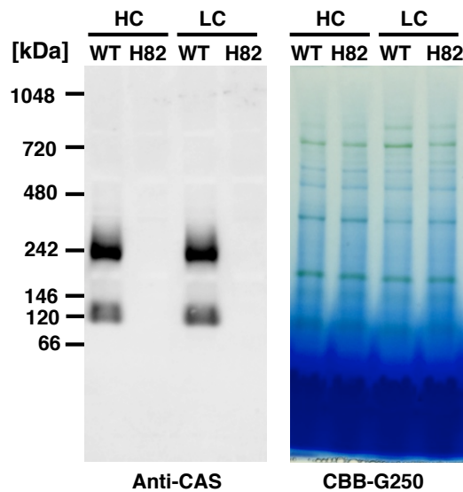
Figure 32. Molecular mass of native CAS protein. Wild-type (WT) and H82 cells were grown in high- \text{CO}_2 (HC) or low- \text{CO}_2 (LC) conditions for 12 h. Total proteins were dissociated using 0.5% n-dodecyl \beta -D-maltoside and separated by blue-native PAGE, in which the gel was stained by Coomassie Brilliant Blue-G250 (right). The PVDF membrane was subjected to an immunoblotting assay using an anti-CAS (C) antibody.
