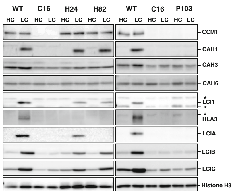
Figure 14. Accumulation of CCM-related proteins. Accumulation of CCM-related proteins in wild-type (WT), C16, H24, H82, and P103 cells was analyzed by immunoblotting analysis. Cells were grown in high-CO 2 (HC) conditions for 12 h and then shifted to HC or low-CO 2 (LC) conditions for 12 h. Histone H3 was used as a loading control. Asterisks indicate the nonspecific protein bands.
