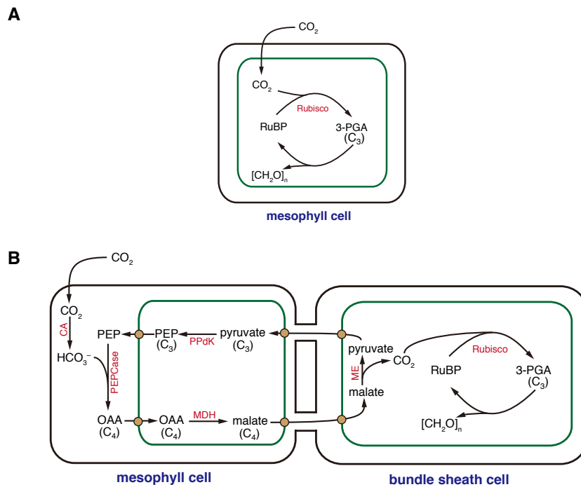
Figure 2. Schematic diagrams of C 3 Calvin–Benson–Bassham (A) and C 4 cycles for CO 2 fixation (modified from Langdale et al., 2011). (A) In C 3 plants, CO 2 is fixed in mesophyll cells by Rubisco. (B) In C 4 plants, CO 2 is first converted to C 4 acid in mesophyll cell and then transferred into bundle sheath cell for fixation by Rubisco. The green squares indicate the chloroplast envelope. The proteins involved in these pathways are shown in red. The yellow dots indicate proteins involved in transportation of intermediates. RuBP, ribulose-1,5-bisphosphate; PGA, phosphoglyceric acid; PEPCase, phosphoenolpyruvate carboxylase; OAA, oxaloacetic acid; MDH, malate dehydrogenase; PPdK, pyruvate, phosphate dikinase; ME, malic enzyme; CA, carbonic anhydrase.
