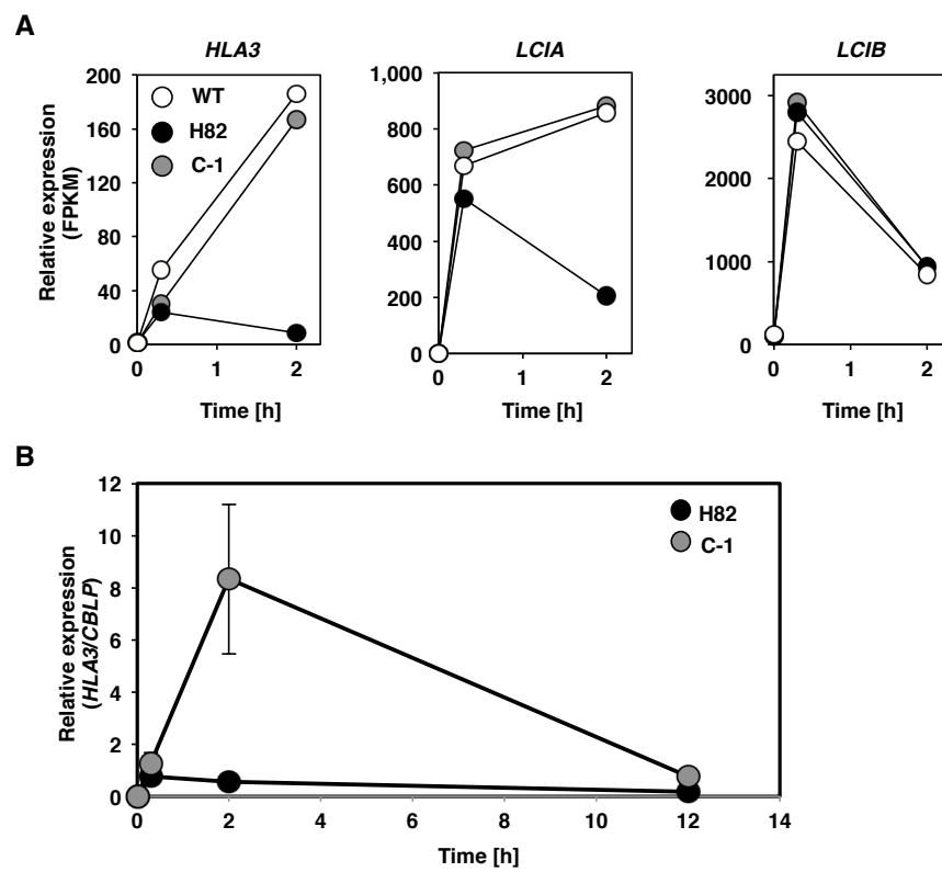
Figure 25. Time course of relative expression of HLA3 , LCIA , and LCIB . (A) Time course of fragments per kilobase of exon per fragments mapped (FPKM) values of LCIA , HLA3 , and LCIB in wild-type (WT), H82, and C-1 cells by RNA-seq analysis. Each strain grown in high- \text{CO}_2 (HC, 0 h) conditions was transferred to low- \text{CO}_2 (LC) conditions for 0.3 or 2 h. FPKM values calculated from two biological replicates. (B) The expression of HLA3 was analyzed in H82 and C-1 cells at the indicated time points by qRT-PCR. CBLP gene encoding Chlamydomonas beta subunit-like polypeptide was used as an internal standard. Data in all experiments are mean values \pm SD from three biological replicates. Each strain grown in HC (0 h) conditions was transferred to LC conditions for 0.3, 2, or 12 h.
