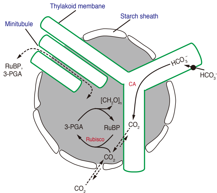
Figure 7. Schematic diagram of pyrenoid structure and the function of the pyrenoid in \text{CO}_2 -concentrating mechanism (CCM) (modified from Meyer et al., 2015). The pyrenoid is surrounded by starch sheaths and encapsulates enzymes of Calvin–Benson–Bassham (CBB) cycle, including more than 90% of Rubisco. In \text{CO}_2 -limiting conditions, the amount of \text{CO}_2 from passive diffusion is decreased. Most \text{CO}_2 comes from active uptake by \text{HCO}_3^- transporters (closed circle) into the thylakoid lumen, and \text{HCO}_3^- is converted into \text{CO}_2 by carbonic anhydrase (CA) in acidic lumen conditions. Subsequently, the \text{CO}_2 produced diffuses into the pyrenoid matrix for fixation by Rubisco. Small molecules, such as RuBP and 3-PGA, could diffuse between the chloroplast stroma and pyrenoid matrix through the minitubules formed by thylakoid stacks. The broken lines indicate the diffusion paths of \text{CO}_2 .
