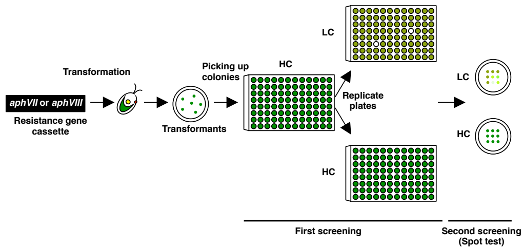
Figure 10. Schematic illustration of screening process. PCR-amplified hygromycin (hyg) or paromomycin (par) resistance gene cassettes were introduced into wild-type (WT) cells by electroporation. Colonies with resistance were picked up, cultured in 96-well microtiter plates under high-CO 2 (HC) conditions, and replicated into two plates. One plate was incubated under HC conditions, and the other one was incubated under low-CO 2 (LC) conditions. By measuring optical density at 700 nm every 12 h, HC-requiring candidates were isolated. The reproducibility of the HC-requiring phenotype was checked by a spot test in second screening.
