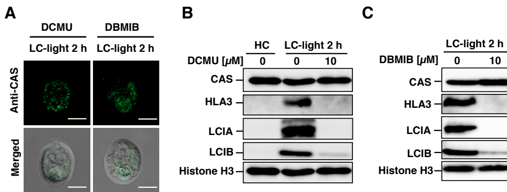
Figure 30. Subcellular localization of CAS and accumulation of CAS, HLA3, LCIA, and LCIB in the presence DCMU or DBMIB. (A) The effect of 3-(3,4-dichlorophenyl)-1,1-dimethylurea (DCMU, 10 μM) or 2,5-dibromo-3-methyl-6-isopropylbenzoquinone (DBMIB, 10 μM) on the localization of CAS in wild-type (WT) cells. High-CO 2 (HC)-grown cells were centrifuged, re-suspended in fresh HSM medium containing the indicated chemicals, and switched to low-CO 2 (LC) conditions for 2 h. (B and C) Accumulation of proteins in WT cells grown in the ethanol (mock, solvent used for inhibitors), DCMU (10 μM), or DBMIB (10 μM).
