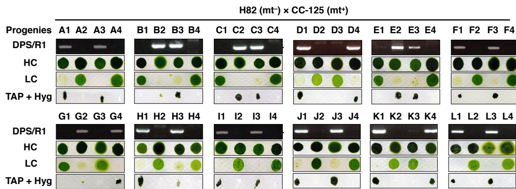
Figure 18. Tetrad analysis of the H82 mutant. Genetic linkage of the hygromycin (hyg) insertion, hyg resistance, and high-CO 2 (HC)-requiring phenotype. Genomic DNA was extracted from tetrad progenies (A–L), obtained from crosses of H82 (mt - ) and CC-125 (mt + ) strains. Genomic PCR was performed with primer sets depicted in Figure 16A. LC, low-CO 2 .
