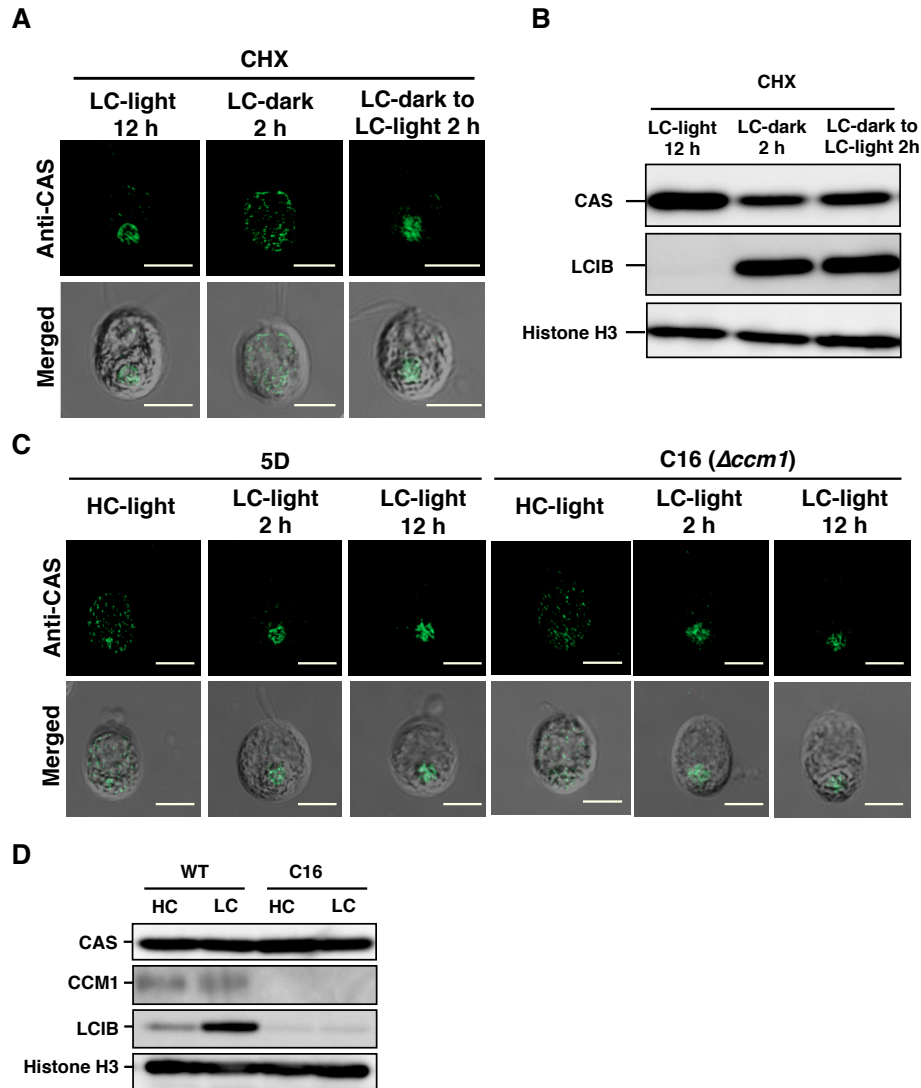
Figure 31. Subcellular localization of CrCAS and accumulation of CAS and LCIB in the presence of cycloheximide (CHX) or the CCM1 insertion mutant. (A) The effect of CHX ( 10 \mu\text{g mL}^{-1} ) on the localization of CAS in wild-type (WT) cells. For CHX treatments, high- \text{CO}_2 (HC)-grown cells were transferred to low- \text{CO}_2 (LC)-light conditions in the presence of CHX for 12 h. The LC-light acclimated cells were subjected to LC-dark conditions in the presence of CHX for 2 h. The LC-dark-acclimated cells were transferred to LC-light conditions with or without CHX for 2 h. For all panels, each image is placed with the flagella facing upward on the panel. Merged images show the fluorescence image superimposed with its differential interference contrast image. Scale bars, 5 \mu\text{m} . (B) The effect of CHX on the accumulation of CAS and LCIB. (C) Localization of CAS in a CCM1 insertion mutant, C16, and its parental 5D strain using an indirect immunofluorescence assay. Cells grown in HC-light conditions were shifted to LC-light conditions for 2 h or 12 h. (D) Accumulation of CAS in WT C-9 strain and C16 cells grown in HC or LC conditions for 12 h in light.
