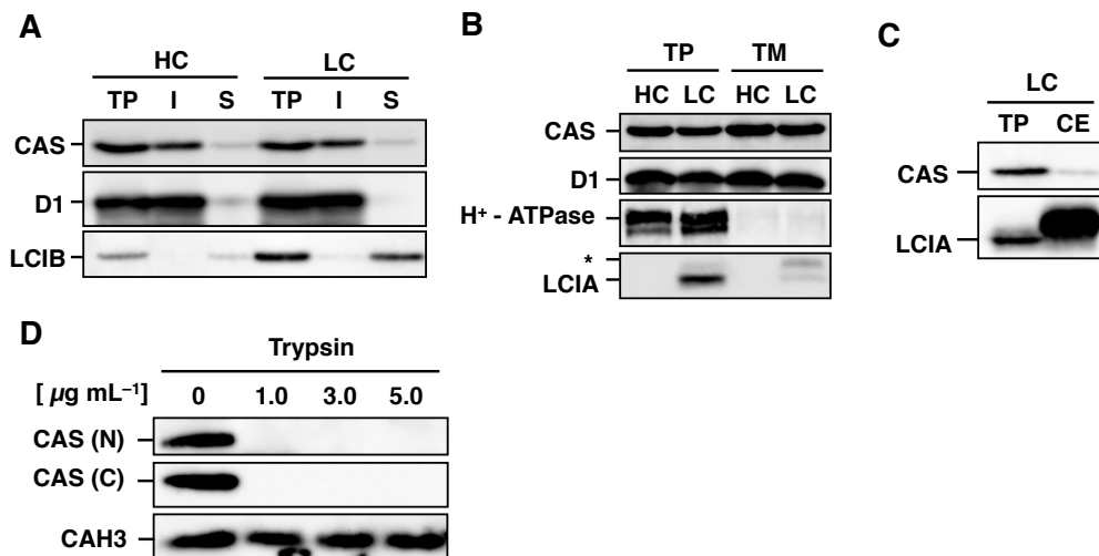
Figure 28. Localization and topology of CrCAS by subcellular fractionation. (A, B, and C) Immunoblotting analysis in soluble, insoluble, thylakoid membrane, and chloroplast envelope fractions with antibodies against CAS, D1, LCIB, H + -ATPase, and LCIA. Cells were grown in high-CO 2 (HC) or low-CO 2 (LC) conditions for 12 h. Asterisks indicate nonspecific bands. TP, total protein; S, soluble fraction; I, insoluble fraction; TM, thylakoid membrane fraction; and CE, chloroplast envelope fraction. (D) Topology of CrCAS. The thylakoid fraction (0.05 mg chlorophyll mL -1 ) isolated from CC-400 cells was suspended in buffer containing trypsin at the indicated concentrations or no protease. The proteins were separated by 15% SDS-PAGE and probed by N-terminal (N)-, C-terminal (C)-specific anti-CAS antibodies or an anti-CAH3 antibody.
