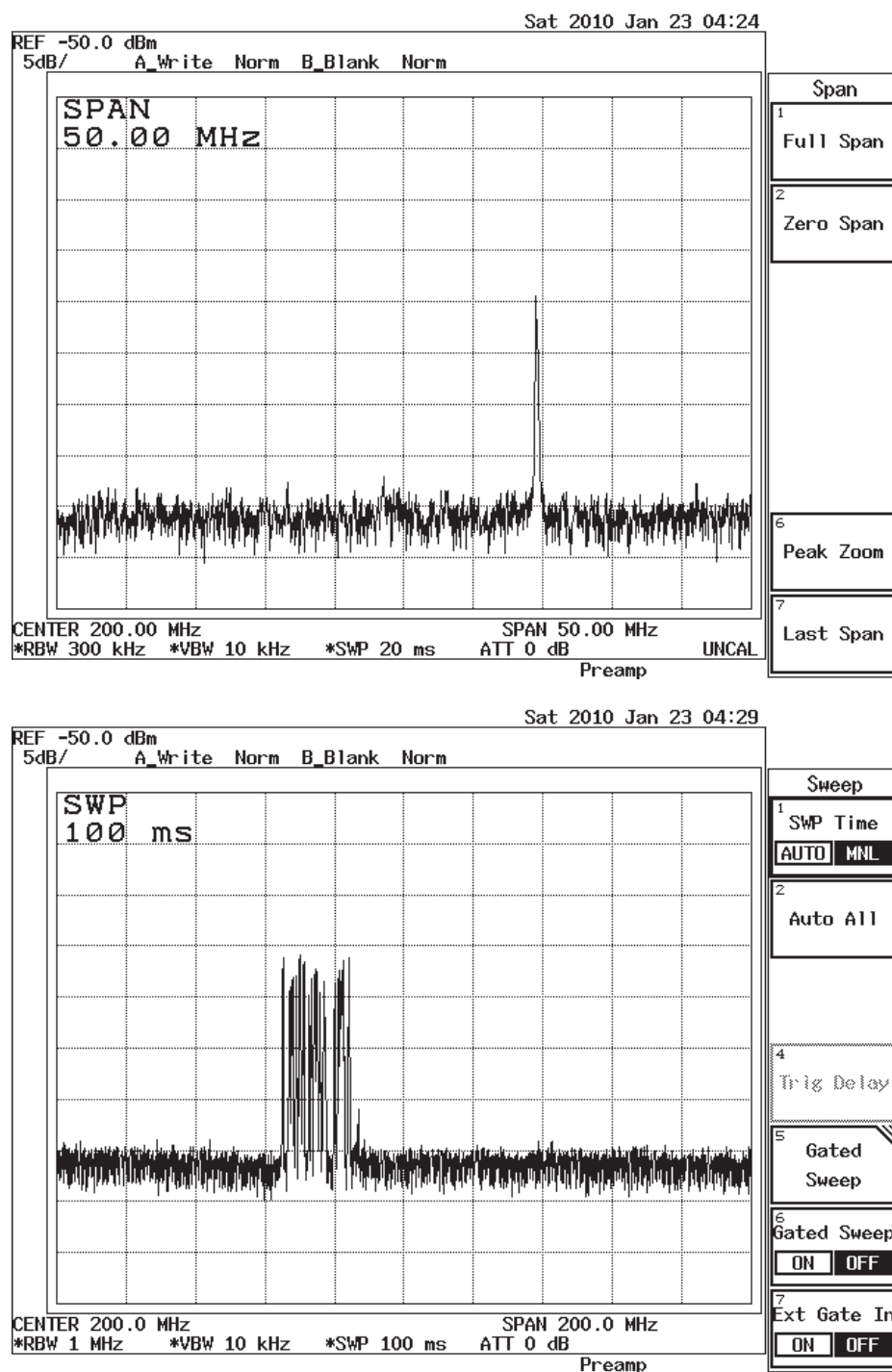
Fig. 3.9 Beat signals between ECLD and frequency-doubled Ti:S laser. Linewidth with single-frequency oscillation is obtained to be 2 MHz (upper figure) and 20 MHz (lower figure) for observation times of below 1 ms and 10 ms, respectively. The observation times are estimated from the sweep times of the RF synthesizer.
