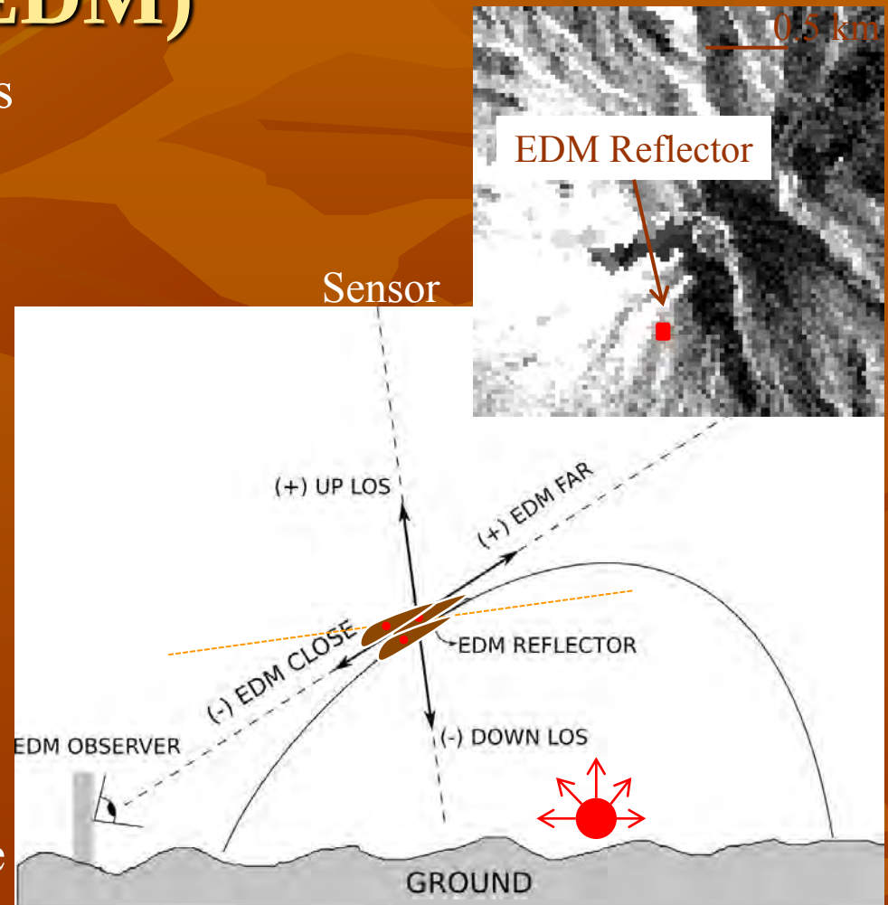
Illustration of LOS displacement and EDM change distance observing same object at the summit of volcano.
