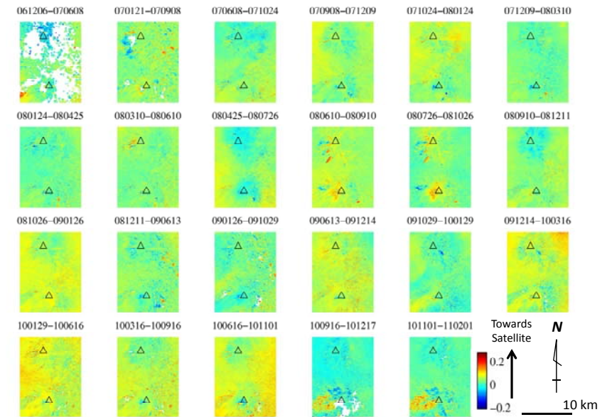
Figure 3. Interferograms after PWL and RLC atmospheric corrections show uncorrelated signal between Mt. Merbabu (North Triangle) and Mt. Merapi (South Triangle).
