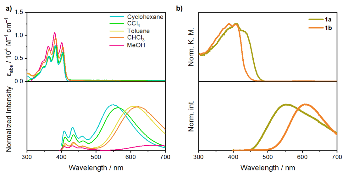
Figure 3. a) UV-Vis absorption (top) and PL spectra (bottom) of 1 in various solvents (1.0 × 10 -5 M). b) diffusion reflectance (top) and PL (bottom) spectra of 1a and 1b .
