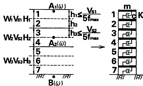
Fig.4.6 Modeling for multi-layered ground model
