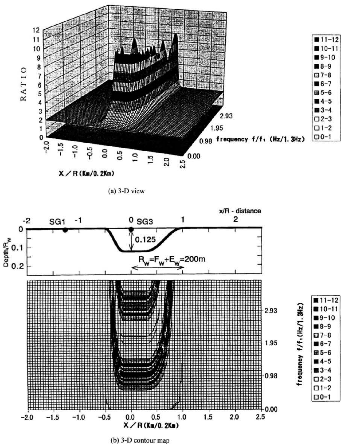
Fig. 2.14 Transfer function of horizontal ground response for SH wave analyzed from 1-D model at TKY
