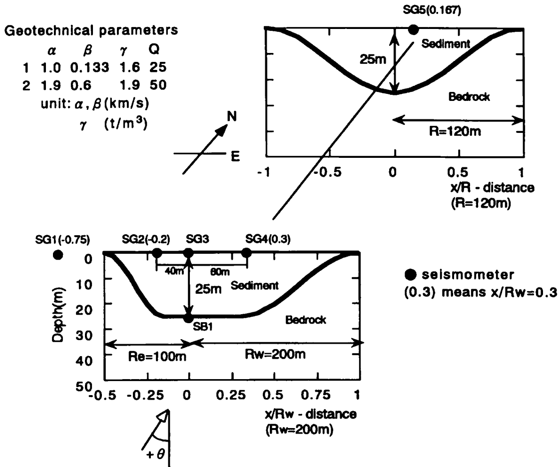
Fig.5.25 Two-dimensional ground model at TKY
