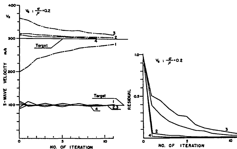
Fig. 2.7 Results of sensitivity of identified S-wave velocities
