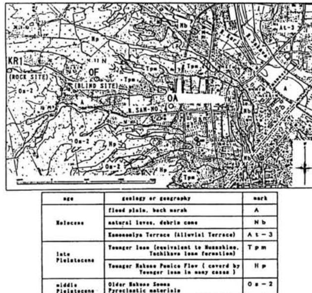
Fig. 5.3 Subsurface geological map at AGK site (KR1, KS1 and KS2 indicate the downhole recording test sites for ESG 10) )
