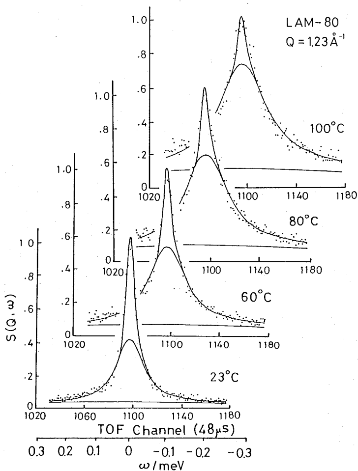
Fig. 11. Dynamic scattering laws S(Q, \omega) of cis-1,4-polybutadiene (PB) in the melt from 23°C to 100°C measured by LAM-80. Solid lines represent the fitting results including elastic and quasielastic scattering components. The almost flat lines represent the very broad quasielastic components observed by LAM-40.
