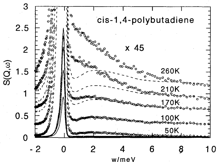
Fig. 6. Dynamic scattering laws S(Q, \omega) of cis-1,4-polybutadiene (PB) measured by LAM-40 below and above the glass transition temperature T_g ( =170\text{K} ). The spectra were obtained by summing up 6 spectra at scattering angle 24^\circ , 40^\circ , 56^\circ , 72^\circ , 88^\circ and 104^\circ and the average Q value is 1.54 \text{ \AA}^{-1} . The spectra are expanded by a factor 45 and shifted by 0.2 for each. Dashed lines are the values expected from the Bose factor, which were calculated based on the spectrum at 50K.
