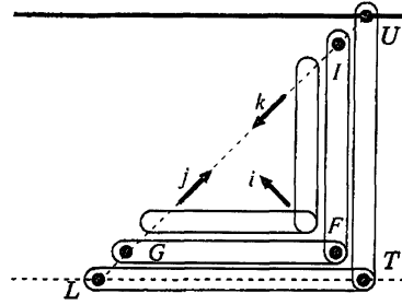
Figure 13: drawing the diamond by the firing squad synchronization technique
