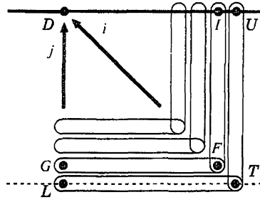
Figure 8: drawing the square by firing squad synchronization
