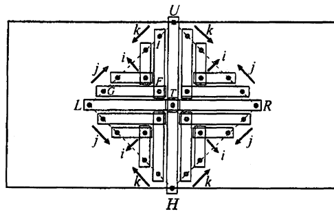
Figure 14: drawing the diamond by the firing squad synchronization technique
