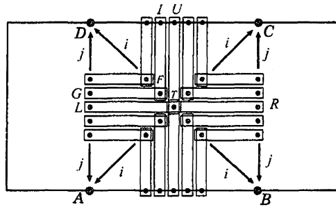
Figure 9: drawing the square by firing squad synchronization in four area
