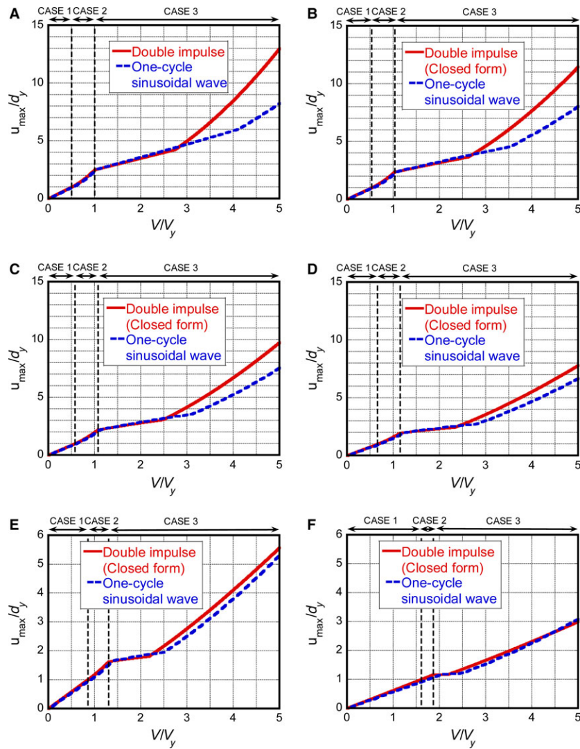
Figure 13. Comparison of the maximum elastic-plastic deformation u_{\max}/d_y of the model with viscous damping under critical double impulse (quadratic function approximation) with that under the equivalent one-cycle sine wave: (A) h = 0 , 13 (B) h = 0.02 , (C) h = 0.05 , (D) h = 0.1 , (E) h = 0.2 , (F) h = 0.5
