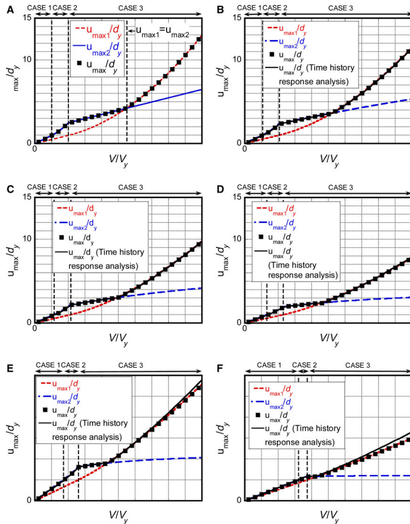
Figure 9. Comparison of the maximum elastic-plastic deformation u_{\max}/d_y of the model with viscous damping under the critical double impulse using the quadratic approximation of the damping force-deformation relation with that obtained by time-history response analysis: (A) h = 0^{13} , (B) h = 0.02 , (C) h = 0.05 , (D) h = 0.1 , (E) h = 0.2 , (F) h = 0.5
