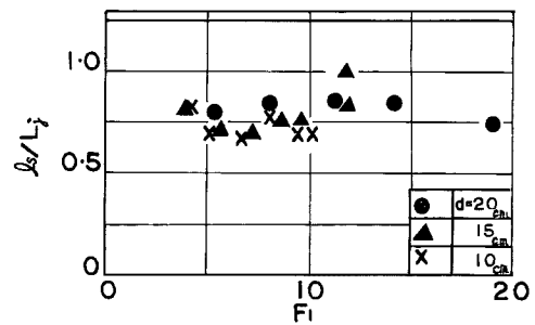
Fig. 6. Length of roller in terms of L_j .
