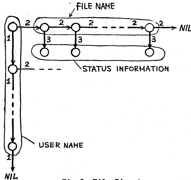
Fig.2. File Directory
