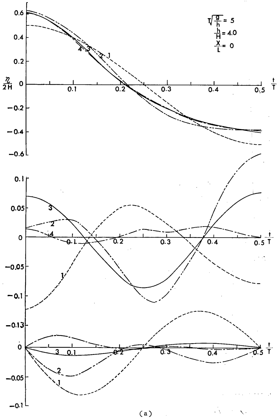
Fig. 1 Variations of free surface boundary condition errors for validity of finite amplitude standing wave theory, defined by \varepsilon_1 and \varepsilon_2 , and wave profiles.
