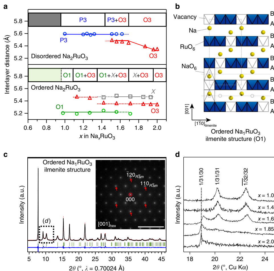
Figure 4 | Structural changes of disordered and ordered Na 2 RuO 3 during charge. (a) Interlayer distance of the different phases involved on desodiation as a function of x in disordered and ordered Na x RuO 3 . (b) Crystal structure of ilmenite-type Na 1 RuO 3 . All Na ions displace cooperatively towards Na vacancies in the honeycomb planes. (c) Observed and calculated (Rietveld method) synchrotron X-ray diffraction patterns for ordered Na 1 RuO 3 . Red crosses: experimental, black line: calculated, blue line: difference and green bars: Bragg positions. The inset shows the selected area electron diffraction (SAED) pattern for ilmenite-type Na 1 RuO 3 . Scale bar, 10 nm -1 . (d) Ex situ XRD patterns showing the evolution of the superstructure peaks for ordered Na x RuO 3 on charge.
