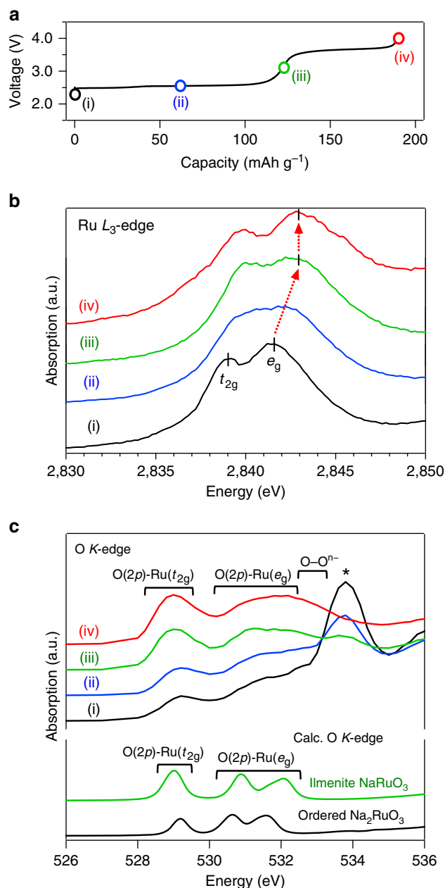
Figure 6 | Electronic structure changes of ordered Na 2 RuO 3 upon charge. (a) States of charge of the samples for X-ray absorption spectroscopy. (b) Ruthenium L 3 -edge and (c) oxygen K-edge X-ray absorption spectra for various O-Na x RuO 3 compositions: (i) x=2.0 (black), (ii) x=1.5 (blue), (iii) x=1.0 (green) and (iv) x=0.62 (red). The asterisked peak corresponds to O 2p-Na 3p. The calculated oxygen K-edge spectra for ordered Na 2 RuO 3 (black) and ilmenite-type NaRuO 3 (green) are also shown.
