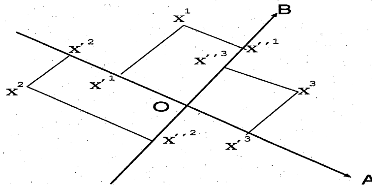
Figure 4 : Shapley's construction of orderings
