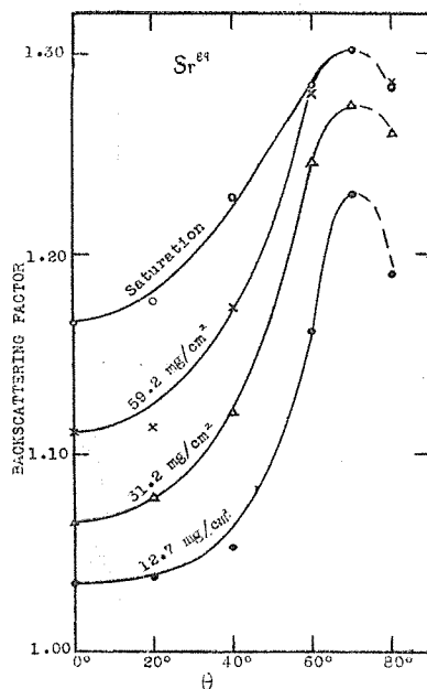
Fig. 6. Angular distribution of the backscattering factor for \beta -rays of \text{Sr}^{90} with aluminium backings.
