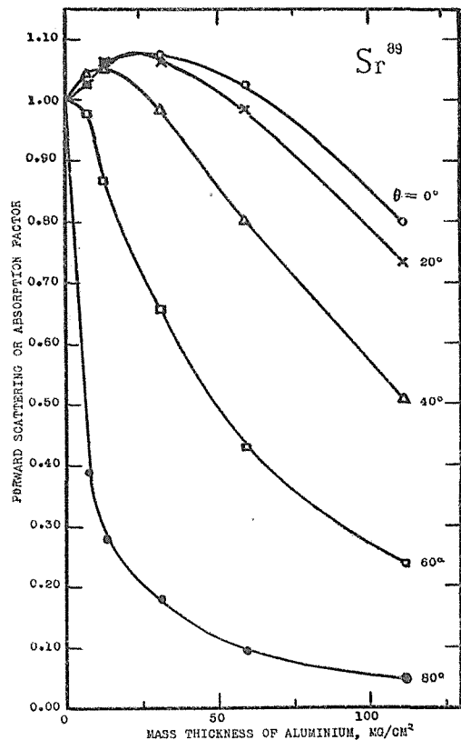
Fig. 15. The forward scattering or absorption for \beta -rays of \text{Sr}^{89} as a function of thickness of the aluminium scatterer.
