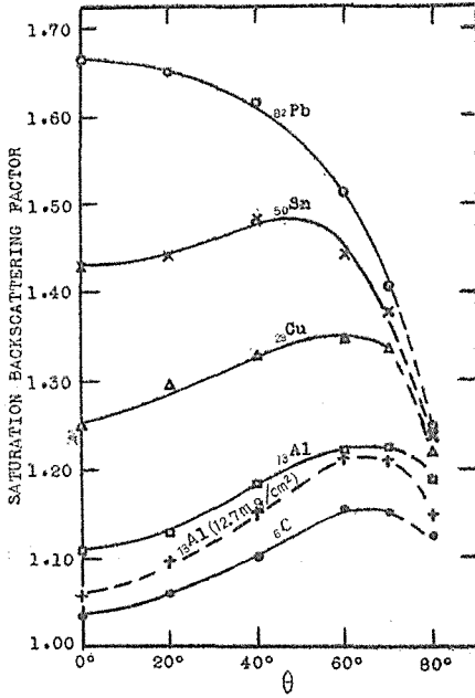
Fig. 10. Angular distribution of the saturation backscattering factor for \beta -rays of \text{I}^{131} with several backings.
