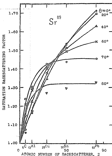
Fig. 9. Saturation backscattering factor for \beta -rays of \text{Sr}^{89} as a function of atomic number of backscatterer.
