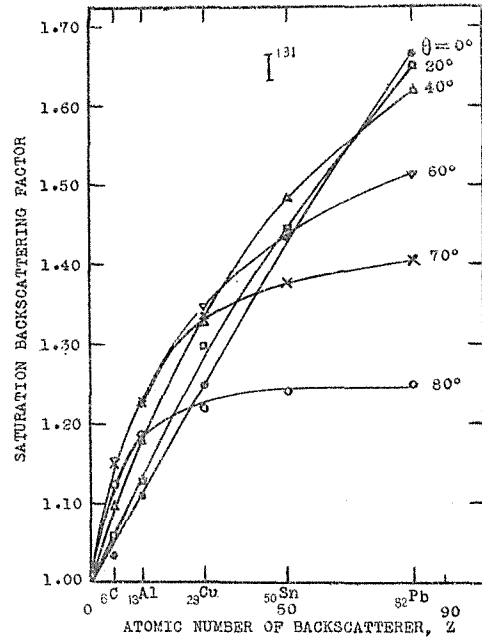
Fig. 11. Saturation backscattering factor for \beta -rays of \text{I}^{131} as a function of atomic number of backscatterer
