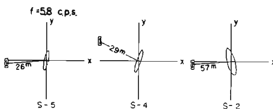
Fig. 12 Loci of oscillation at S-2, S-4, and S-5 generated by the oscillator situated in drift.
