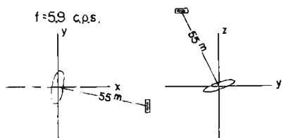
Fig. 11 Loci of oscillation at S-3 generated by the oscillator situated at the ground surface. The oscillation were applied to normal to the direction of stratification.
