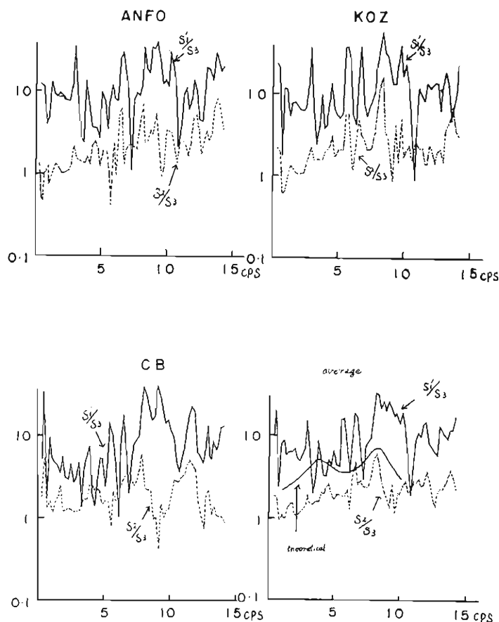
Fig. 20 Ratios of amplitude spectra : S_1/S_s , S_2/S_s
