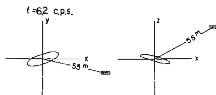
Fig. 10 Loci of oscillation at S-3 generated by the oscillator situated at the ground surface. The oscillations were applied to parallel to the direction of stratification.
