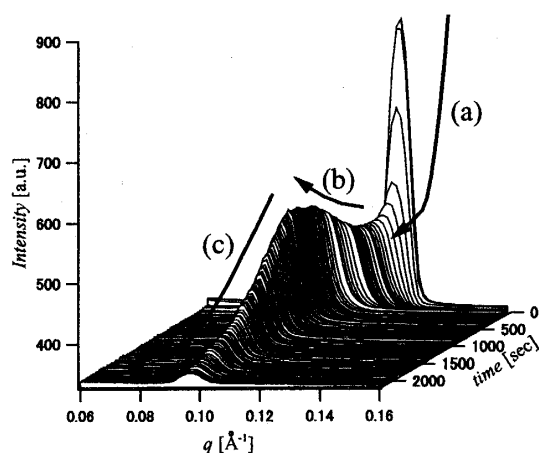
Figure 1: Time-resolved SAXS profile for hydration process of multi-stacked phospholipid bilayers. The Bragg peaks correspond to the regular stacking of bilayers. There are three stages (a), (b) and (c).
