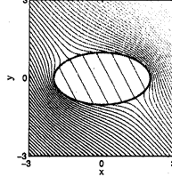
Figure 2.3: Field is uniform inside the elliptic inclusions.
