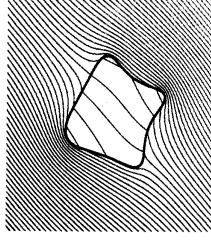
Figure 2.1: An inclusion embedded in the free space with a uniform field
