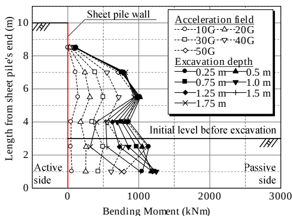
(a) Bending moment at wall (Sand layer)
