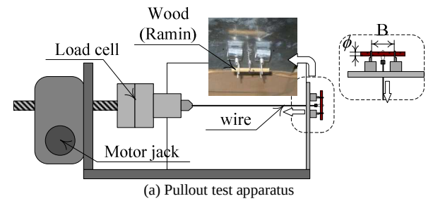
(a) Pullout test apparatus
