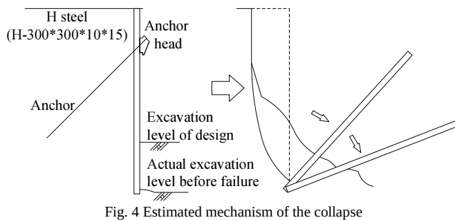
Fig. 4 Estimated mechanism of the collapse
