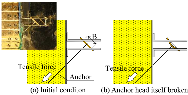
Fig. 8 Physical modelling of broken anchor head
