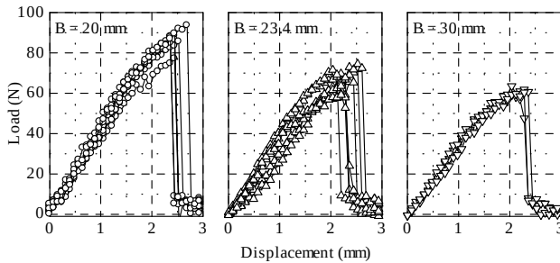
(b) Load – displacement curves in pullout test Fig. 9 pullout test
