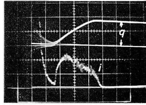
(b) q (0.43 nC/div.), i (2 mA/div.) (2 \mu s/div.)
