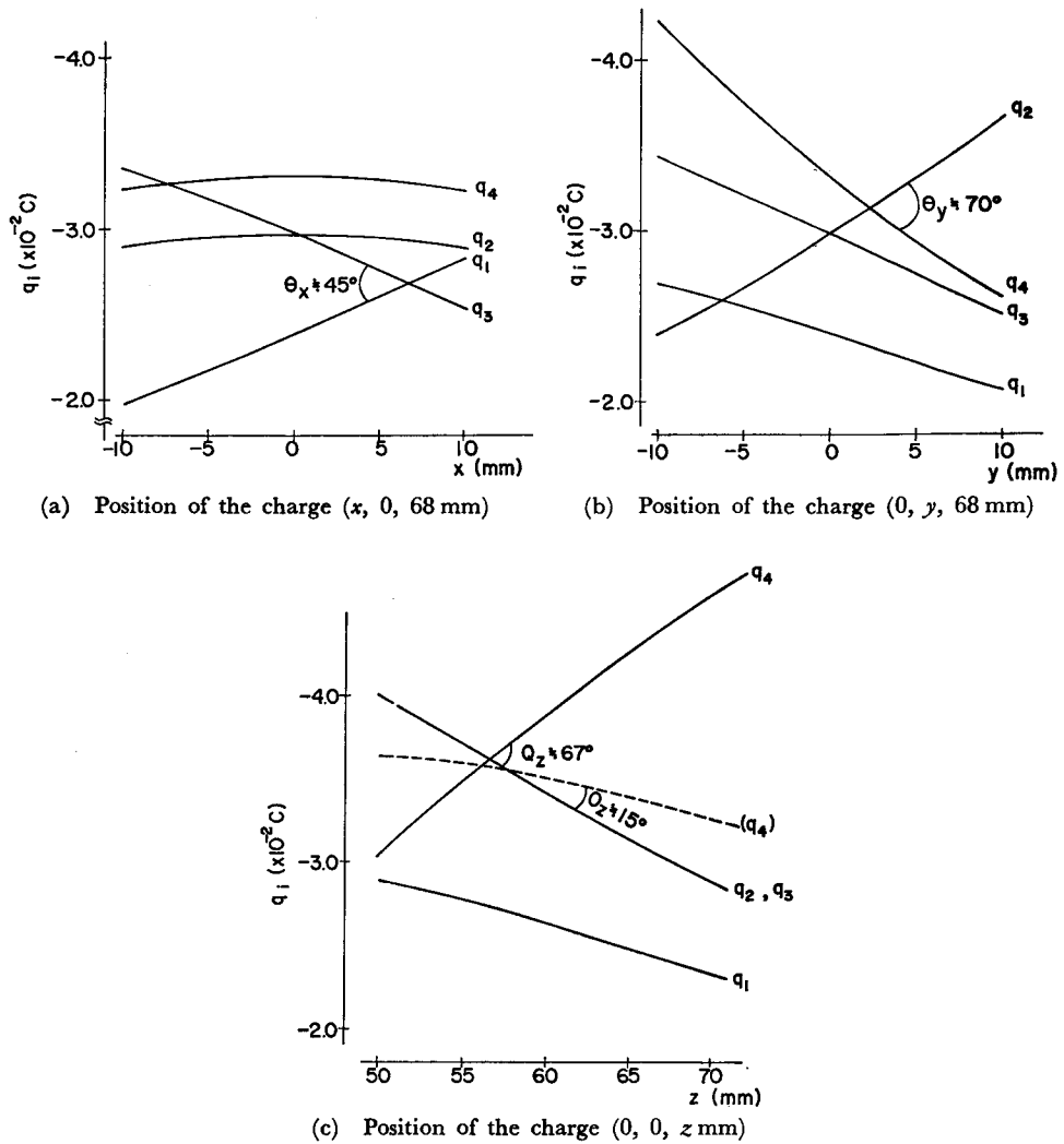
Fig. 7. Variation of q_i with the position of a point charge Q_s ( =1 C).
