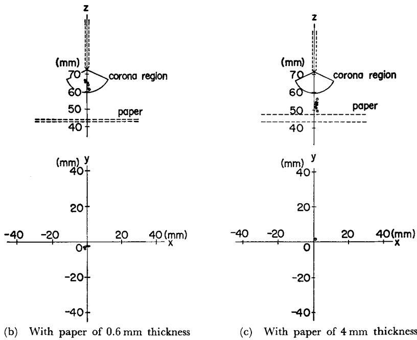
Fig. 5. Position of the corona charge evaluated by using Eq. (4) (Applied voltage; +50 kV).
