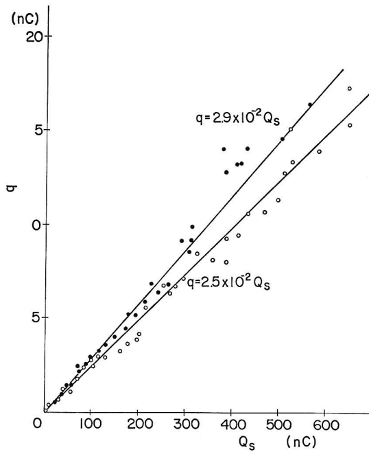
Fig. 4. Relations between amount of space charge Q_s and the induced charge on the probe ( q=100 mm, \bullet ; positive corona, \circ ; negative corona).
