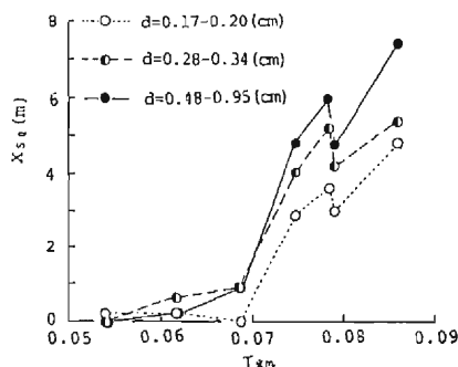
Fig. 13. Relation between the median travel distance and the tractive force (Exp. D, T=20 min).
