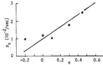
Fig. 4. Relation between the degree of exposure and pick up rate for uniform material ( \tau_{*0}=0.08 ).
