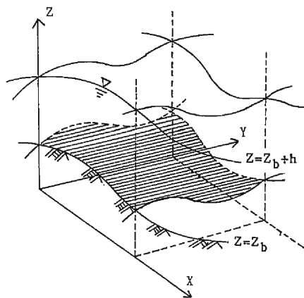
Fig. 1. Definition sketch of coordinates system.
