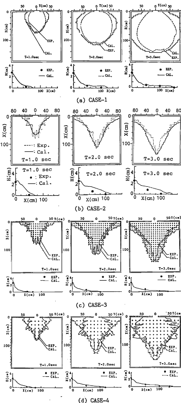
Fig. 7. Comparison between experimental results with calculated ones concerned with shapes of flooding and water surface profiles along the flow axis.
