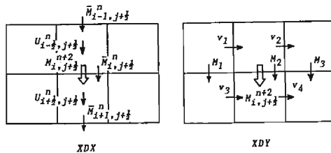
Fig. 3. Arrangement of u_0 , v_0 and M in calculation of XDX and XDY .
