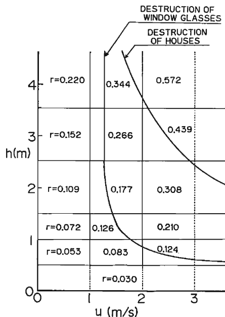
Fig. 31. Modified relationship between velocity and water depth for the damage factor.
