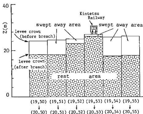
Fig. 24. Example of the scales and elevations for brach point P1 meshes in calculation before and after the bank breach.
