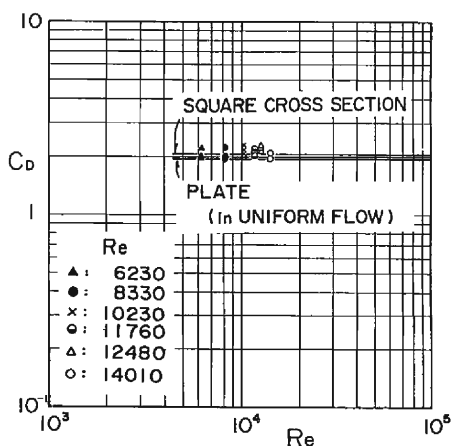
Fig. 12. Relationship between drag coefficient and Reynolds number.
