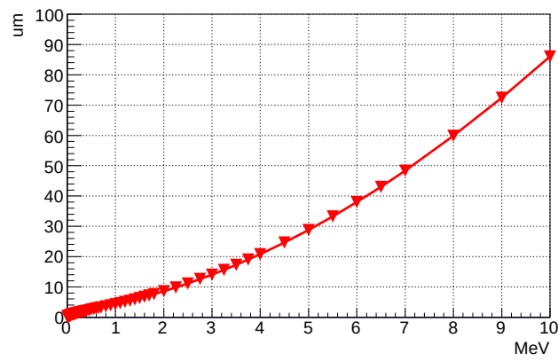
Figure 6.1.14: The calculated range of alpha particles in polyimide by SRIM. The highest energy of alpha particle of U-chain and Th-chain is 8.785 MeV, and the thickness of the insulator (polyimide) is 100\text{ }\mu\text{m} . Thus, the alpha particles from the back side of the insulator (polyimide) do not come into to the detectable reagon.
