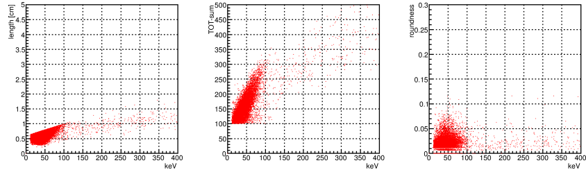
Figure 5.1.3: Energy dependence of the length (left), the TOT-sum (center), and the roundness (right). The events are cut by fiducial-cut, length-cut and TOT-sum-cut. These events correspond to the blue line in Figure 5.1.5.
