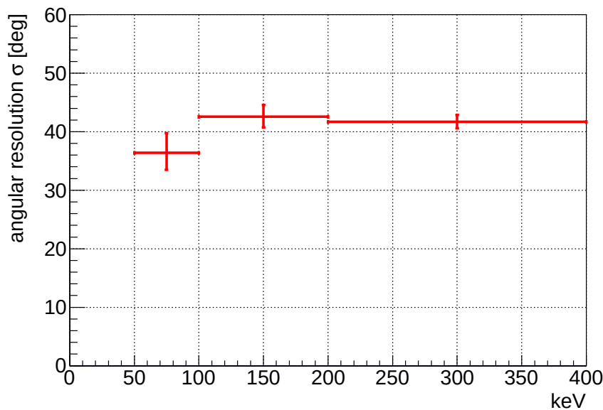
Figure 4.4.21: Obtained angular resolution for each energy.
