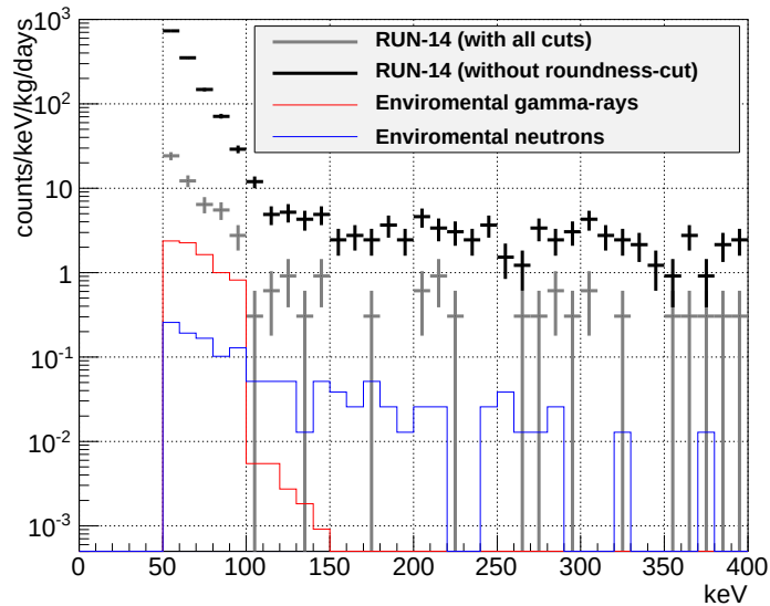
Figure 6.2.7: Energy spectrum of the measurement and estimated environmental backgrounds. Gray line shows the measured spectrum with all cuts. Black line shows the measured spectrum with all but the roundness-cut. Red line shows the estimated spectrum by environmental gamma-rays. Blue line shows the estimated spectrum by environmental neutrons.
