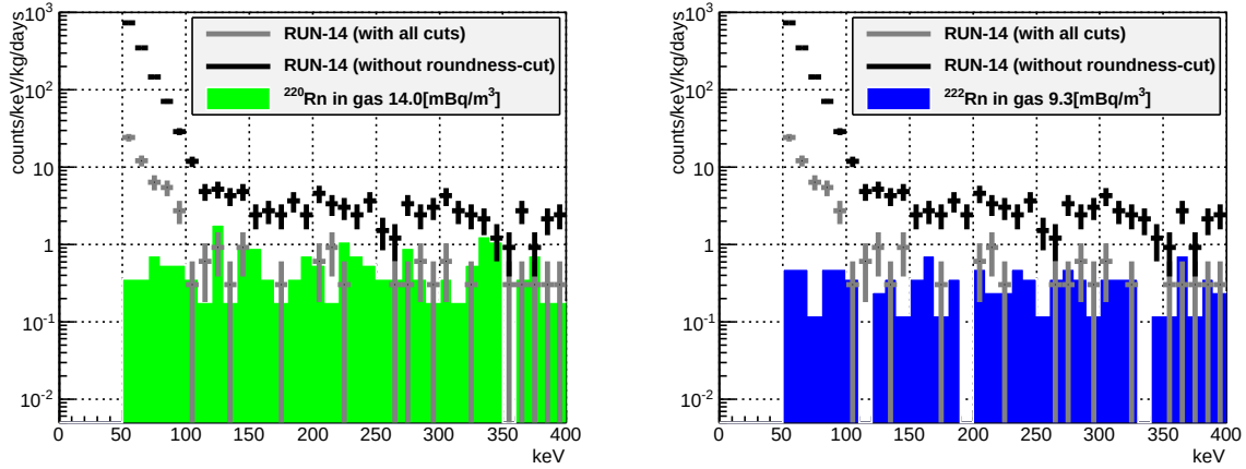
Figure 6.2.8: Estimated energy spectra of background from ^{220}\text{Rn} (left) and ^{222}\text{Rn} (right) in the detection volume. Gray line shows the measured spectrum in RUN14 with all cuts. Black line shows the measured spectrum in RUN14 with all but the roundness-cut.
