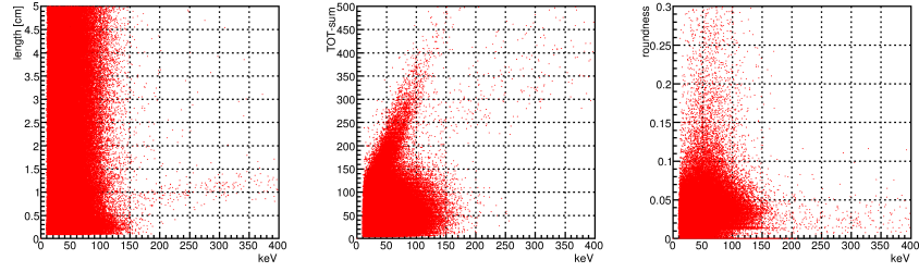
Figure 5.1.1: Energy dependence of the length (left), the TOT-sum (center), and the roundness (right). The events are cut by only fiducial-cut. These events correspond to the black line in Figure 5.1.5.
