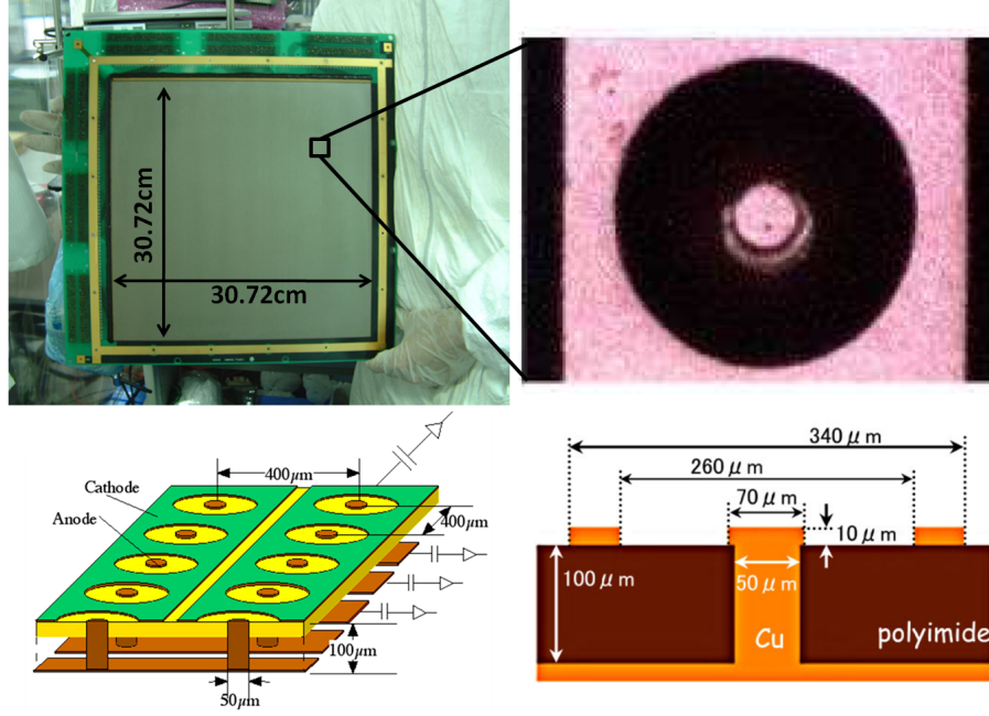
Figure 4.1.4: The photograph of \mu -PIC (left top) and the schematic view of \mu -PIC (left bottom). Upper right figure shows the enlarged photograph by microscope. Bottom right figure shows the cross-section view of the \mu -PIC structure.
