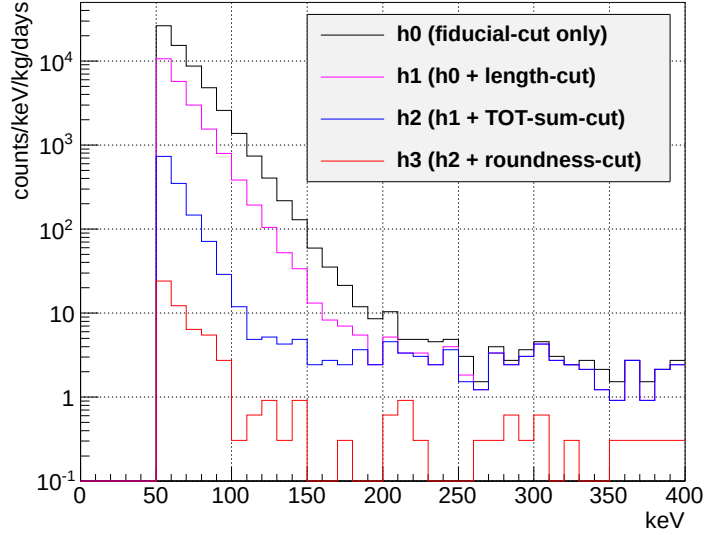
Figure 5.1.5: Obtained energy spectra in Kamioka RUN-14. Black line is the spectrum with only the fiducial-cut. As show in the legend, pink, blue, and red histograms are the energy spectra at each cut-step described in Section 4.4.3, and correspond to the events shown in Figure 5.1.1-5.1.4.
