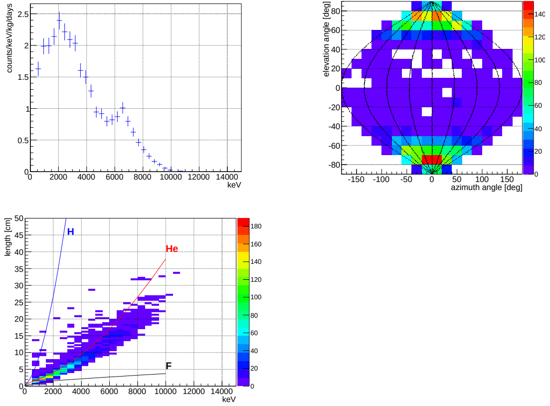
Figure 6.0.3: Obtained energy spectrum (top-left), energy-length distribution (bottom), and direction distribution (top-right) of RUN14 in the range of 500 – 15000 keV. Only fiducial-cut is applied.
