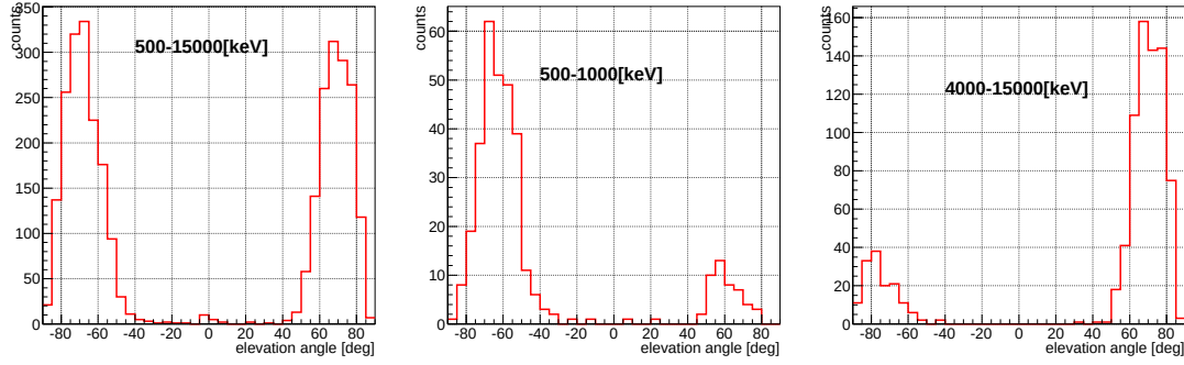
Figure 6.1.9: Measured elevation angle distribution of continuous high energy background. Left, center and right figure shows the distributions correspond to the energy region of 0.5 - 15 MeV, 0.5 - 1 MeV, and 4 - 15 MeV, respectively.
