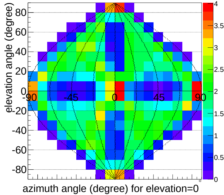
Figure 4.4.22: Direction-dependent efficiency in the 50 – 100 keV range measured with DAQ-mode5 and the self trigger. The vertical axis is the elevation angle and the horizontal axis is the azimuth angle. Color scale is normalized counts by the mean value.
