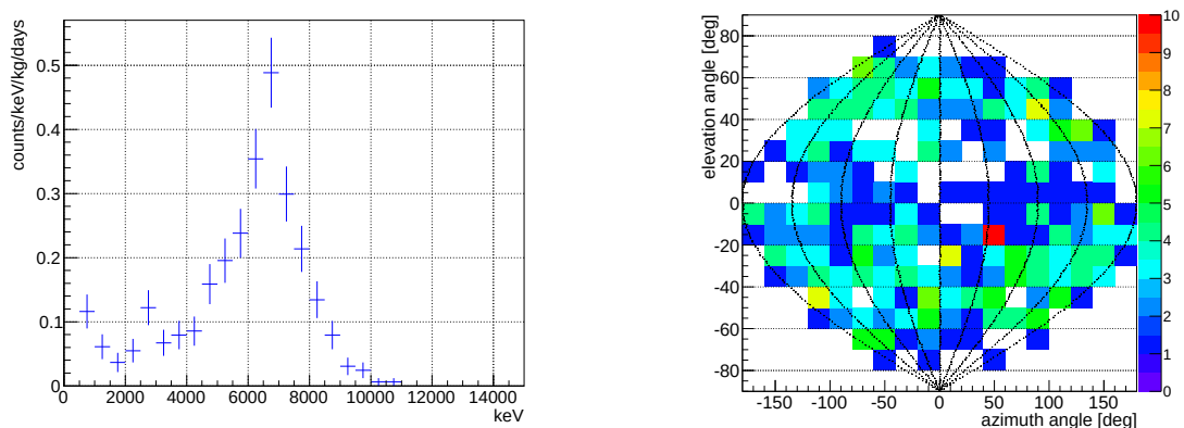
Figure 6.1.4: Obtained energy spectrum (left) and direction distribution (right) above the red dotted line in Figure 6.1.3.
