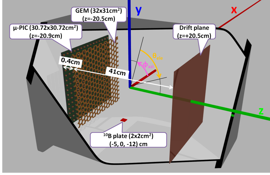
Figure 4.1.2: The schematic image of the \mu -TPC named NEWAGE-0.3b'. The coordinate system, with its origin at the center of the detection volume, is also shown. Red, blue and green lines shows the x , y and z axis. A glass plate with a thin layer of ^{10}\text{B} is set at (-5, 0, -12) cm for the energy calibration.
