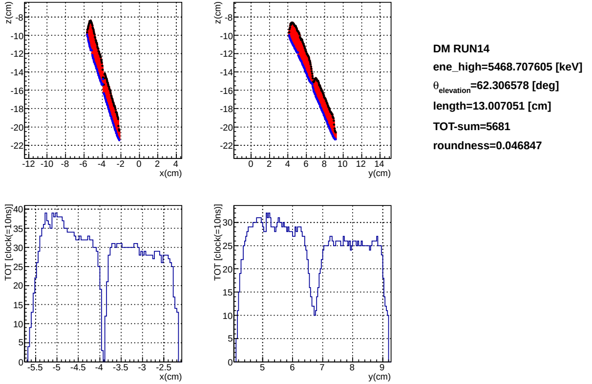
Figure 6.1.8: Example of a high energy (5470 keV) track and TOT distribution. Left-top and right-top figure shows x-z and y-z projected track, respectively. Left-bottom and right-bottom figure shows TOT distribution for x-strips and y-strips, respectively. The gap around x = -4 cm is due to the segmentation gap of GEM and correspond to the gap around y = 6.7 cm.
