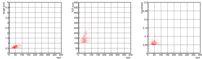
Figure 5.1.4: Energy dependence of the length (left), the TOT-sum (center), and the roundness (right). The events are final sample with the fiducial-cut, length-cut, TOT-sum-cut and roundness-cut. These events correspond to the red line in Figure 5.1.5.
