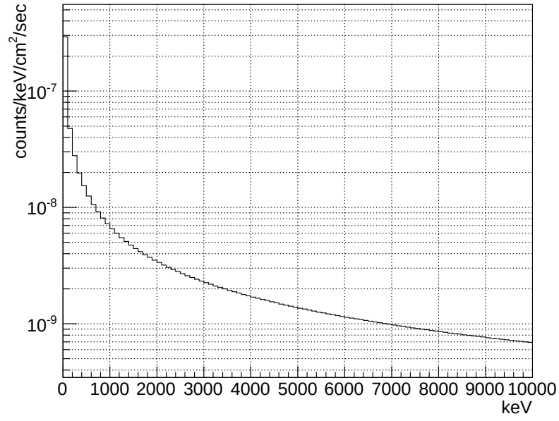
Figure 6.2.3: Estimated flux of environmental fast neutrons in Kamioka mine.
