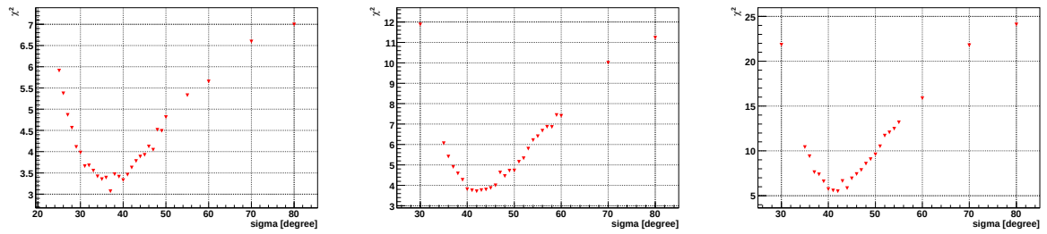
Figure 4.4.20: \chi^2 values obtained between measured and simulated |\cos \theta| distributions as a function of angular resolution. The energy range of left, center, and right figures are 50 – 100 keV, 100 – 200 keV, and 200 – 400 keV, respectively.
