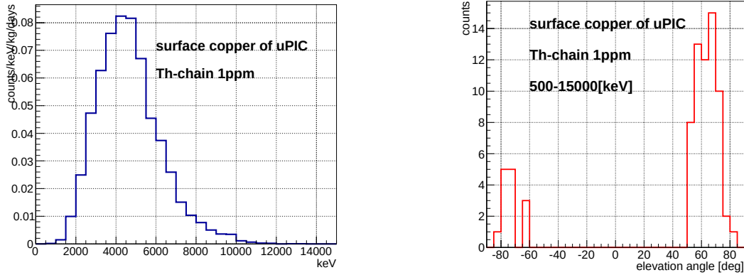
Figure 6.1.11: The simulation result of the energy spectrum (left) and elevation angle distribution in energy of 500 - 15000\ \text{keV} (right) by assuming 1 ppm contamination of Th-chain in the surface copper of the \mu -PIC.
