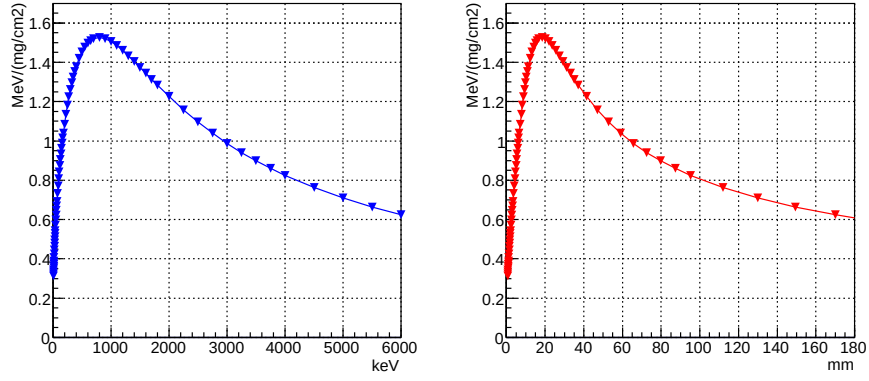
Figure 6.1.7: Energy deposition of \alpha particles as a function of energy (left) and length (right) in the 0.1 atm CF 4 gas.
