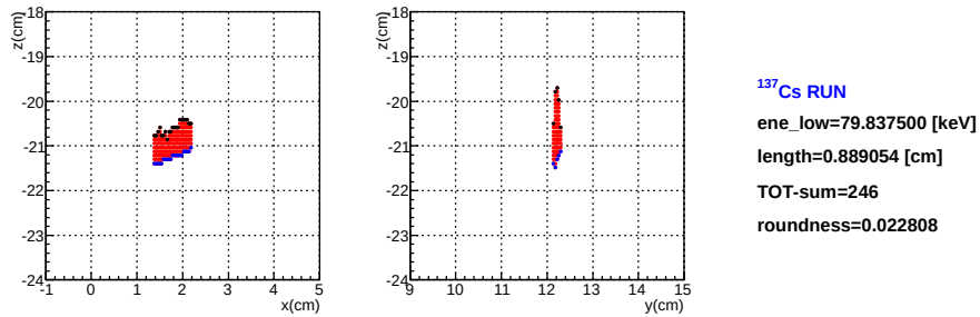
Figure 4.4.9: Track sample measured with ^{137}\text{Cs} , cut by roundness-cut.
