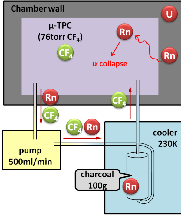
Figure 4.1.5: The schematic image of the gas circulation system for lowering radon backgrounds and keeping the gas quality.
