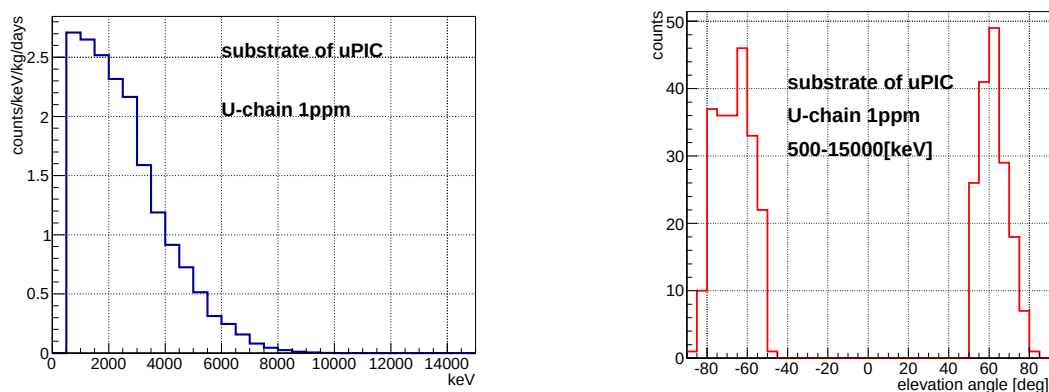
Figure 6.1.13: The simulation result of the energy spectrum (left) and elevation angle distribution in an energy range of 500 – 15000 keV (right) by assuming 1 ppm contamination of U-chain in the substrate of the \mu -PIC.
