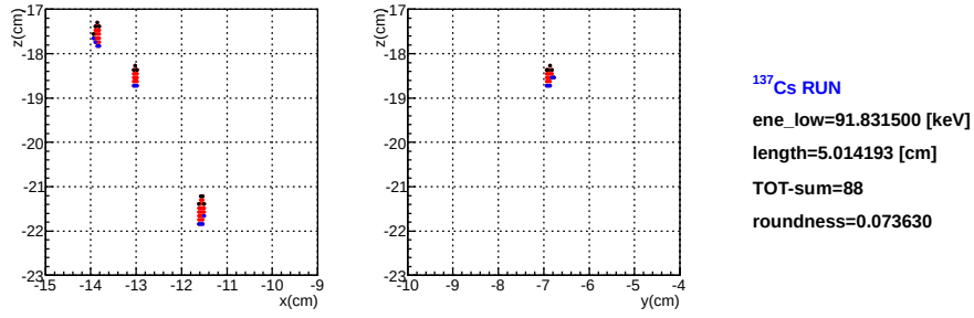
Figure 4.4.7: Track sample measured with ^{137}\text{Cs} , cut by length-cut.
