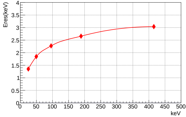
Figure 4.4.5: Estimated energy resolution ( \sigma keV) due to the electric noise. The energy dependence is due to the width of waveforms.
