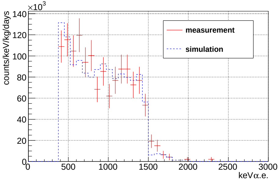
Figure 4.4.2: The result of an energy calibration using \alpha particles from ^{10}\text{B}(\text{n}, \alpha)^7\text{Li} . Blue line is simulated energy spectrum and red points are measured one.
