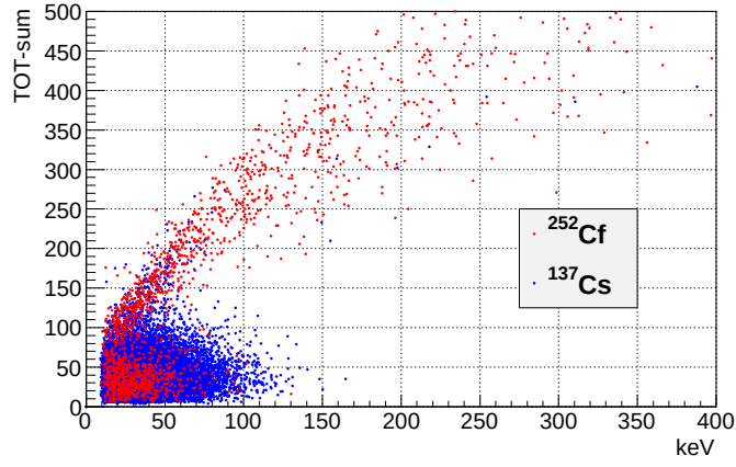
Figure 4.4.11: Energy dependence of the TOT-sum after the length-cut. Red and blue points are same to above figure.
