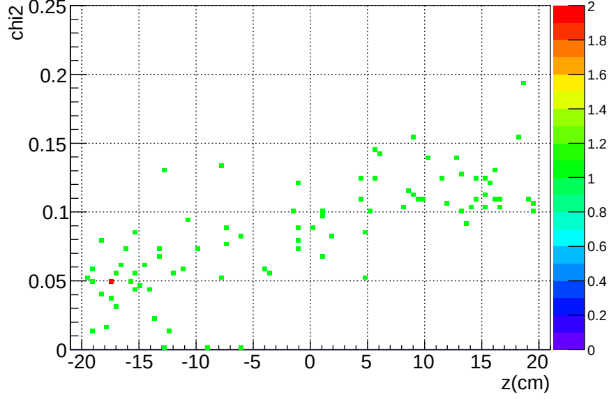
Figure 4.4.13: The measured roundness as a function of drift length.
