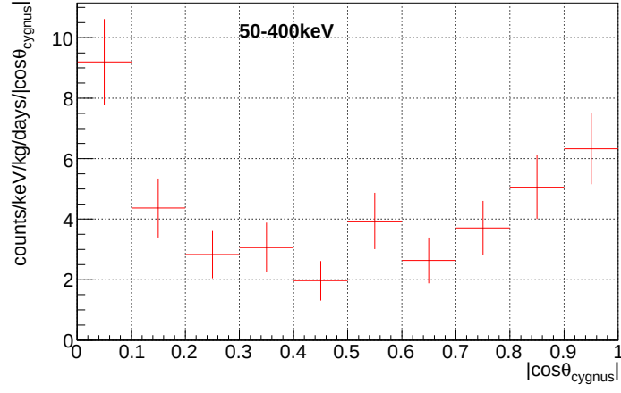
Figure 5.1.8: Obtained |\cos \theta_{\text{cygnus}}| distribution of RUN-14 in the energy range of 50 – 400 keV
