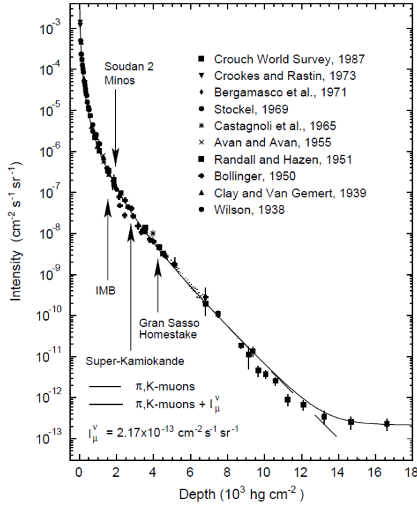
Figure 6.2.2: Cosmic-ray muon flux as a function of depth in 10^3 \text{ hg/cm}^2 equivalent to km w.e.[81].
