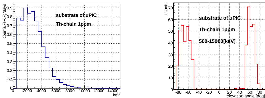
Figure 6.1.12: The simulation result of the energy spectrum (left) and elevation angle distribution in an energy range of 0.5 – 15 MeV (right) by assuming 1 ppm contamination of Th-chain in the substrate of the \mu -PIC.
