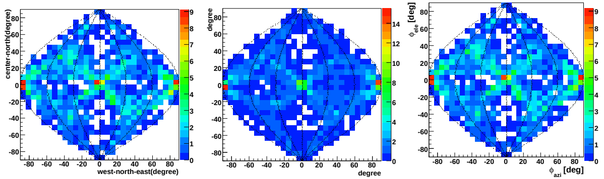
Figure 4.4.17: Direction-dependent efficiency, or the response to isotropic irradiation, for angular resolution measurement range measured with DAQ-mode1 and external-trigger mode. The energy range of left, center, and right figures are 50 – 100 keV, 100 – 200 keV, and 200 – 400 keV, The vertical axis is the elevation angle and the horizontal axis is the azimuth angle. Color scale is counts normalized by the mean value.
