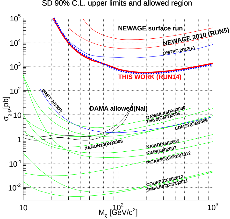
Figure 5.2.2: Limits of SD cross section, \sigma_{\chi-p}^{\text{SD}} , as a function of mass of WIMP mass M_\chi . Red thick solid line is the result of a directional method in this work. Blue thick dotted line is a result obtained with the conventional method for reference. Red thin lines labeled "NEWAGE surface run" and "NEWAGE 2010 (RUN5)" are previous results measured at surface and Kamioka, respectively[83]. Allowed region (DAMA[39]) and upper limits of other experiments are shown for comparison. Green lines are limits set by liquid or solid detectors, blue lines are the limits set by gas detectors with conventional analysis.
