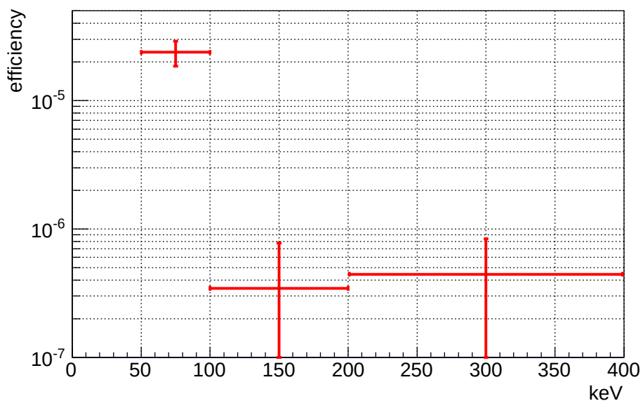
Figure 4.4.15: The detection efficiency of the electron event, or gamma-ray rejection power.
