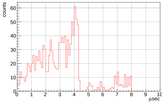
Figure 4.4.1: Drift time distribution of nuclear recoils in a drift velocity measurement.
