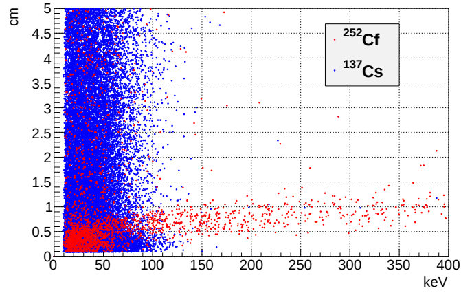
Figure 4.4.10: Energy dependence of the track-length. Red and blue points are measured with ^{252}\text{Cf} and ^{137}\text{Cs} , respectively.
