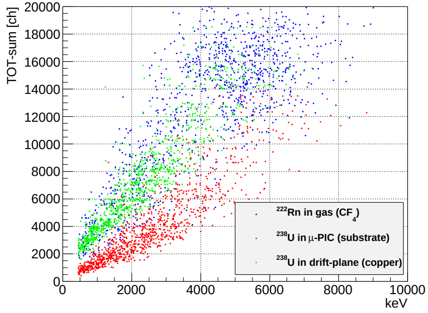
Figure 6.1.2: Simulated TOT-sum as a function of energy. Color indicates the origins of the sources.
