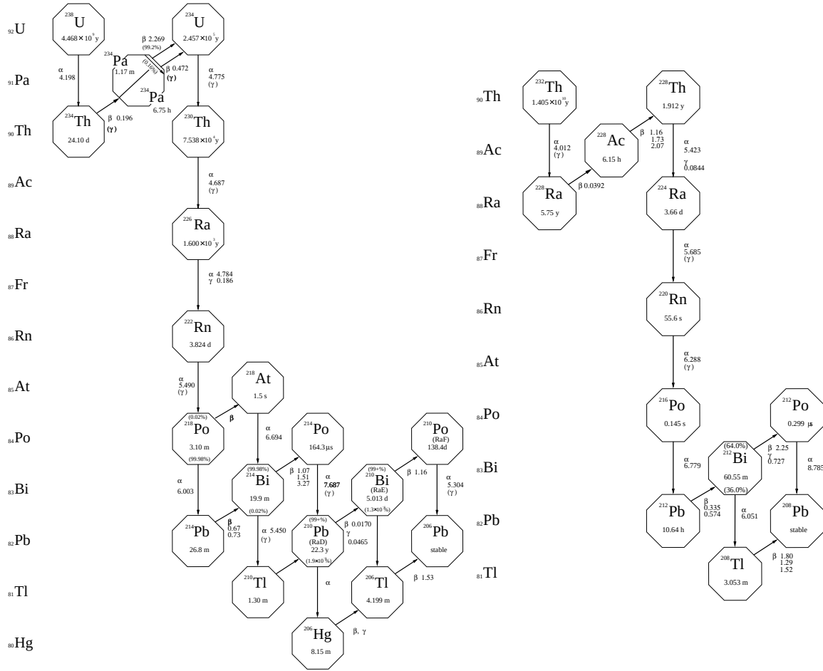
Figure 6.0.1: Decay chain of ^{232}\text{Th} and ^{238}\text{U} .
