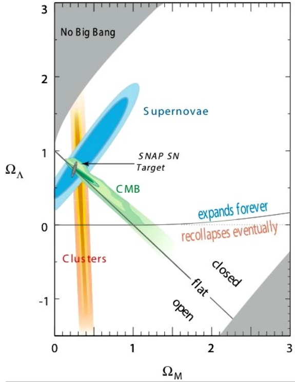
Figure 1.1.4: Allowed regions of cosmological parameters ( \Omega_\Lambda , \Omega_m ) by observations of IaSN ("Supernovae" in figure)[3], CMB[1], and BAO ("clusters" in figure) [2]. A flat universe with (\Omega_\Lambda, \Omega_m) \simeq (0.7, 0.3) is favored by each three observations.
