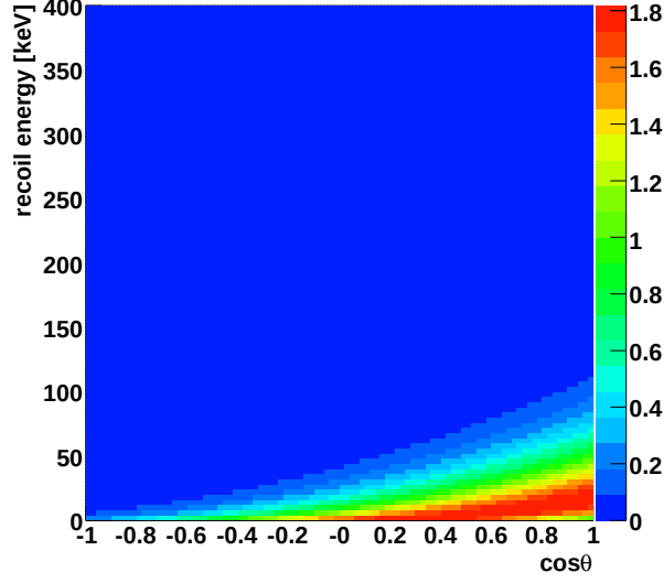
Figure 2.4.4: The expected angle-energy distribution, where the target is ^{19}\text{F} for the SD interaction, M_{\text{D}} = 100 \text{ GeV} , \sigma_{\chi\text{-p}}^{\text{SD}} = 1 \text{ pb} , \theta is the angle formed by the WIMP-wind direction and recoil nuclei direction. The color bar represent the event rate with an unit of [\text{count}/\text{keV}/\text{kg}/\text{days}/\cos\theta] .
