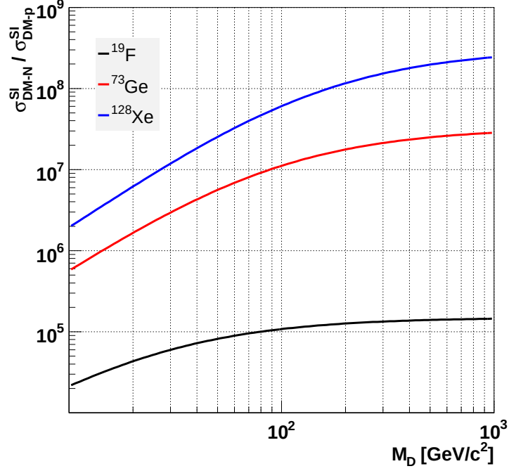
Figure 2.2.2: SI cross sections normalized by neutralino-proton SI cross section, \sigma_{\chi-N}^{\text{SI}}/\sigma_{\chi-p}^{\text{SI}} as a function of neutralino mass. Black, red and blue line shows target difference as ^{19}\text{F} , ^{73}\text{Ge} and ^{128}\text{Xe} .
