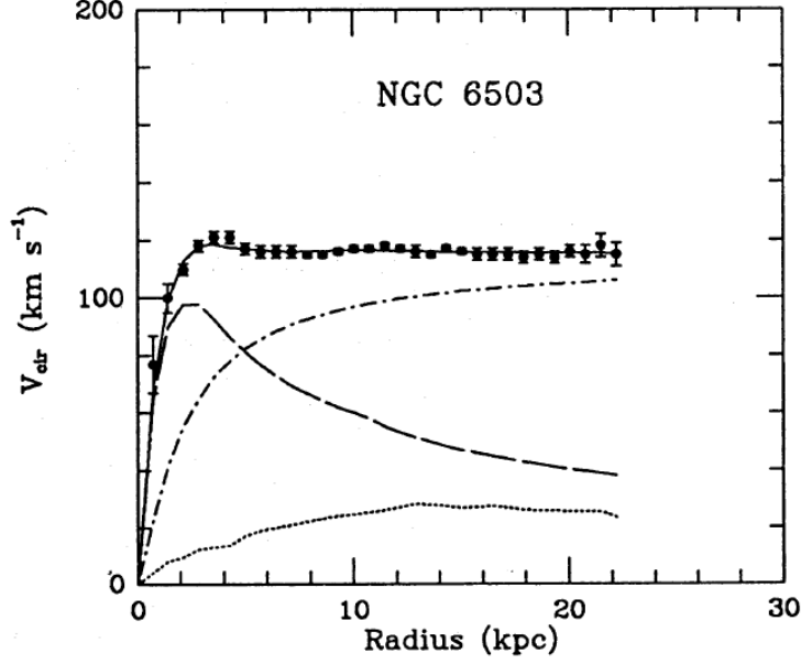
Figure 1.1.1: The rotation curve of NGC6503 spiral galaxy. The black points are measured velocity by Doppler shift of 21 cm line[5]. The dashed line and dotted line are the contribution to the rotation velocity from the observed disk and gas, respectively. The dashed-dotted line is the contribution from the invisible mass at the galaxy halo. The solid line is a sum of them.
