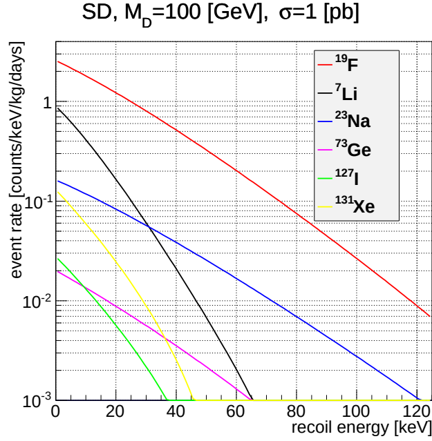
Figure 2.4.2: The expected energy spectrum dR/dE_R of various targets for the SD-interacting neutralino with a mass of M_D = 100 \text{ GeV}/c^2 and \sigma_{\chi-p}^{\text{SD}} = 1 \text{ pb} .
