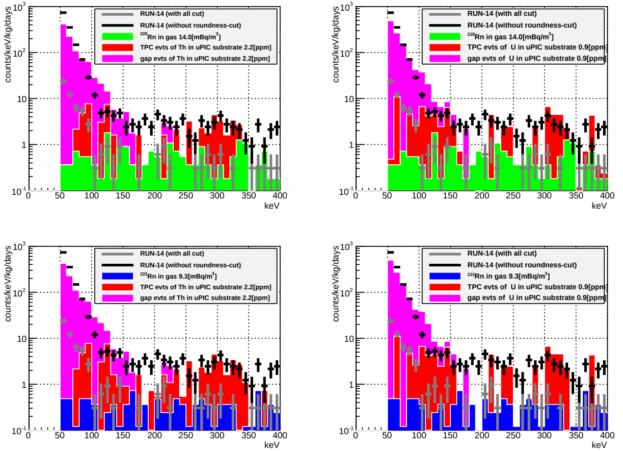
Figure 6.2.13: The estimated energy spectrum due to the radons and the radioactive impurities included in the substrate of the \mu -PIC. Each figure differs in the type of radon and U/Th-chain in substrate.
