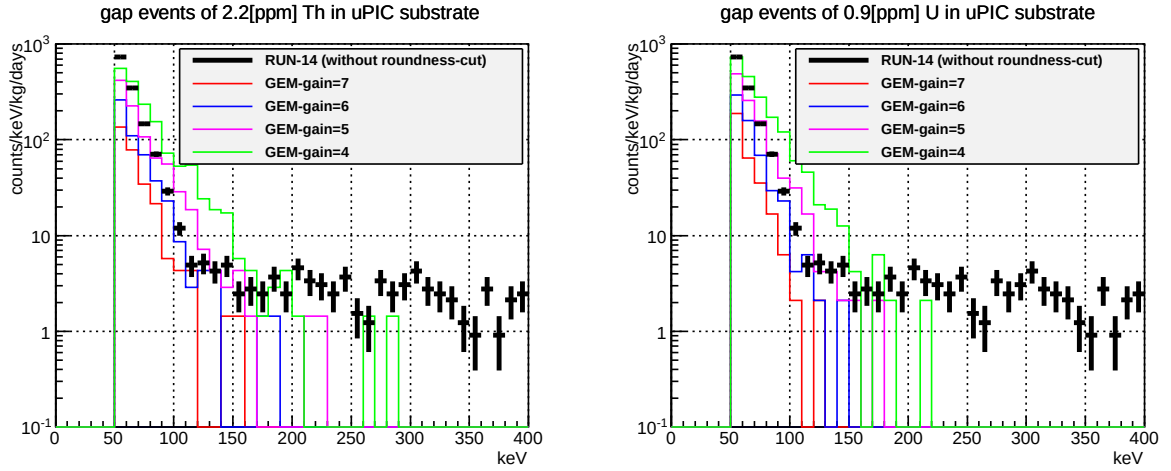
Figure 6.2.11: The estimated energy spectra of the events that \alpha particles from radioactive impurities included in the substrate of the \mu -PIC stopping in the gap region (C' in Figure 6.2.1). Left and right figure show the results by assuming 2.2 ppm of Th-chain and 0.9 ppm of U-chain, respectively. The evaluated concentration amounts of each isotope-chain discussed in Section 6.1.2 is used. We assumed several typical gain of GEM because we cannot measure the accurate gain of GEM itself. We put the measured spectrum of RUN14 without the roundness-cut because the events from substrate is basically cut by the effect of z-fiducilization of roundness-cut.
