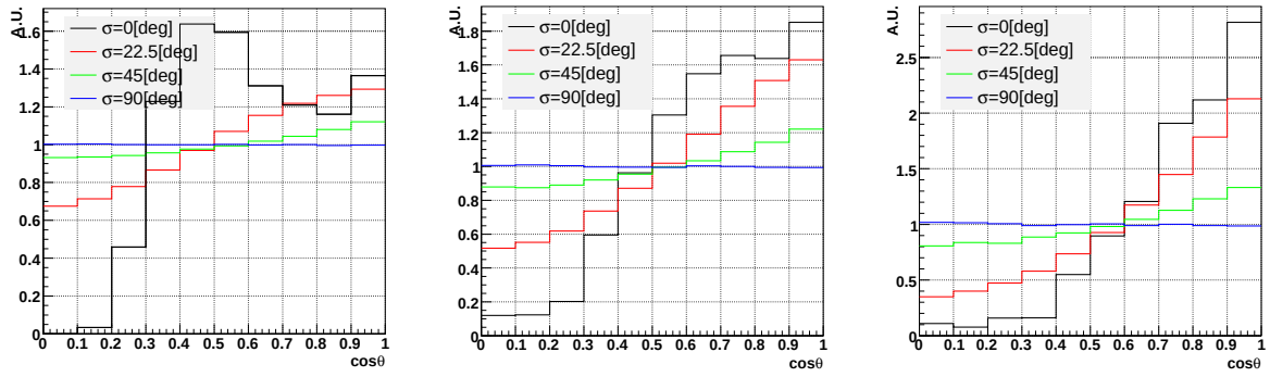
Figure 4.4.19: Simulated |\cos \theta| distributions assuming angular resolutions of 0^\circ (black), 22.5^\circ (red), 45^\circ (green), 90^\circ (blue). The energy range of left, center, and right figures are 50 – 100 keV, 100 – 200 keV, and 200 – 400 keV, respectively.
