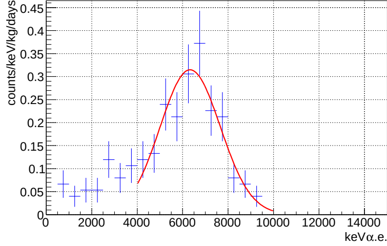
Figure 4.4.3: The measured energy spectrum of \alpha particles due to the radon progeny (blue histogram). Red line is the fitted line in case of ^{220}\text{Rn} .
