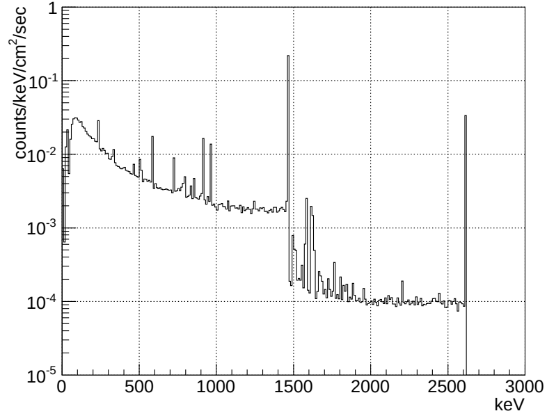
Figure 6.2.5: Estimated flux of environmental gamma-rays from measurement of a CsI(Tl) scintillator[83]. The gamma-rays from ^{40}\text{K} , U-chain, and Th-chain in the rock are taken into account.
