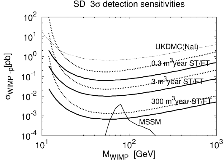
Figure 4.0.1: Sensitivity goals of the NEWAGE project. Thick and dotted lines show expected 3\sigma asymmetry detection sensitivities by the ST(semi-tracking) and FT(full-tracking) modes, respectively. Details are described in [73]. An experimental result of NAIAD (thin dashed dotted line labeled UKDMC) and MSSM predictions (thin line labeled MSSM) are also shown [41, 74].
