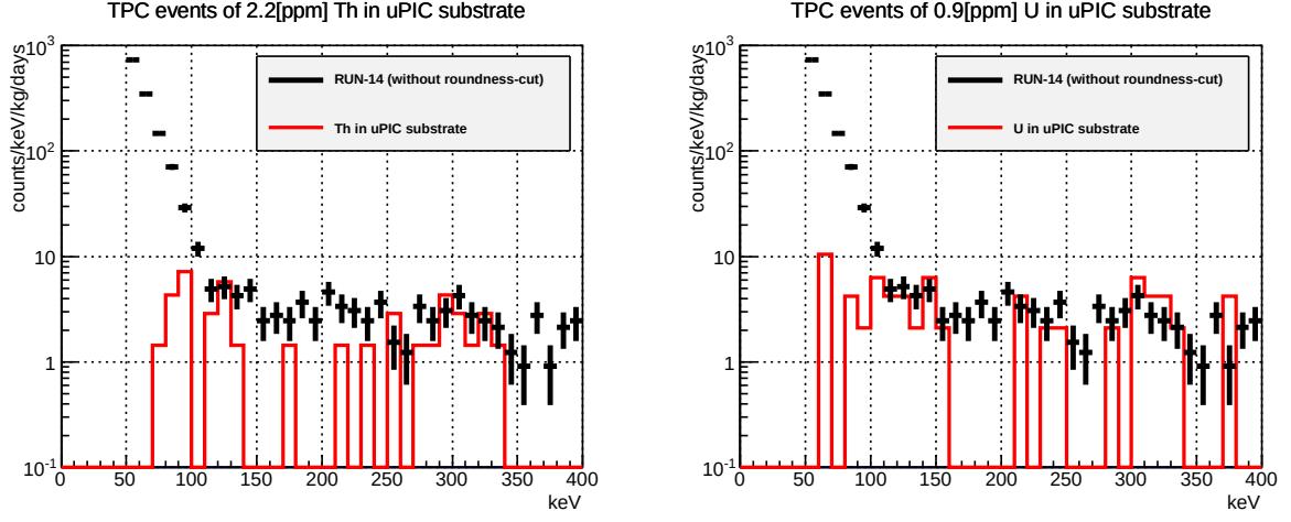
Figure 6.2.10: The estimated energy spectra of the events that \alpha particles from radioactive impurities included in the substrate of the \mu -PIC in the detection region (C in Figure 6.2.1). Left and right figure show the results by assuming 2.2 ppm of Th-chain and 0.9 ppm of U-chain, respectively. The evaluated concentration amounts of each isotope-chain discussed in Section 6.1.2 is used. We put the measured spectrum of RUN14 without the roundness-cut because the events from substrate is basically cut by the effect of z-fiducilization of roundness-cut.
