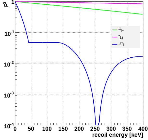
Figure 2.3.3: The SD form factors of some isotopes as a function of the recoil energy E_R . Green, pink and blue lines show target isotopes of ^{19}\text{F} , ^7\text{Li} and ^{127}\text{I} , respectively.
