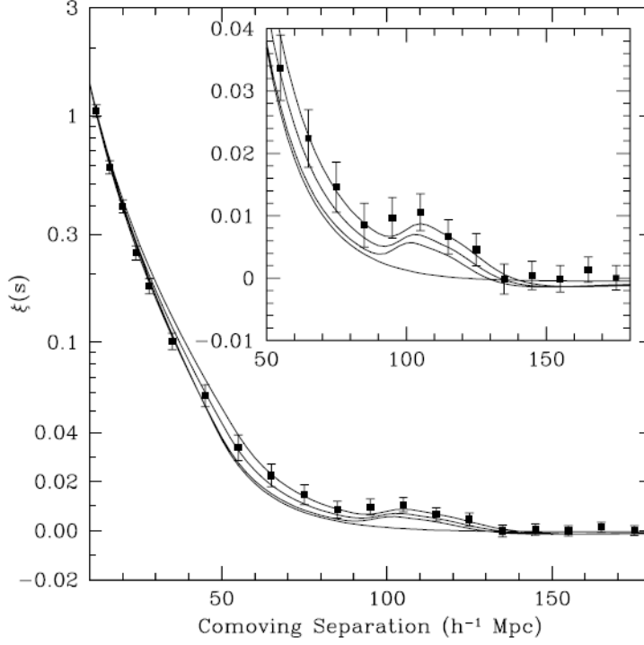
Figure 1.1.7: Measured two point correlation function of galaxies by SDSS[2]. Top, second and third lines show models assuming \Omega_m h^2 = 0.12 , 0.13 and 0.14 , respectively, all with \Omega_b h^2 = 0.024 and n = 0.98 . The bottom line shows a pure CDM model assuming \Omega_b h^2 = 0 and \Omega_m h^2 = 0.105 . Here, h is Hubble parameter normalized by 100 and n is number density of galaxy. Inset is the enlarged view.
