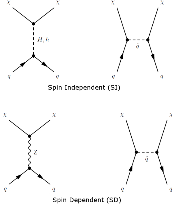
Figure 2.2.1: Feynman diagrams of neutralino-quark elastic scattering. Upper set is SI and lower set is SD, respectively.
