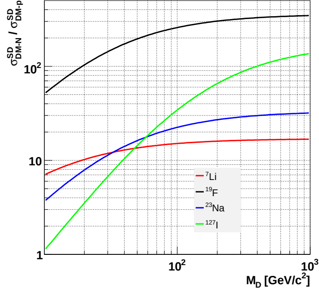
Figure 2.2.3: \sigma_{\chi-N}^{SD} / \sigma_{\chi-p}^{SD} as a function of neutralino mass. Red, black, blue and green line shows target isotope difference as ^7\text{Li} , ^{19}\text{F} , ^{23}\text{Na} and ^{127}\text{I} , respectively.
