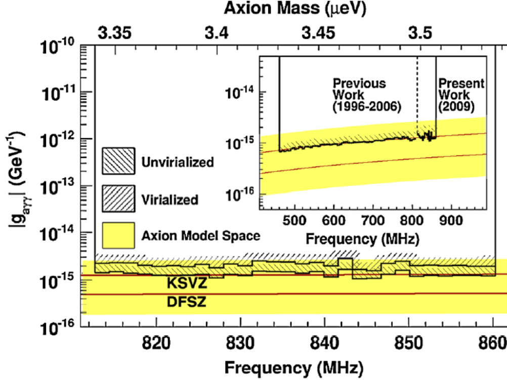
Figure 1.2.2: 90%C.L. limit of the axion-photon coupling for each mass of axion [16].
