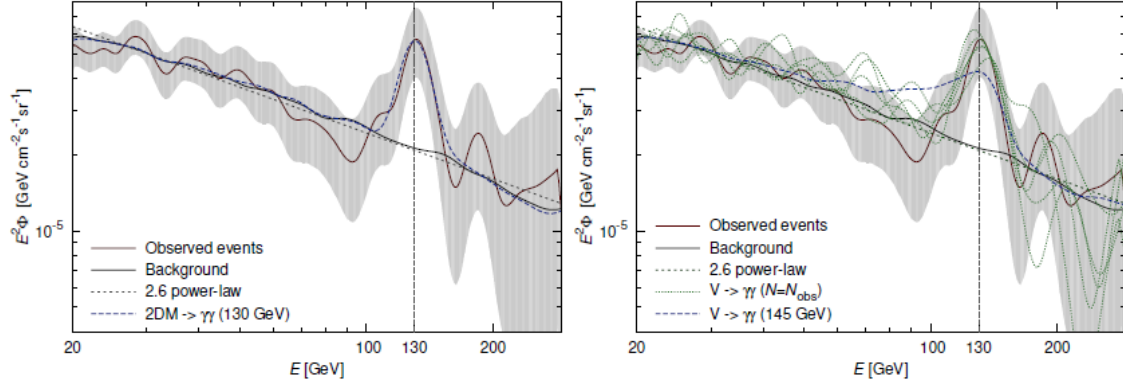
Figure 1.3.2: Energy spectrum of gamma-rays from the center of our galaxy measured by Fermi (red solid line). Gray region is 95%C.L. error band. Black dashed line is the best fit model assuming dark matter annihilation. Left and right figures are fitted with the 2\text{DM} \rightarrow 2\gamma channel model and 2\text{DM} \rightarrow 2V \rightarrow 4\gamma channel model, respectively, where V is light hypothetical final states. Best-fit mass are 130 GeV and 145 GeV for left and right figure, respectively.
