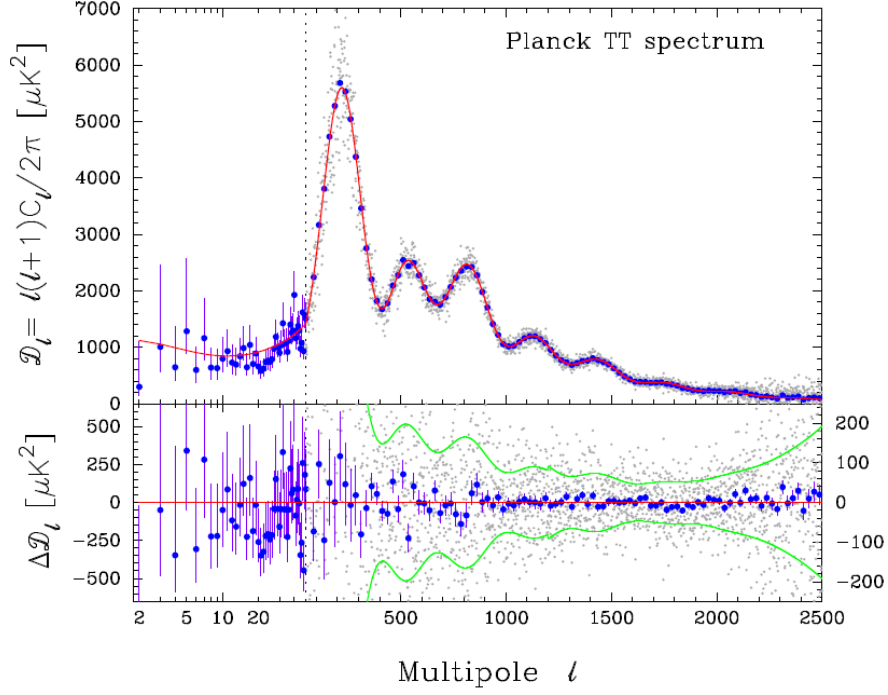
Figure 1.1.6: Angular power spectrum of CMB observed by Planck[1]. Blue points are measured data, red line is the best fit model. Bottom figure shows the residual from the best fit model.
