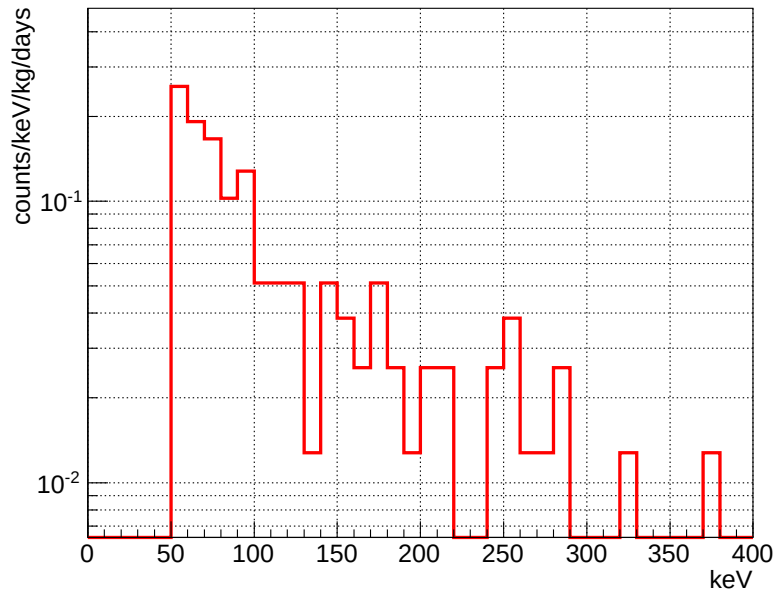
Figure 6.2.4: Estimated energy spectrum of nuclei recoiled by environmental neutrons. The estimated event rate at 50 – 60 keV is 0.3 counts/keV/kg/days.
