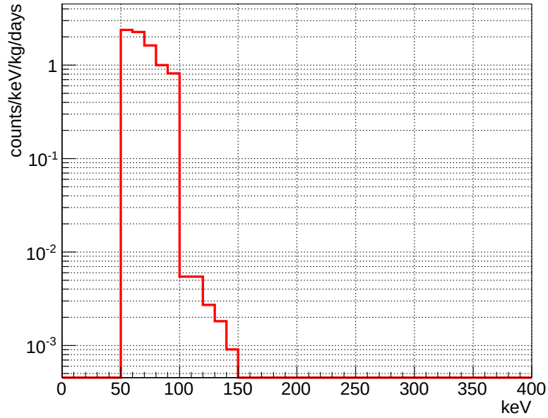
Figure 6.2.6: Estimated energy spectrum by environmental gamma-rays.
