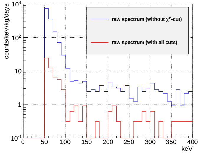
Figure 6.0.2: Obtained energy spectrum of RUN14 in the range of 50 – 400 keV.
