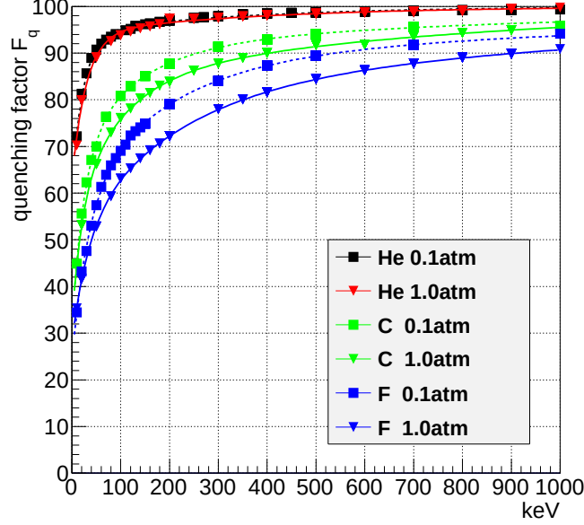
Figure 3.2.4: Quenching factor of various nucleus in \text{CF}_4 gas calculated by SRIM[67]. Each line shows different nuclei-pressure combination as shown in the legend.
