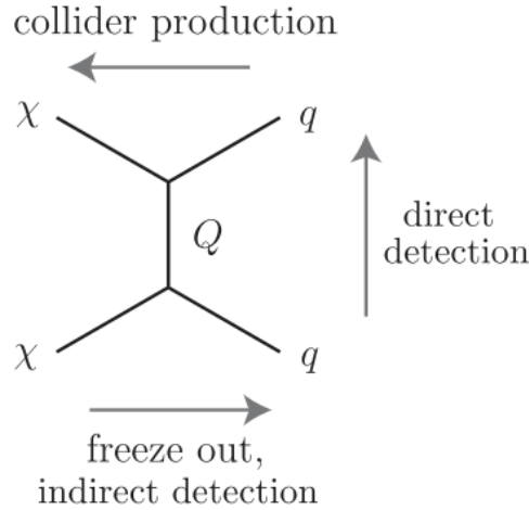
Figure 1.3.1: Feynman diagram contributing to, direct searches, indirect search, and collider production of dark matter[23]. Here, \chi , q and Q represent nenutralino, SM particle and a force-mediating boson, respectively.
