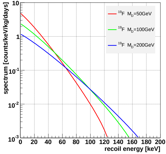
Figure 2.3.4: The expected energy spectra of SD interaction with ^{19}\text{F} target, where \sigma_{\chi^-p}^{\text{SD}} = 1 \text{ pb} is assumed. Red, green and blue lines show the cases for the neutralino mass of M_D = 50, 100 and 200 \text{ GeV}/c^2 , respectively.
