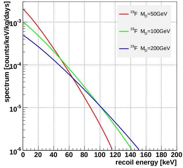
Figure 2.3.2: The expected energy spectra of SI interaction with ^{19}\text{F} target, where \sigma_{\chi-p}^{\text{SI}} = 10^{-6} \text{ pb} is assumed. Red, green and blue lines show the cases for the neutralino mass of M_D = 50 , 100 and 200 \text{GeV}/c^2 , respectively.
