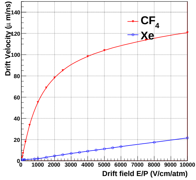
Figure 3.2.2: Drift velocities of electrons as a function of electric field calculated by MAGBOLTZ for \text{CF}_4 (red) and Xe(blue).
