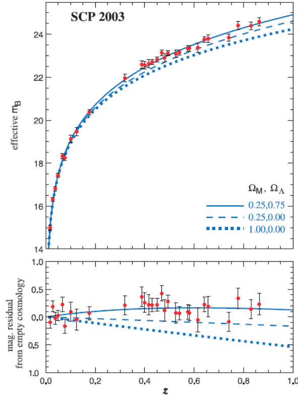
Figure 1.1.5: Observed IaSN luminosity (converted to magnitude m ) as a function of the distance (shown in units of redshift z )[3]. Red points are measured and blue lines are models. Bottom figure shows the residual from the model assuming \Omega_m = 0 , \Omega_\Lambda = 0 . The model with \Omega_m = 0.25 , \Omega_\Lambda = 0.75 was found to be consistent to the measurements.
