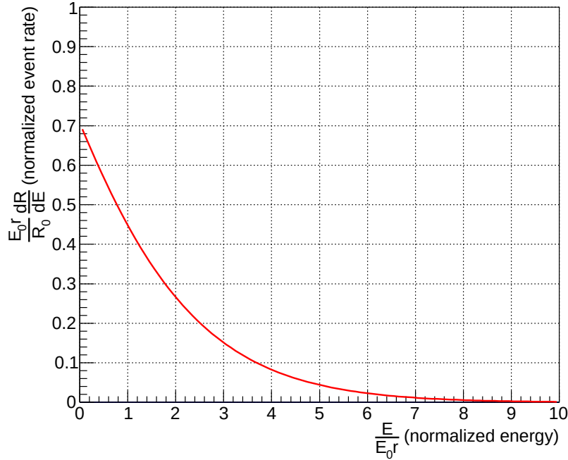
Figure 2.1.2: The normalized energy spectrum of nucleus caused by an elastic scattering of the WIMP. ^{19}\text{F} is assumed for the target.
