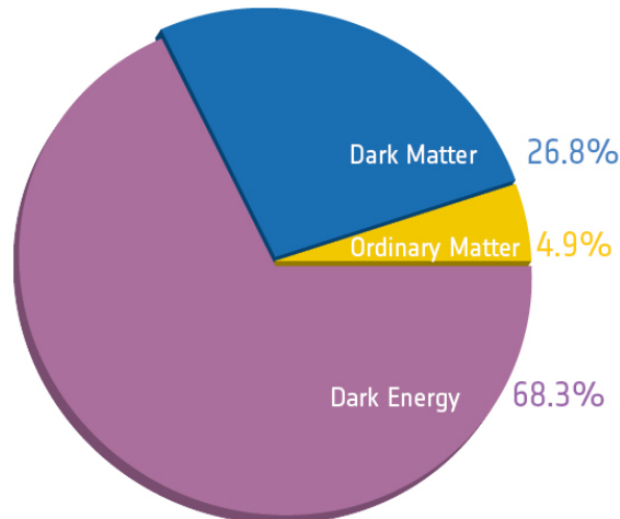
Figure 1.0.1: Composition of the energy of the universe. The universe was known to consist of 68.3 % dark energy, 26.8 % dark matter, and 4.9 % baryon (ordinary matter) from recent observations[1]
