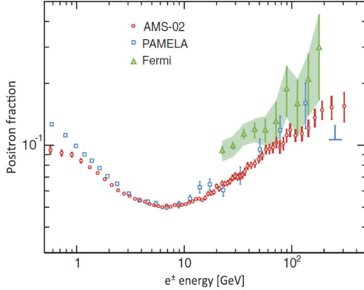
Figure 1.3.3: positron fraction N_{e^+}/(N_{e^-} + N_{e^+}) in the cosmic-ray measured by AMS-02, PAMELA and Fermi.
