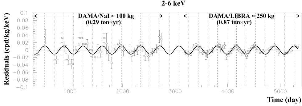
Figure 3.1.2: The observed annual modulation of the residual event rate of 2 – 6 keV energy range acquired over 13 annual cycles by DAMA and DAMA/LIBRA with a total exposure of 1.17 ton·year[37]. The horizontal axis shows the days from DAMA/NaI started. Solid line is the best fit sine curve.
