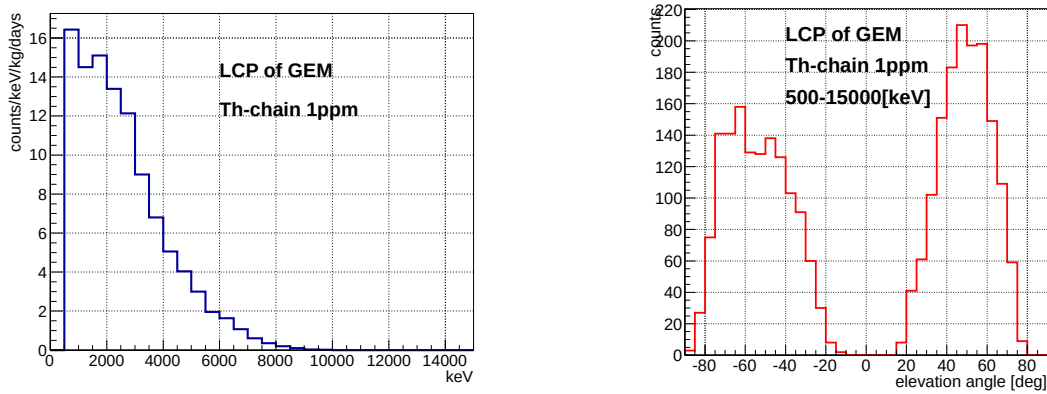
Figure 6.1.10: The simulation result of the energy spectrum (left) and elevation angle distribution in energy of 0.5 - 15 MeV (right) by assuming 1 ppm contamination of Th-chain in LCP of GEM (⑤,⑤').
