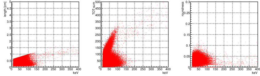
Figure 5.1.2: Energy dependence of the length (left), the TOT-sum (center), and the roundness (right). The events are cut by fiducial-cut and length-cut. These events correspond to the purple line in Figure 5.1.5.
