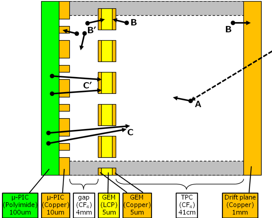
Figure 6.2.1: Candidates of low-energy background events (50 – 400 keV). From the discussion of high energy background as in Section 6.1, we only discuss about U/Th contamination in substrate of \mu -PIC as a background from material of the detector.
