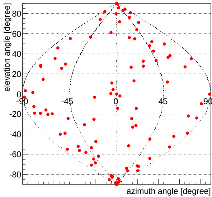
Figure 5.1.7: Obtained direction of the nuclear tracks of RUN-14 in the energy range of 50 – 400 keV
