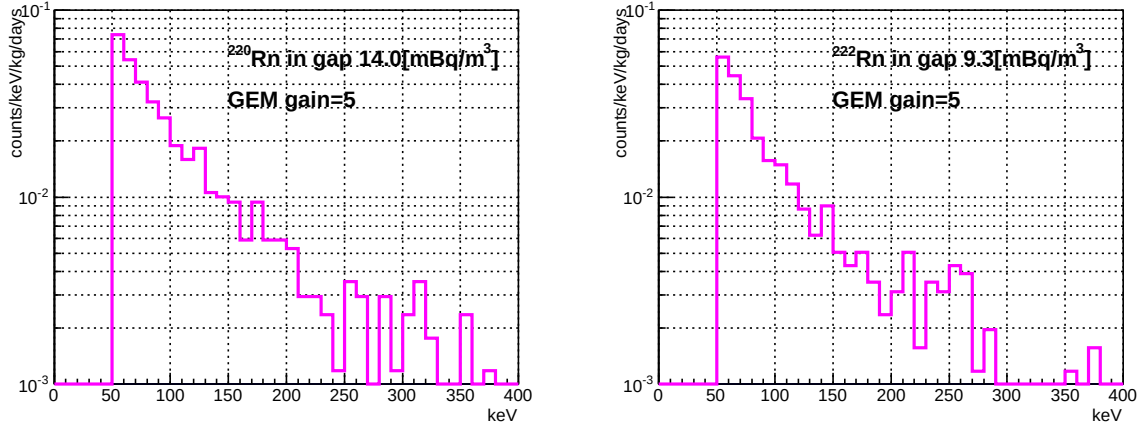
Figure 6.2.9: Estimated energy spectra of background from ^{220}\text{Rn} (left) and ^{222}\text{Rn} (right) in the gap volume. We assumed a typical gain of GEM.
