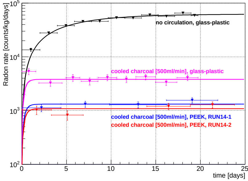
Figure 6.1.6: The measured time dependence of the peak component ( > 3000 keV).
