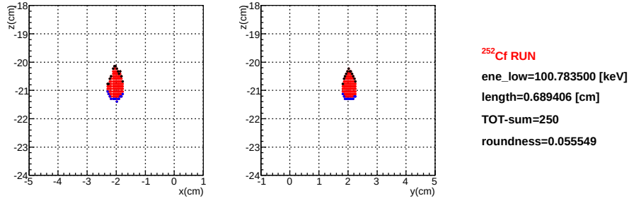
Figure 4.4.6: Track sample measured with ^{252}\text{Cf} . Left and right panel shows the x - z and y - z projection of the digitized track acquired by DAQ-mode5. Blue and black points shows the rise-time points and fall-time points. This event survives the length-cut, TOT-sum-cut and roundness-cut.
