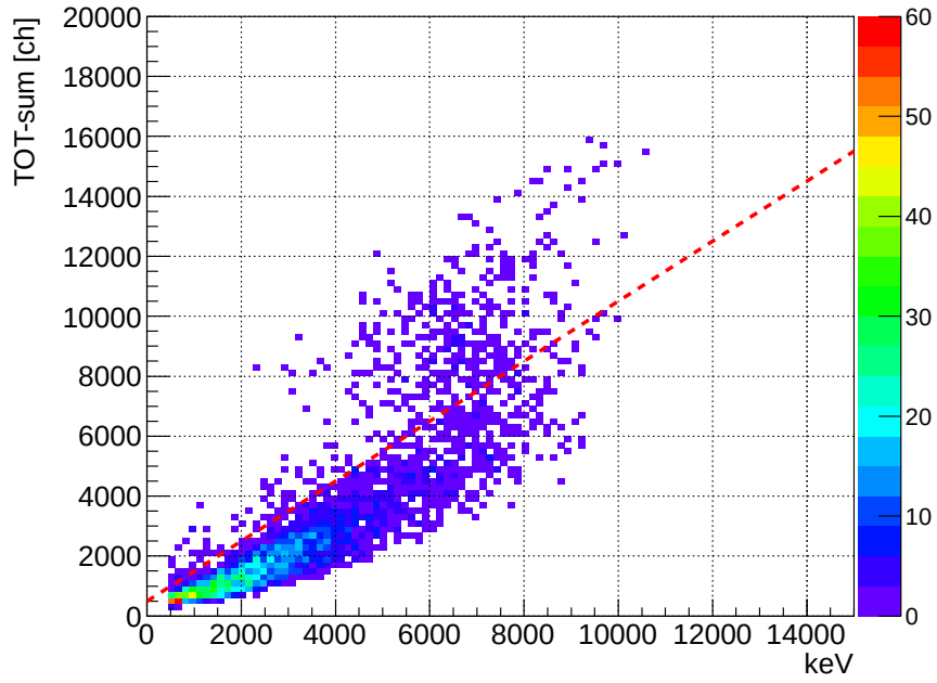
Figure 6.1.3: Measured TOT-sum as a function of energy.
