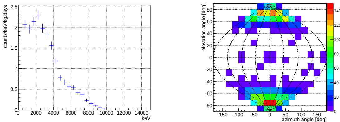
Figure 6.1.5: Obtained energy spectrum (left) and direction distribution (right) below the red dotted line in Figure 6.1.3.
