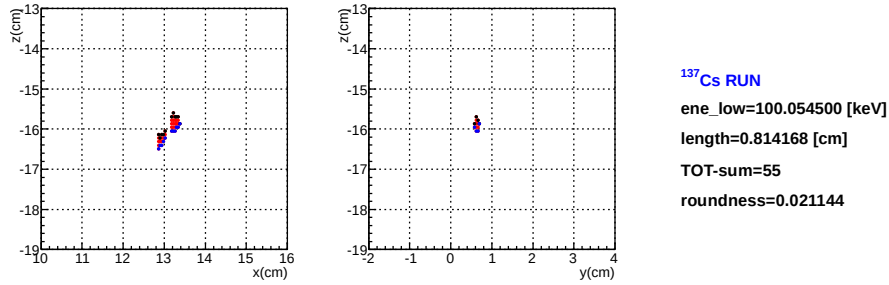
Figure 4.4.8: Track sample measured with ^{137}\text{Cs} , cut by TOT-sum-cut.
