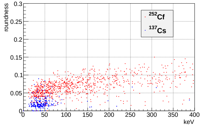
Figure 4.4.12: Energy dependence of the roundness after the length-cut and TOT-sum-cut. Red and blue points are same to above figure.
