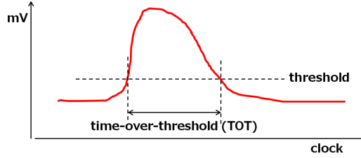
Figure 4.2.2: The schematic image of time-over-threshold (TOT). Red line shows the waveform of a strip.
