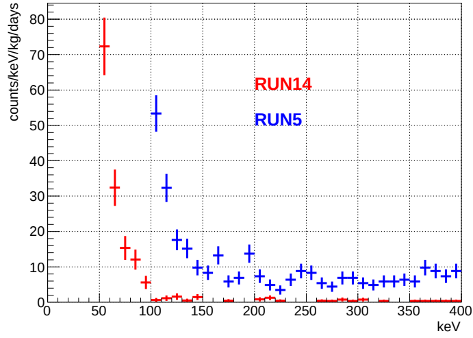
Figure 5.1.6: Obtained energy spectrum in Kamioka RUN-14 (red points). Blue points are the results of previous measurements RUN-5[58, 83]. Detection efficiency was taken into account.
