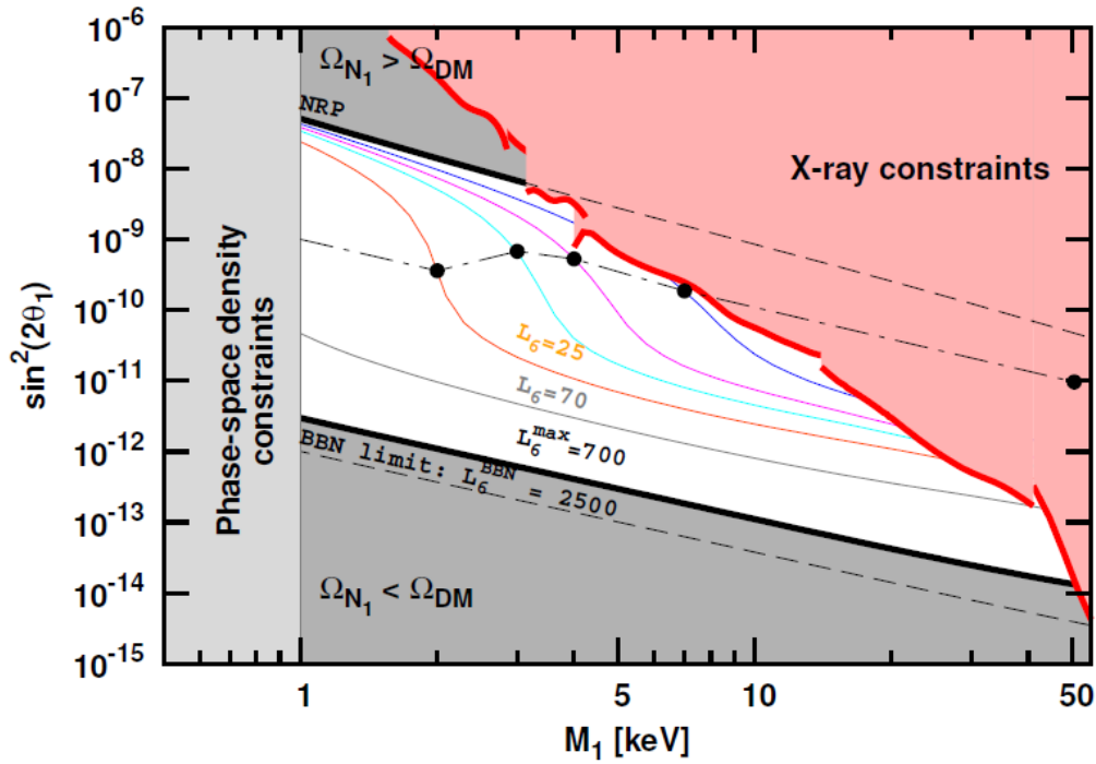
Figure 1.2.4: Obtained limits of the mixing angle \theta_1 as a function of sterile neutrino mass M_1 [18]. The red region is the constraint region by X-ray observations. The gray region is the constraint the sterile neutrino dark matter.
