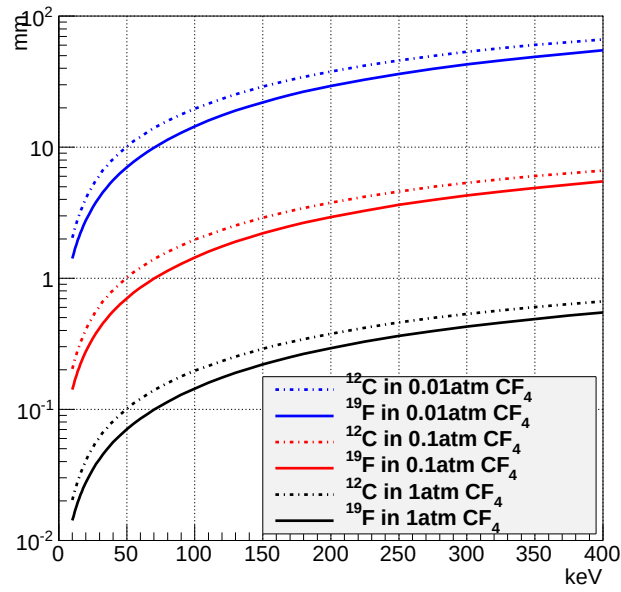
Figure 3.2.3: Track length of recoil ^{12}\text{C} (dotted line) and ^{19}\text{F} (solid line) in \text{CF}_4 gas calculated by SRIM with each pressure (blue:0.01atm, red:0.1atm, black:1.0atm).
