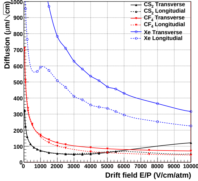
Figure 3.2.1: Gas diffusions of electrons or negative ions as a function of the electric field at a temperature of 300K calculated by MAGBOLTZ. Dotted and Solid line are longitudinal and transverse diffusion, respectively. Color shows the molecular; red, blue and black correspond to \text{CF}_4 , Xe and \text{CS}_2 , respectively.
