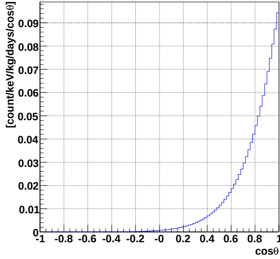
Figure 2.4.5: The expected \cos\theta distribution (100 – 120 keV), where the target is ^{19}\text{F} for the SD interaction, M_{\text{D}} = 100 \text{ GeV} , \sigma_{\chi\text{-p}}^{\text{SD}} = 1 \text{ pb} , \theta is the angle formed by the WIMP-wind direction and the recoil nuclei direction.
