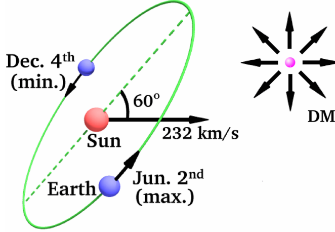
Figure 2.1.1: The schematic view of the motion of the Sun and the Earth in our galaxy.
