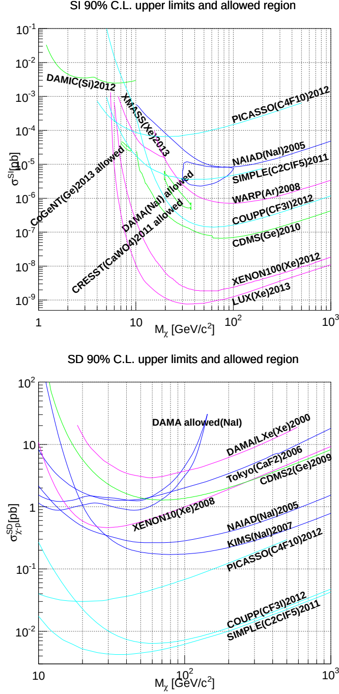
Figure 3.1.1: Results of direct dark matter search experiments. Upper and lower figures are searches of SI and SD \chi -p interacting WIMPs, respectively. See Table 3.0.1 for references. Region enclosed by line is allowed region (DAMA). Other upper regions of lines are excluded regions. Color indicates the type of detector; blue for solid scintillator, purple for liquid noble gas detector, green for semiconductor detector, and sky blue for bubble chamber.
