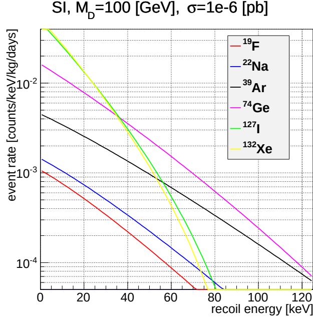
Figure 2.4.1: The expected energy spectrum dR/dE_R of various targets for the SI-interacting neutralino with a mass of M_D = 100 \text{ GeV}/c^2 and \sigma_{\chi-p}^{\text{SI}} = 1 \times 10^{-6} \text{ pb} .
