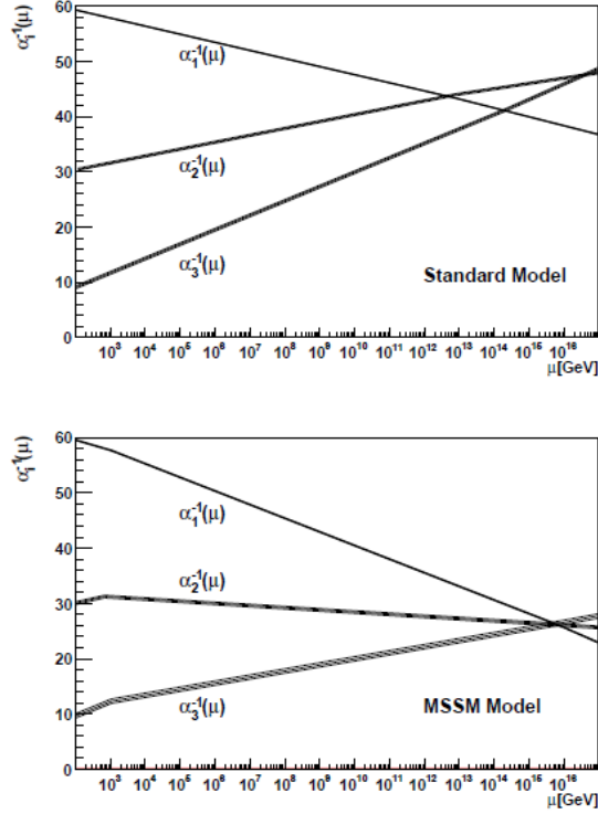
Figure 1.2.1: The relation of the coupling constants and energy in the standard model (SM) (top) and in the minimum supersymmetric standard model (SMMS) (bottom). \alpha_1, \alpha_2 and \alpha_3 are the U(1) , U(2) and U(3) couplings, respectively.
