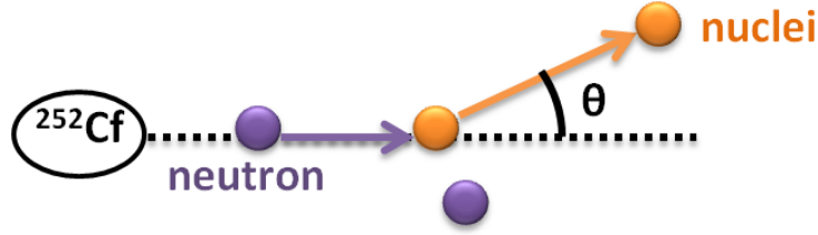
Figure 4.4.16: The schematic view of nuclear recoil. \theta is the recoil angle.
