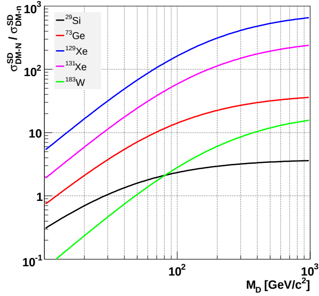
Figure 2.2.4: \sigma_{\chi-N}^{SD} / \sigma_{\chi-n}^{SD} as a function of neutralino mass. Black, red, blue, pink, green line shows target isotope difference as ^{29}\text{Si} , ^{73}\text{Ge} , ^{129}\text{Xe} , ^{131}\text{Xe} and ^{183}\text{W} , respectively.
