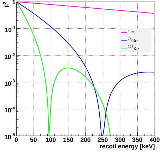
Figure 2.3.1: The SI form factors of some isotopes as a function of the recoil energy E_R . Pink, blue and green lines show target isotopes of ^{19}\text{F} , ^{74}\text{Ge} and ^{132}\text{Xe} , respectively.
