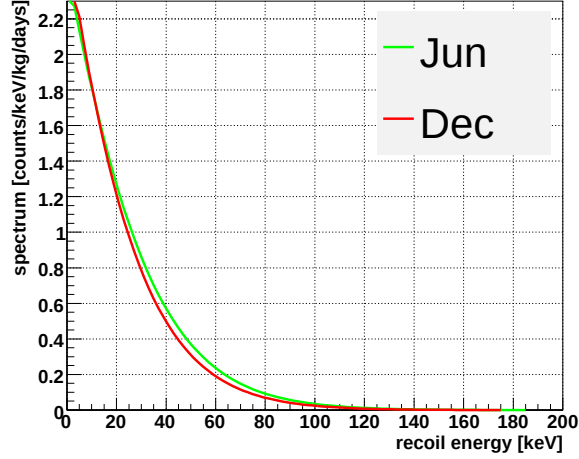
Figure 2.4.3: The expected modulation of energy spectrum between June and December, where the target is ^{19}\text{F} for the SD interaction, M_{\text{D}} = 100 \text{ GeV} , \sigma_{\chi\text{-p}}^{\text{SD}} = 1 \text{ pb} .
