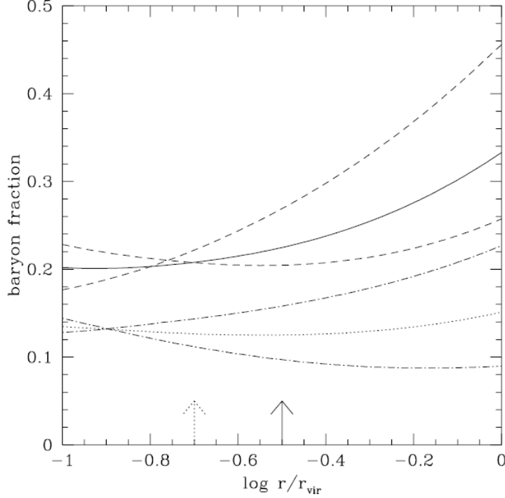
Figure 1.1.2: The baryon fraction of galaxy clusters Abell1060 and AWM7 observed by ASCA[6]. Horizontal axis is distance from the center of galaxy clusters normalized by r_{\text{vir}} . r_{\text{vir}} is the 2 \pm 0.5 Mpc and 2 \pm 0.4 Mpc for Abell1060 and AWM7 were taken, respectively. Solid line and dotted line show the best fit model corresponding to Abell1060 and AWM7, respectively. Dashed line and dot-dash line show the model in case most compact and most expanded, respectively.
