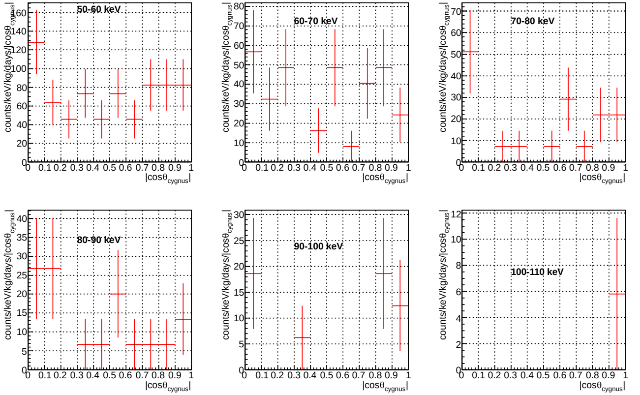
Figure 5.1.9: Obtained |\cos \theta_{\text{cygnus}}| distribution of RUN-14 of the lowest 6 bins.
