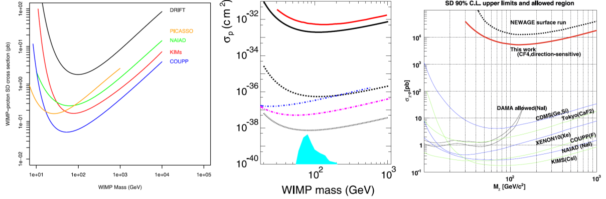
Figure 3.2.5: Results of direction-sensitive direct dark matter search experiments. In left figure, black solid line shows the result of DRIFT(2012)(without direction-sensitive analysis)[56]. In the central figure, black solid line shows the result of DM-TPC(2011)[57]. In right figure, red solid line shows the result of NEWAGE(2010)[58]. For more information, see references.
