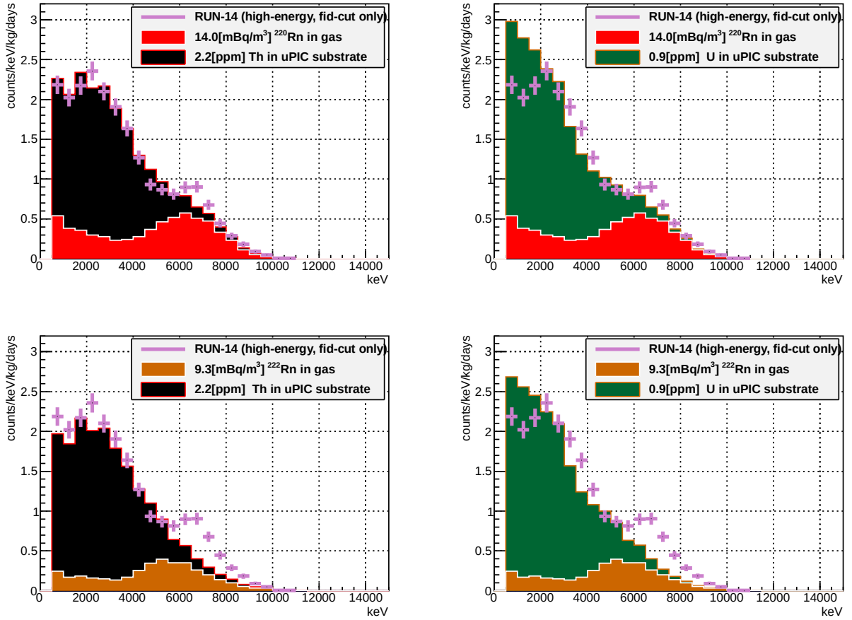
Figure 6.1.15: Energy spectrum of the high energy background. Each figure differs in the type of radon and U/Th in substrate.
