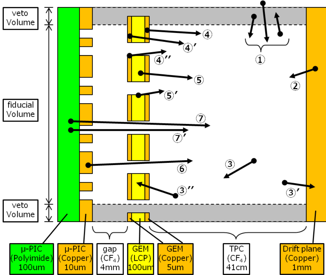
Figure 6.1.1: Candidates of high-energy background events (500 – 15000 keV).
