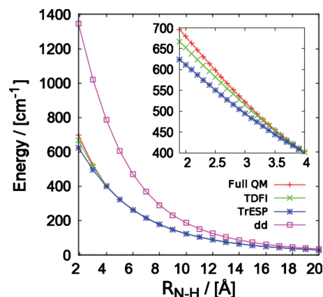
FIG. 4. Electronic coupling energies between two SB5 chromophores as a function of intermolecular N-H distance. (+) Full quantum-mechanical, (x) TDFI, (*) TrESP, and (□) dd results. All calculations are performed with TD-rCAM-B3LYP/6-31G*.
