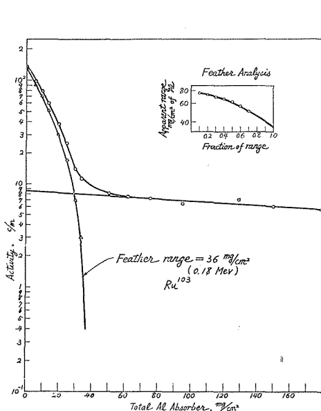
Fig. 8 : \beta -ray Absorption Curve, Ru 103 : Applied potential ; 1350 V, Geometry ; sample 3rd shelf, absorber 2nd shelf.
