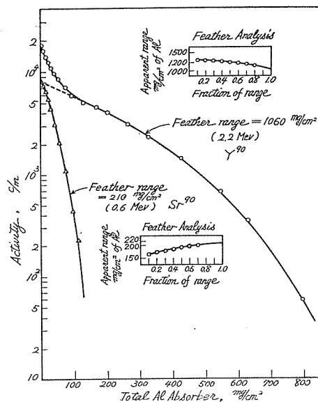
Fig. 7 : \beta -ray Absorption Curve
