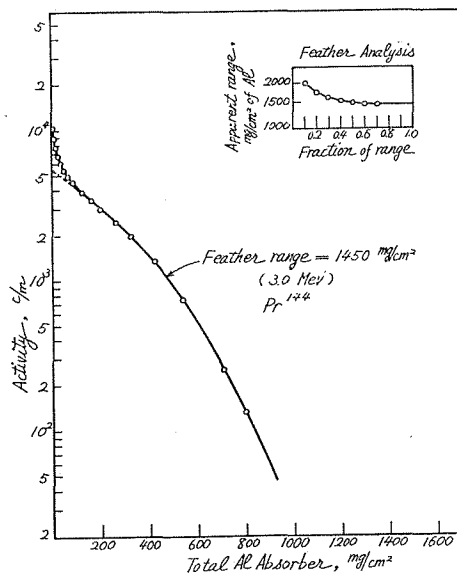
Fig. 4 : \beta -ray Absorption Curve, Ce-Pr (original sample) : Applied potential ; 1350 V, Geometry ; sample 3rd shelf, absorber 2nd shelf.
