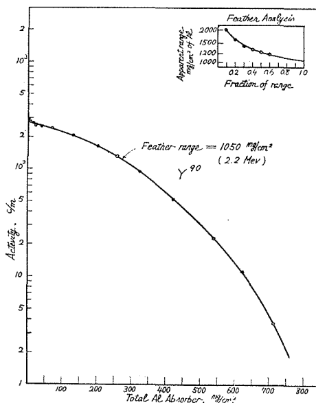
Fig. 20 : \beta -ray Absorption Curve, \text{Y}^{90} ( R_f=0.20 ): Applied potential; 1350 V, Geometry; sample 3rd shelf, absorber 2nd shelf.
