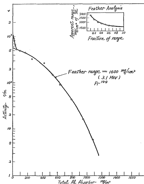
Fig. 9 : \beta -ray absorption Curve, Ce 144 -Pr 144 : Applied potential ; 1350 V, Geometry ; sample 3rd shelf, absorber 2nd shelf.
