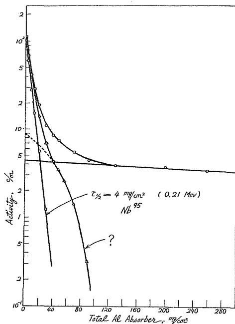
Fig. 22 : \beta -ray Absorption Curve, \text{Nb}^{95} : Applied potential ; 1450 V, Geometry ; sample 1st shelf, absorber 1st shelf.
