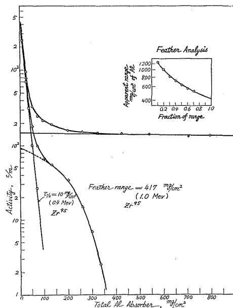
Fig. 2 : \beta -ray Absorption Curve, Zr-Nb (original sample) : Applied potential ; 1350 V, Geometry ; sample 3rd shelf, absorber 2nd shelf.
