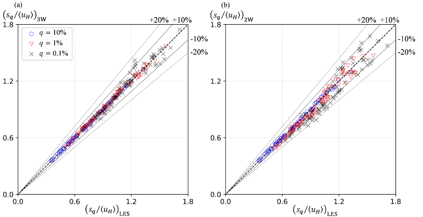
Fig. 6. Comparison of the LOSWSs with q = 10\% , 1\% and 0.1\% . The x-axis denotes the wind speed calculated from the LES time-series data (s_q / \langle u_H \rangle)_{LES} and y-axis denotes the wind speed estimated from the (a) 3W method (s_q / \langle u_H \rangle)_{3W} or (b) 2W method (s_q / \langle u_H \rangle)_{2W} . \langle u_H \rangle is the mean streamwise velocity at the building height of the inflow boundary.
