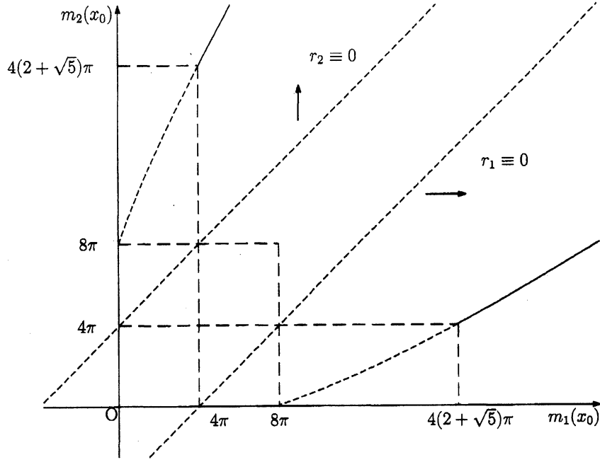
Figure 3: The parabola
