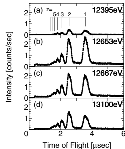
FIG. 2. The PEPICO spectrum versus time of flight for the Se cluster beam at the preedge region (a), at the resonance absorption region (b), at the beginning (c), and end (d) of the EXAFS region.
