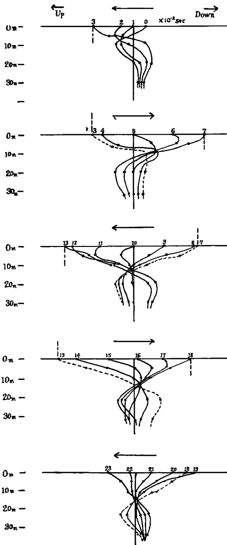
Fig. 8 The amplitude distribution of M_2 -waves with depth for every 1/100 sec
