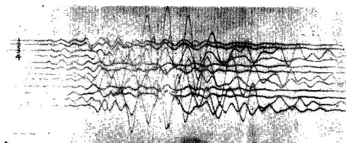
Fig. 12 Seismograms obtained by the shallow shot Shot-receiver distance ; 60 m Shot-hole depth ; 1 m
