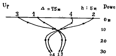
Fig. 7 The amplitude distribution of M_2 -waves with depth Shot-receiver distance ; 75 m Shot-hole depth ; 5 m
