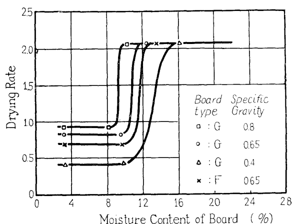
Fig. 13. Moisture content-drying rate diagram. (initial moist. cont. 21~22%, board thickness 20 mm)
