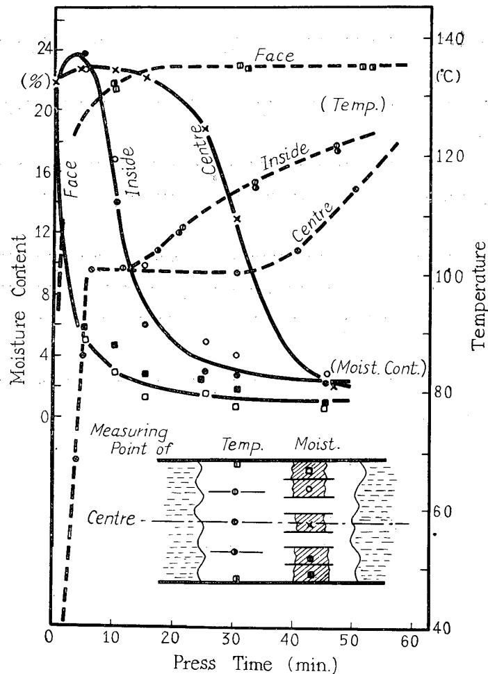
Fig. 15. Moisture and temperature behavior in board. (G-type, spec. grav. 0.65, initial moisture content 22%, board thickness 20 mm)
