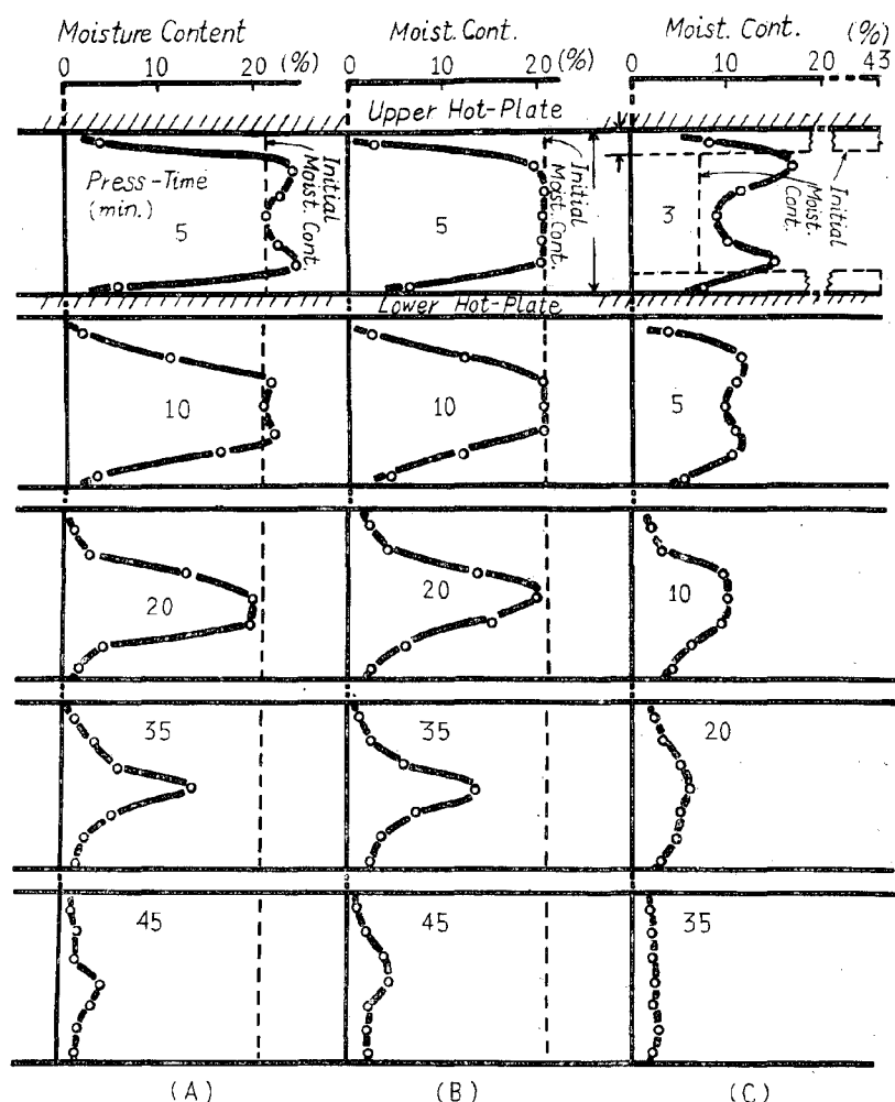
Fig. 14. Moisture distribution in board (20 mm thick)
