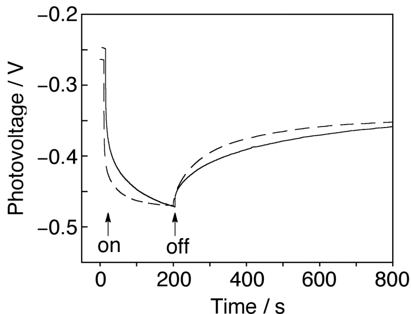
Figure 9. Photovoltage response of the FTO/SnO 2 /(RGO+ZnONP+ZnP) m (solid line) and FTO/SnO 2 /(ZnONP+ZnP) m (dashed line) electrodes under white light illumination (input power: 37.4 mW cm -2 , \lambda > 380 nm) in a deaerated acetonitrile solution containing 0.1 M TBAP.
