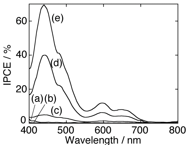
Figure 8. Photocurrent action spectra of the (a) FTO/SnO 2 /(ZnP) m , (b) FTO/SnO 2 /(RGO+ZnONP) m , (c) FTO/SnO 2 /(ZnP) m , (d) FTO/SnO 2 /(ZnONP+ZnP) m , (e) FTO/SnO 2 /(RGO+ZnONP+ZnP) m electrodes. Applied potential: 0.05 V vs SCE; 0.5 M LiI and 0.01 M I 2 in acetonitrile as an electrolyte. IPCE values were calculated by normalizing the photocurrent densities for incident light energy and intensity and by use of the expression: IPCE (\%) = 100 \times 1240 \times i / (W_{in} \times \lambda) = (\text{light harvesting efficiency}) \times (\text{electron injection efficiency}) \times (\text{electron collection efficiency}) , where i is the photocurrent density (A cm -2 ), W_{in} is the incident light intensity (W cm -2 ), and \lambda is the excitation wavelength (nm).
