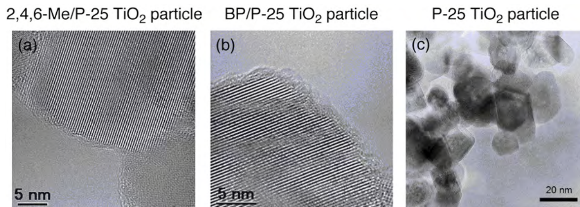
Figure 6. TEM images of TiO 2 nanoparticles sensitized with (a) 2,4,6-Me and (b) BP for 1 h in t -BuOH/ACN that yielded complete monolayers of the dyes. The average thickness of the Zn-porphyrin layers were determined as 1.0 \pm 0.2 nm for BP and 2,4,6-Me . (c) TEM image of TiO 2 nanoparticles with out porphyrin is also shown for comparison.
