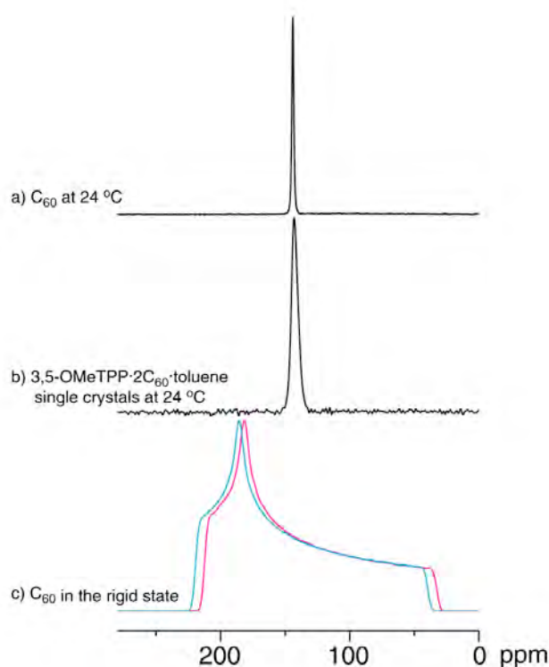
Figure 4. DP/CSA/noDD 13 C NMR spectra of (a) pristine C 60 , (b) 3,5-OMeTPP·2C 60 ·toluene single-crystals at 24°C. Calculated 13 C CSA spectra of C 60 in the rigid state are also shown in (c) for reference. For (c), the experimentally-obtained CSA tensor principal values of ( \sigma_{11} , \sigma_{22} , \sigma_{33} ) = (220, 186, 40) ppm (Ref. 21) and (213, 182, 33) ppm (Refs. 22, 23) are used, as shown in blue and red lines, respectively.
