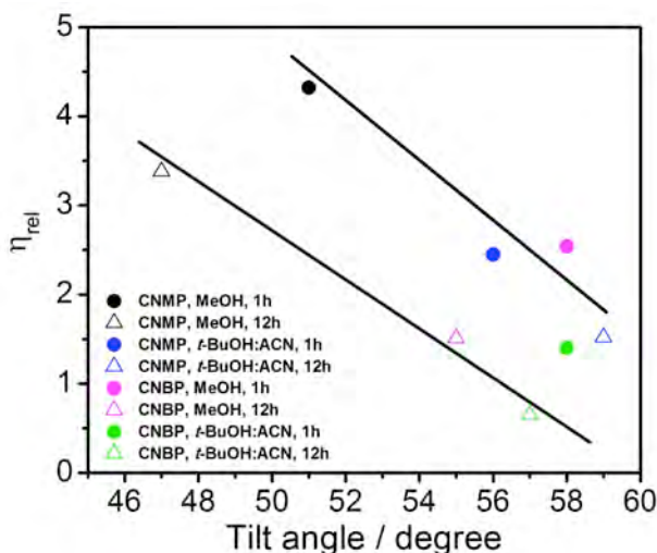
Figure 14. Solar cell efficiency normalized for surface coverage ( \eta_{rel} ) as a function of tilt angle. Closed circle and triangle symbols correspond to the immersion time of 1 h and 12 h, respectively.
