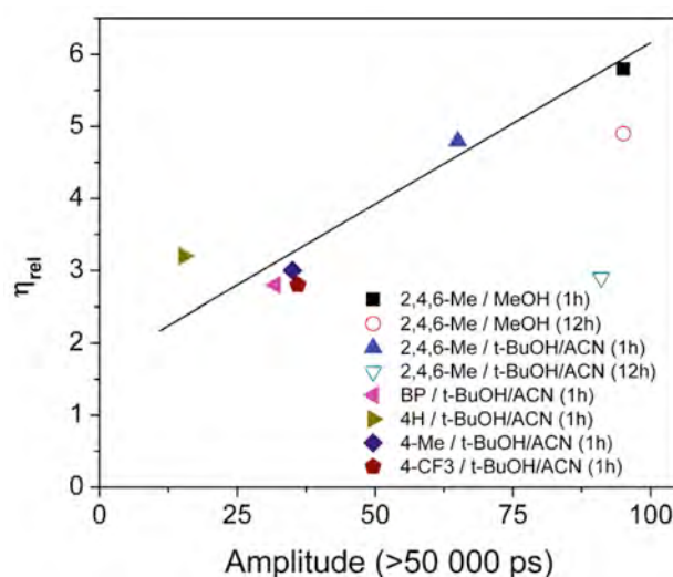
Figure 9. Solar cell power conversion normalized for surface coverage ( \eta_{\text{rel}} ) as a function of long-lived recombination signal ( A_{>50\text{ns}} ). Closed symbols represent measurements of TiO 2 films sensitized for 1 h. Particular dye and solvent are in figure legend.
