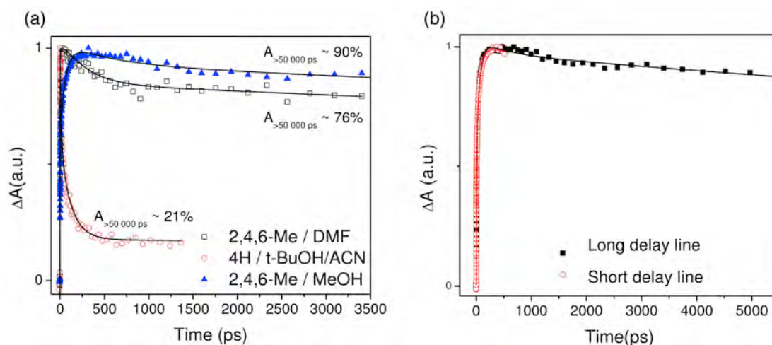
Figure 3. (a) Long delay line kinetics (at 660 nm) of 2,4,6-Me on TiO 2 sensitized in MeOH (closed blue triangle) and DMF (open, black square) and of 4-H on TiO 2 sensitized in t -BuOH/ACN (open, red circle) for 12 hours. All kinetics are normalized to maxima and solid black lines represents fits of the kinetics.
