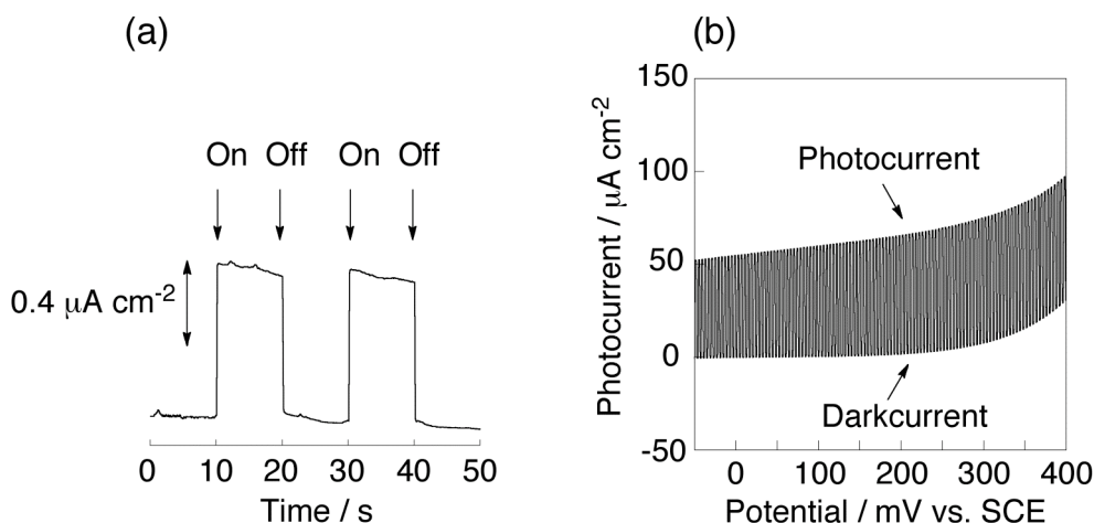
Figure 7. (a) The photoelectrochemical response of the \text{FTO}/\text{ZnO-r}/(\text{C}_{60}\text{-acid})_1/(\text{ZnP}+\text{C}_{60}\text{-acid})_m device. Potential: +0.55 V vs. NHE; excitation wavelength: \lambda_{\text{ex}} = 400 \text{ nm} ( 1.35 \mu\text{W cm}^{-2} ). (b) Current vs. applied potential curve of the \text{FTO}/\text{ZnO-r}/(\text{C}_{60}\text{-acid})_1/(\text{ZnP}+\text{C}_{60}\text{-acid})_m device; excitation wavelength: \lambda_{\text{ex}} > 380 \text{ nm} ( 37.4 \text{ mW cm}^{-2} ). [\text{ZnP}] : [\text{C}_{60}\text{-acid}] = 1 : 6 ( [\text{ZnP}] = 0.67 \text{ mM} , [\text{C}_{60}\text{-acid}] = 4.00 \text{ mM} ); electrolyte: 0.5 M LiI and 0.01 M \text{I}_2 .
