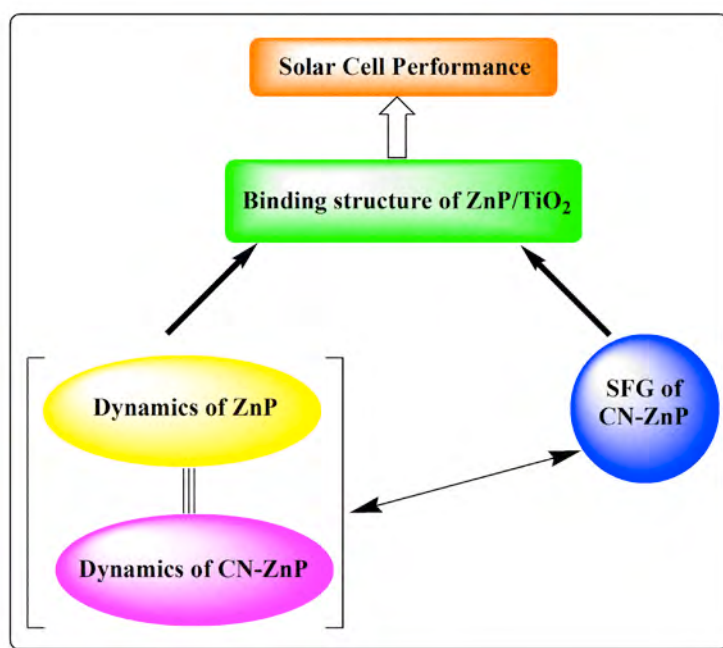
Scheme 1. Illustration of the experimental approach used in this work – Sum Frequency Generation (SFG) measures the binding geometry on the \text{TiO}_2 surface of CN-labeled Zn-porphyrin molecules, and comparison of electron transfer dynamics of CN-labeled and non-labeled molecules reveals the suitability of the CN-ZnPs as structural probes. Finally, binding geometry and electron transfer dynamics are correlated to solar cell performance.
