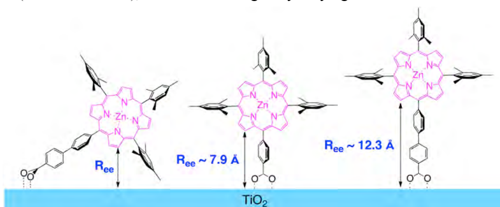
Figure 5. Binding model for Zn-porphyrins to TiO 2 . The edge-to-edge distance ( R_{ee} ) is decreased upon tilting of the dye molecule.
