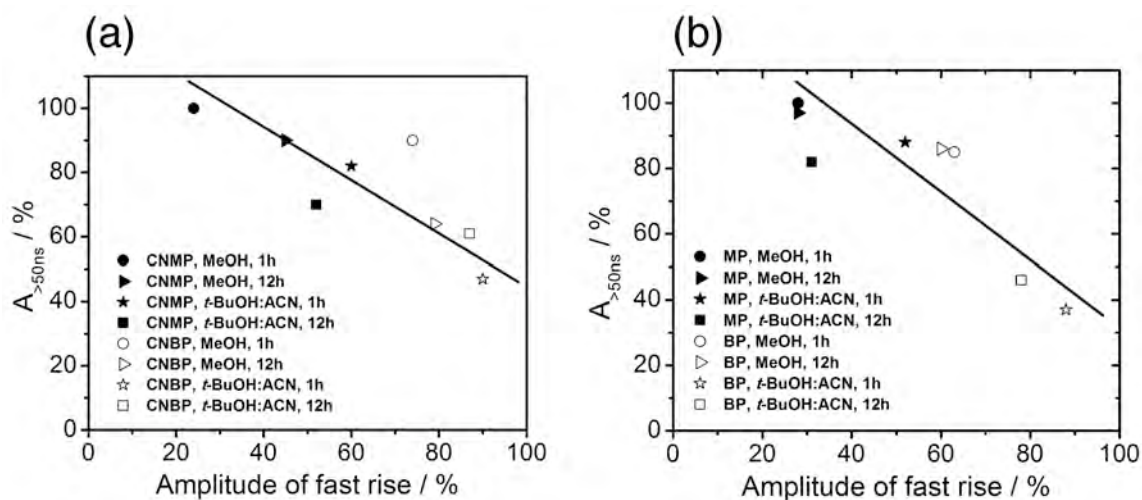
Figure 12. (a) Instantaneous rise as a function of long-lived recombination signal ( A_{>50\text{ ns}} ) of CN-labeled molecules. Closed and opened symbols correspond to monophenyl and biphenyl spacer molecules, respectively. (b) A_{>50\text{ ns}} vs. amplitude of instantaneous rise of transient absorption kinetics of non-labeled molecules. Closed and opened symbols correspond to monophenyl and biphenyl spacer molecules, respectively.
