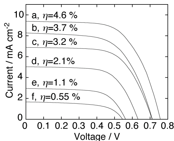
Figure 6. Current-voltage characteristics of 2,4,6-Me -sensitized \text{TiO}_2 cells under AM 1.5 conditions. Conditions for the immersion solvent and time: (a) MeOH, 1 h, (b) MeOH, 12 h, (c) EtOH, 12 h, (d) t -BuOH-MeCN mixture (1:1, v/v), 12 h, (e) \text{CH}_2\text{Cl}_2 , 12 h, and (f) DMF, 12 h. Conditions for the photovoltaic measurements: electrolyte 0.1 M LiI, 0.05 M \text{I}_2 , 0.6 M 2,3-dimethyl-1-propyl imidazolium iodide, and 0.5 M 4- t -butylpyridine in acetonitrile; input power: AM 1.5 under simulated solar light ( 100 \text{ mW cm}^{-2} ). For the 2,4,6-Me -sensitized cell optimized using P-25, J_{\text{sc}} of 9.4 \text{ mA cm}^{-2} , V_{\text{oc}} of 0.76 V, and ff of 0.64 yield \eta of 4.6 % (curve a).
