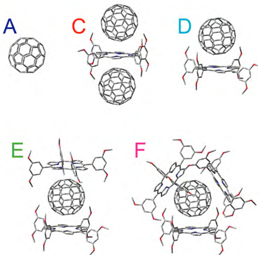
Figure 5. Graphic representation of supramolecular clusters. (A) Free C 60 and 3,5-OMeTPP/C 60 supramolecular complexes with the 3,5-OMeTPP/C 60 molar ratio of (C) 1 : 2, (D) 1 : 1, (E) 2 : 1, and (F) 3 : 1. Hydrogen atoms are omitted for clarity. These possible 3,5-OMeTPP/C 60 supramolecular clusters are used for the isotropic chemical shift calculations.
